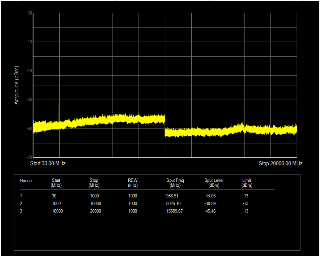
n2 SCS=15kHz DFT_BPSK BW=10MHz Channel=381000 RB=1@0
