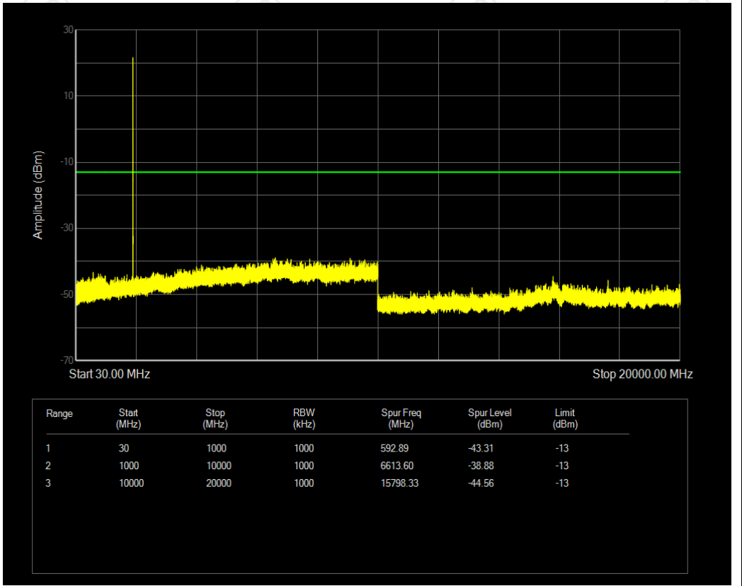
n2 SCS=15kHz DFT_BPSK BW=10MHz Channel=371000 RB=1@0
