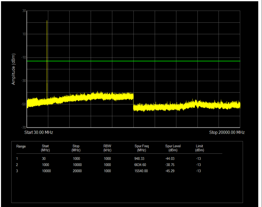
n2 SCS=15kHz DFT_BPSK BW=5MHz Channel=381500 RB=1@0
