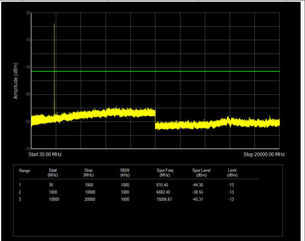
n2 SCS=15kHz DFT_BPSK BW=5MHz Channel=376000 RB=1@0
