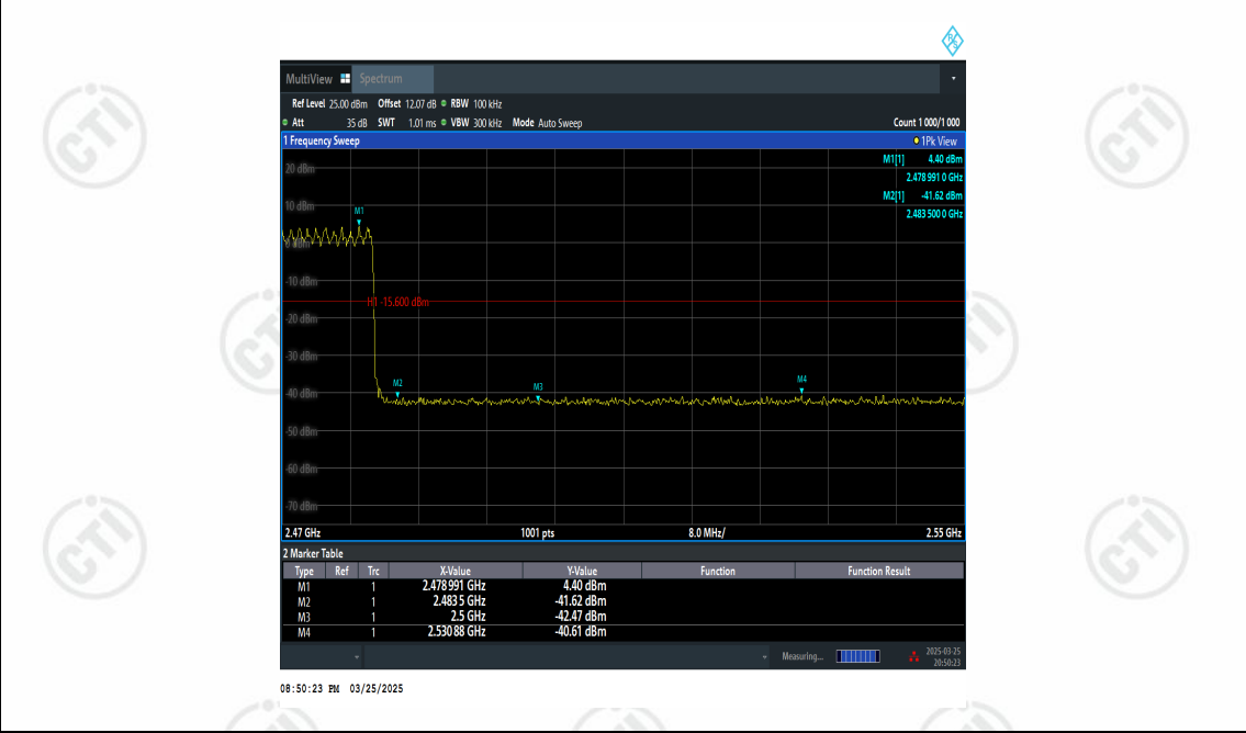
2DH5-Ant1-Hop_2480-PASS
