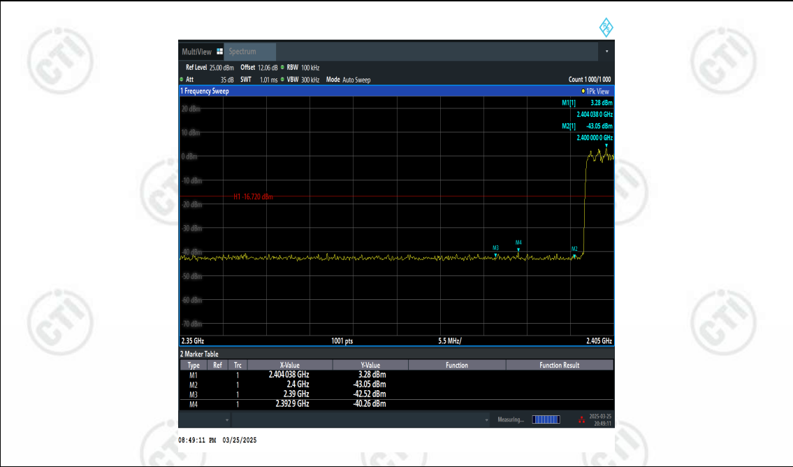
2DH5-Ant1-Hop_2402-PASS
