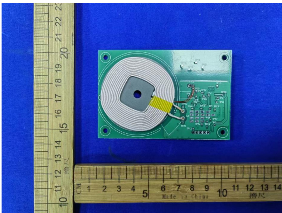
Figure 11. WPT module
