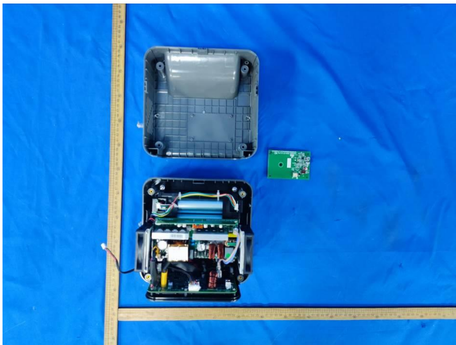
Figure 2. Internal view
