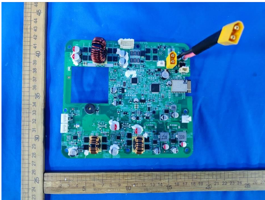
Figure 7. PCB of Main board & BMS board
