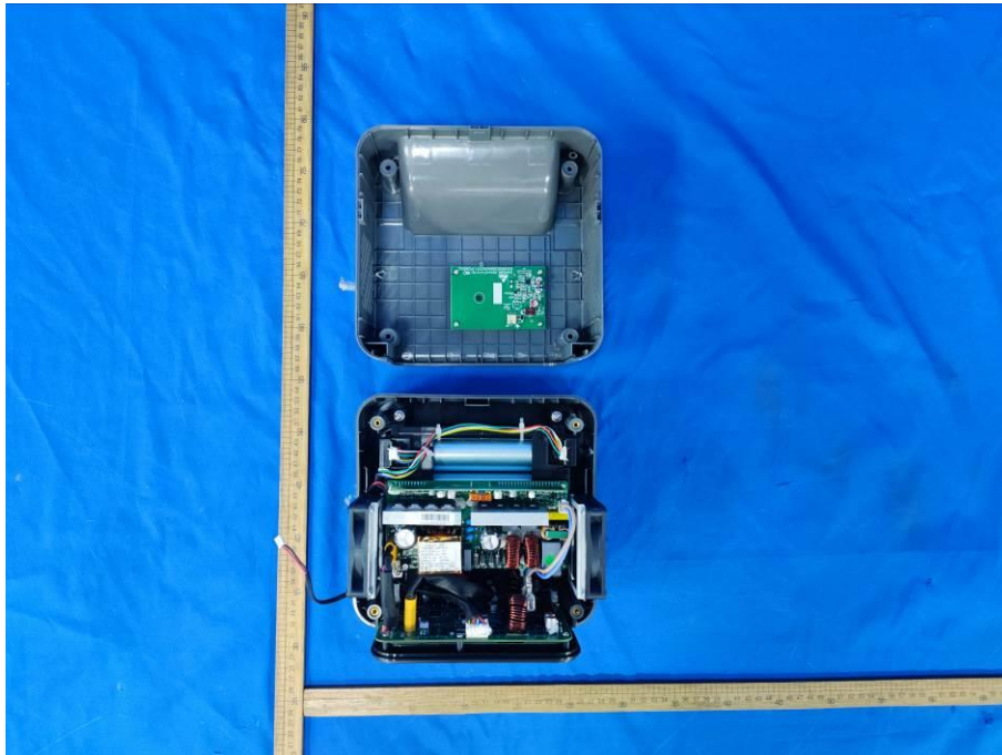
Figure 1. Internal view
