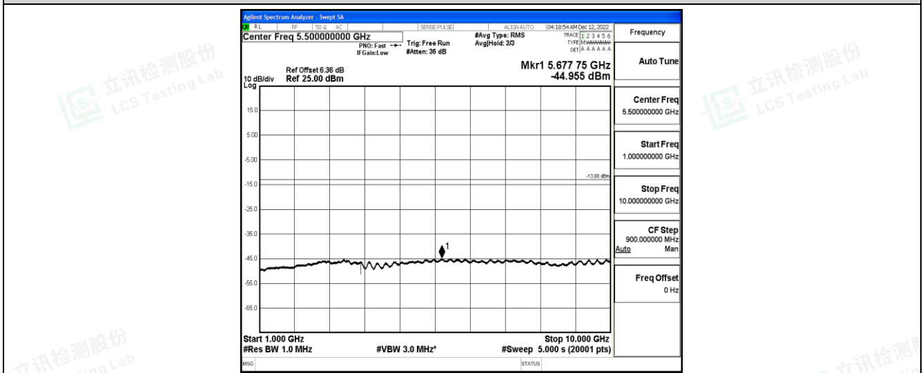
Band26-10MHz-16QAM-26740-1RB#0-Range4:1000~10000MHz
