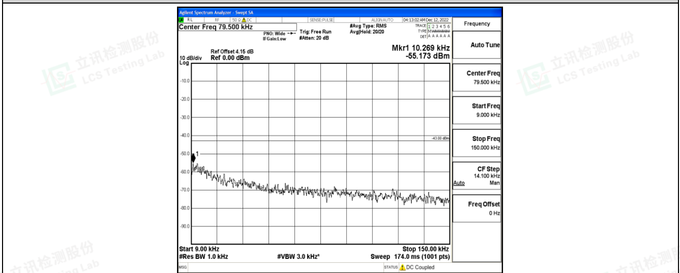
Band26-5MHz-16QAM-26740-1RB#0-Range1:0.009~0.15MHz
