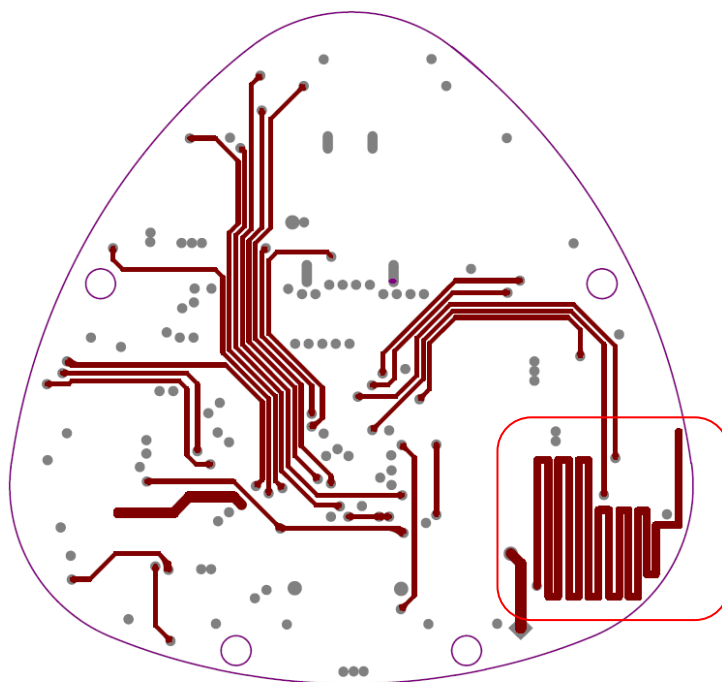
RF Antenna location (PCB Layout 2)
