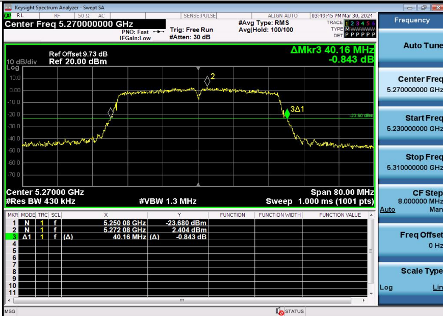
11AC40SISO-Ant2-5270
