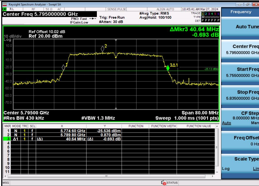
11AC40SISO-Ant2-5795
