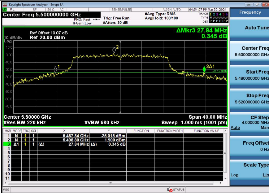
11AX20SISO-Ant2-5500
