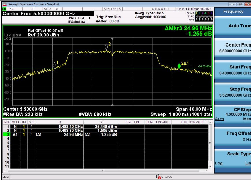
11AC20SISO-Ant2-5500
