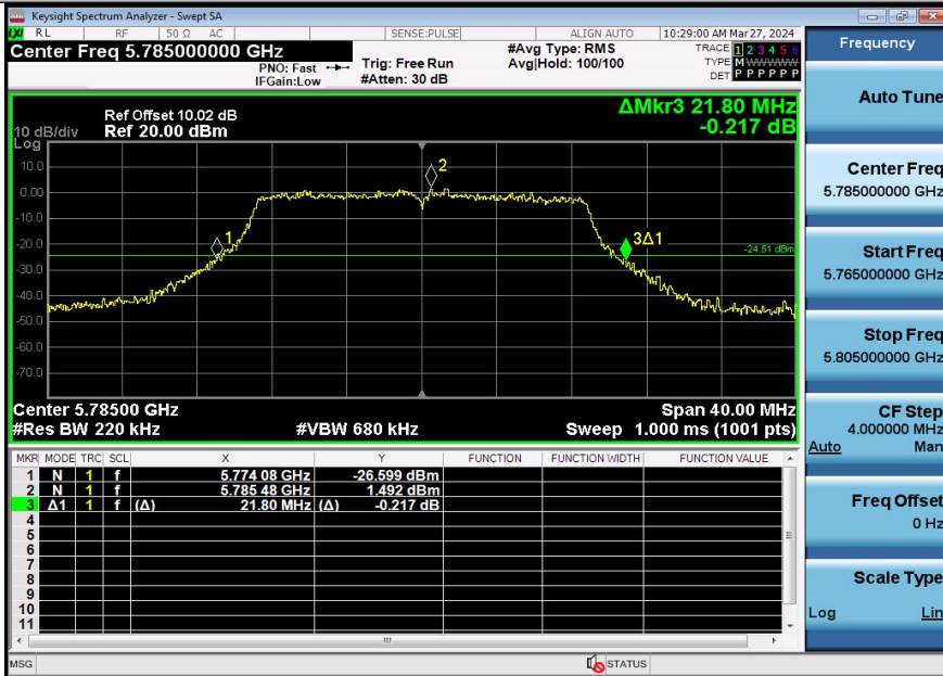
11AC20SISO-Ant2-5785
