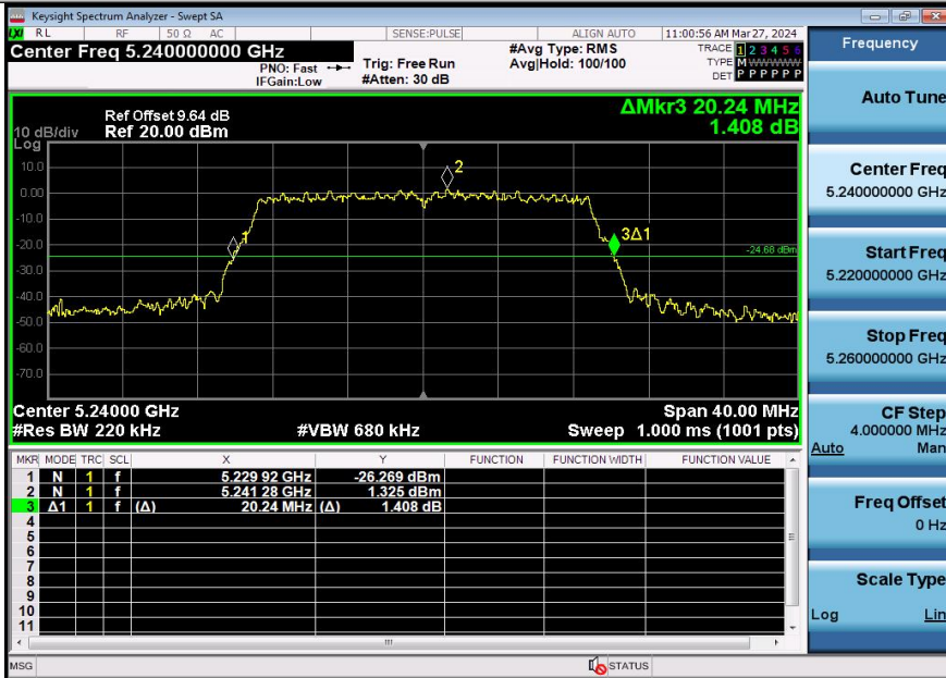
11AX20SISO-Ant2-5240
