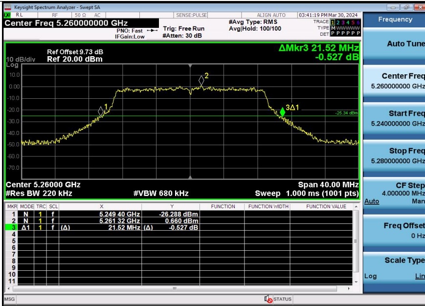
11AC20SISO-Ant2-5260
