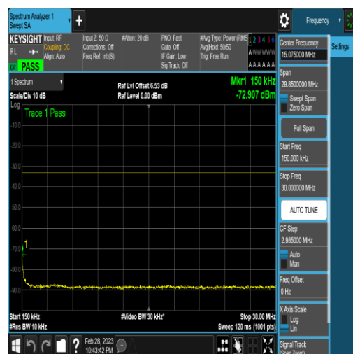
NTNV_N78-3700-3800_PC2_30_20_H_TID4_N/A _0.15_30_#1
