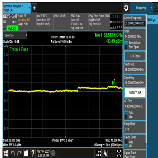
NTNV_DC_2A_n78A-3700-3800_PC3_30_5+100 _M+H_TID6_NS_01_26000_40000_#1
