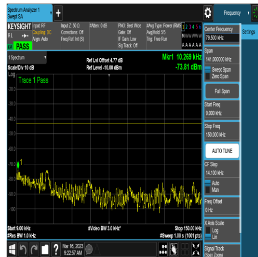
NTNV_DC_2A_n78A-3700-3800_PC3_30_5+100 _M+H_TID16_NS_01_0.009_0.15_#1
