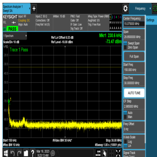
NTNV_DC_2A_n78A-3700-3800_PC3_30_5+100 _M+H_TID16_NS_01_0.15_30_#1
