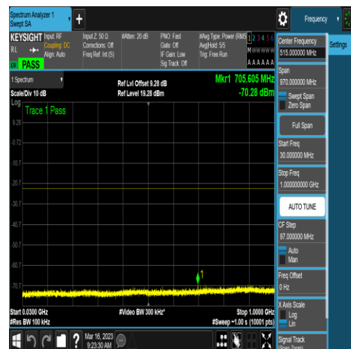
NTNV_DC_2A_n78A-3700-3800_PC3_30_5+100 _M+H_TID16_NS_01_30_1000_#1
