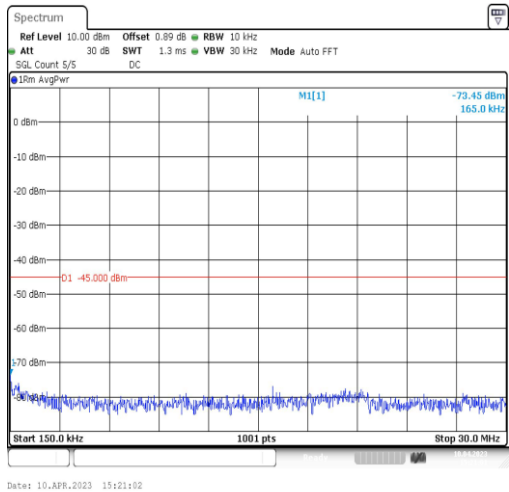
41-41-5MHz-20MHz-QPSK-QPSK-41373-41490-1RB#0-0RB#0-0.15~30MHz
