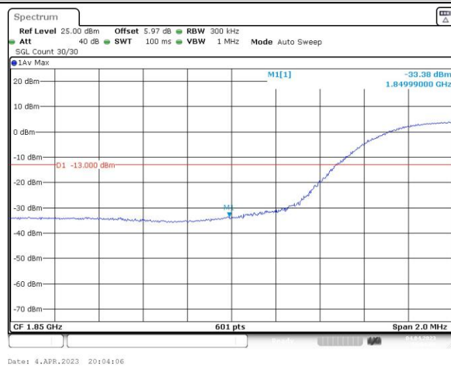
Band25-15MHz-16QAM-26615-1RB#0
