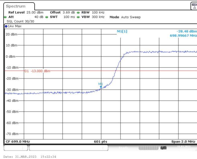
Band12-5MHz-16QAM-23155-1RB#0
