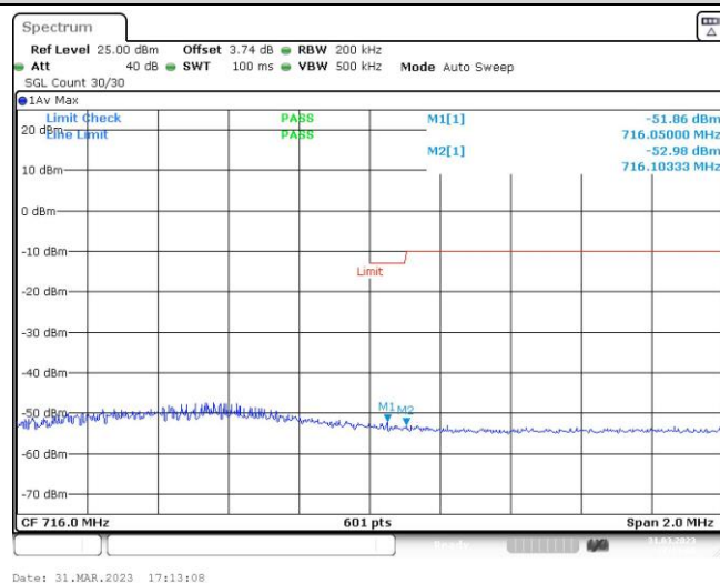
Band12-10MHz-16QAM-23130-1RB#49
