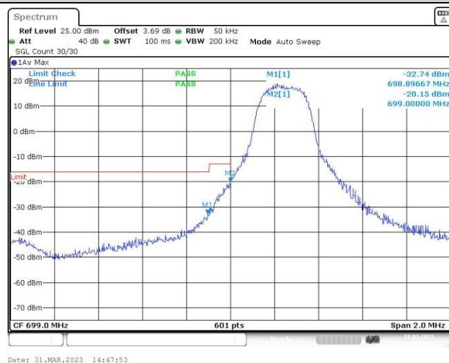
Band12-3MHz-16QAM-23025-1RB#14
