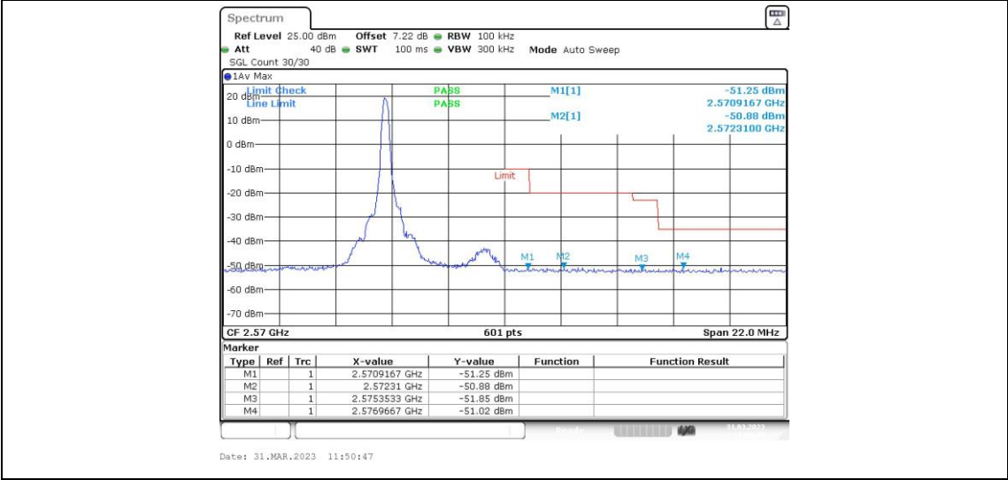
Band7-5MHz-QPSK-21425-1RB#24
