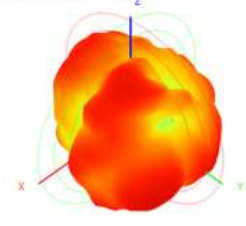
2500.0MHz H+V, Eff: 62.1%
