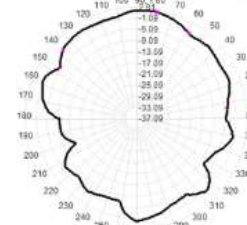
Total(H+V), Max= 1.87dBi, Crd=15.79
