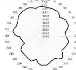
Total(H+V), Max= 1.76dBi, Crd=15.80
