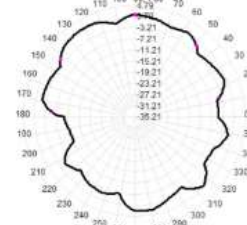
Total(H+V), Max= 1.58dBi, Crd=13.41
