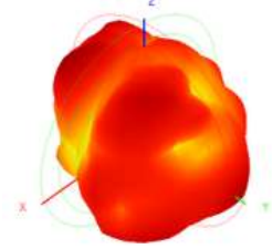
2400.0MHz H+V, Eff: 63.8%
