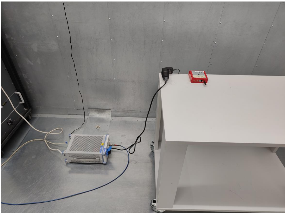
Figure 6: Conducted measurements on AC lines test setup
