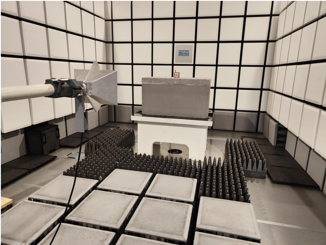
Figure 3: Spurious emission 1-18 GHz
