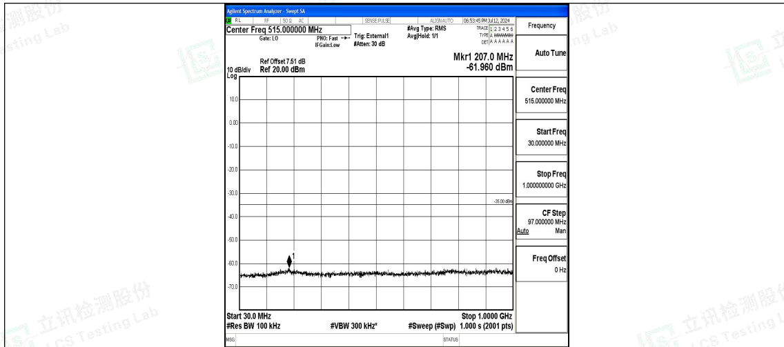
Band41_10MHz_16QAM_40620_1RB#0_30~1000_30~1000
