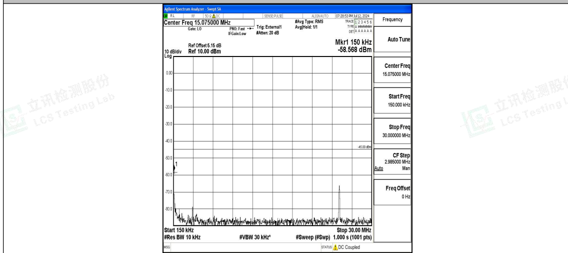
Band41_15MHz_16QAM_40620_1RB#0_0.15~30_0.15~30
