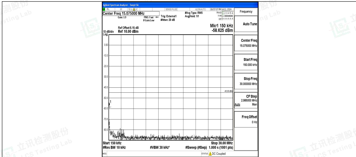
Band41_10MHz_16QAM_41540_1RB#0_0.15~30_0.15~30
