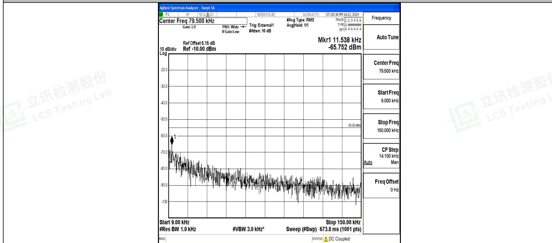
Band41_15MHz_QPSK_40620_1RB#0_0.009~0.15_0.009~0.15
