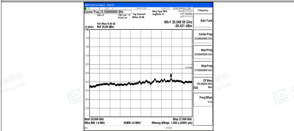
Band41_10MHz_QPSK_41540_1RB#0_20000~27000_20000~27000
