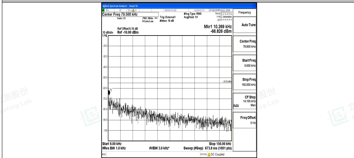
Band41_15MHz_16QAM_40620_1RB#0_0.009~0.15_0.009~0.15
