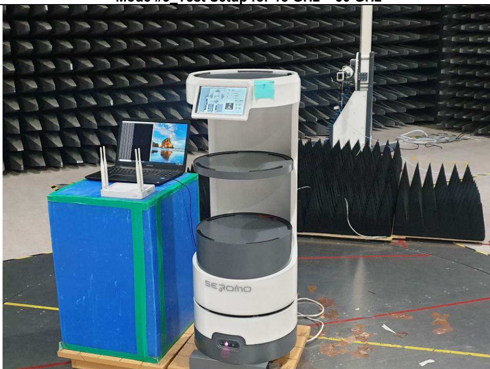
Mode #3 Test Setup for 18 GHz ~ 30 GHz
