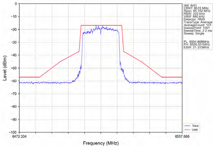
802.11ax(HEW20)_HCH_6515MHz_RU242_Left_Ant1_NTNV
