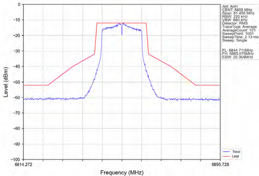
802.11a_HCH_6855MHz_Ant1_NTNV
