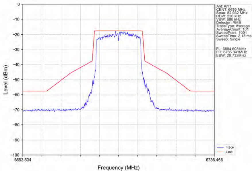
802.11ax(HEW20)_MCH_6695MHz_RU242_Left_Ant1_NTNV
