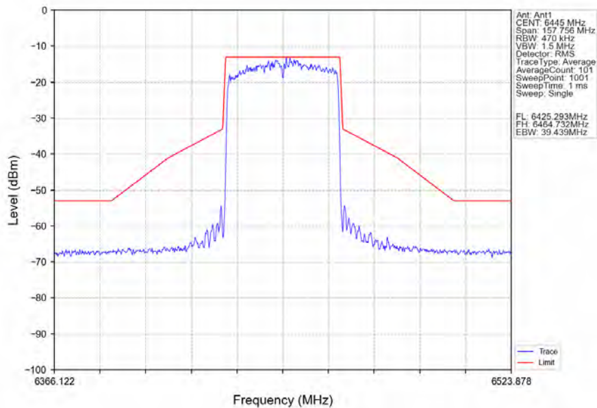
802.11ax(HEW40)_LCH_6445MHz_RU484_Left_Ant1_NTNV
