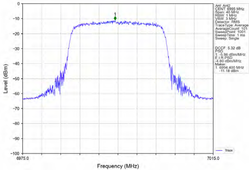
802.11ax(HEW20)_MCH_6995MHz_RU242_Left_Ant2_NTNV
