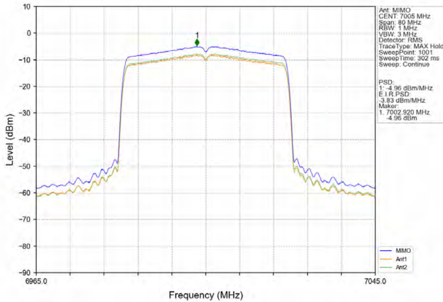
802.11ax(HEW40)_MCH_7005MHz_RU484_Left_MIMO_NTNV
