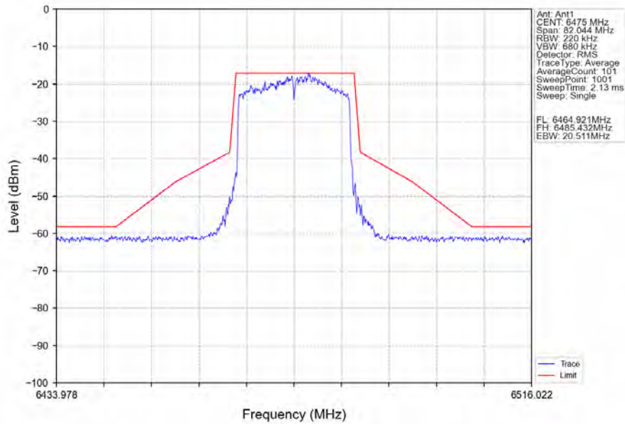
802.11ax(HEW20)_MCH_6475MHz_RU242_Left_Ant1_NTNV
