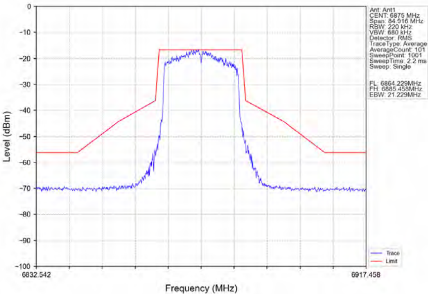
802.11ax(HEW20)_HCH_6875MHz_RU242_Left_Ant1_NTNV
