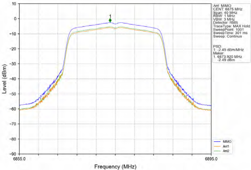
802.11ax(HEW20)_HCH_6875MHz_RU242_Left_MIMO_NTNV
