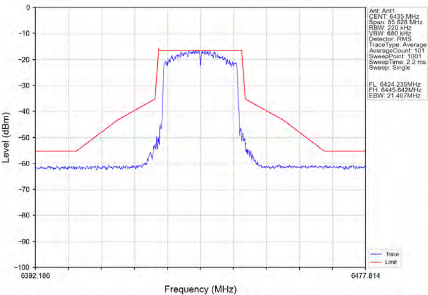
802.11ax(HEW20)_LCH_6435MHz_RU242_Left_Ant1_NTNV
