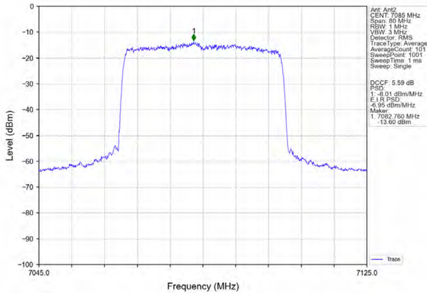
802.11ax(HEW40)_HCH_7085MHz_RU484_Left_Ant2_NTNV
