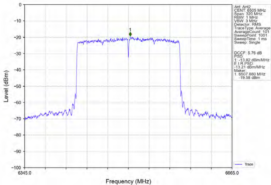
802.11ax(HEW160)_HCH_6505MHz_2xRU996_Left_Ant2_NTNV
