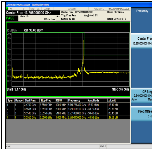
NTNV-n77(3450-3550)-PC2-30-80-H-DFT-BPSK- Edge_1RB_Right-PASS
