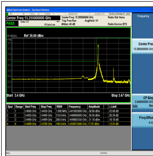
NTNV-n77(3450-3550)-PC2-30-20-L-DFT-BPSK- Edge_1RB_Left-PASS
