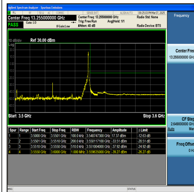
NTNV-n77(3450-3550)-PC2-30-50-H-CP-QPSK- Edge_1RB_Right-PASS
