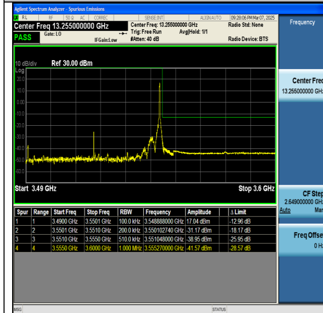
NTNV-n77(3450-3550)-PC2-30-60-H-CP-QPSK- Edge_1RB_Right-PASS
