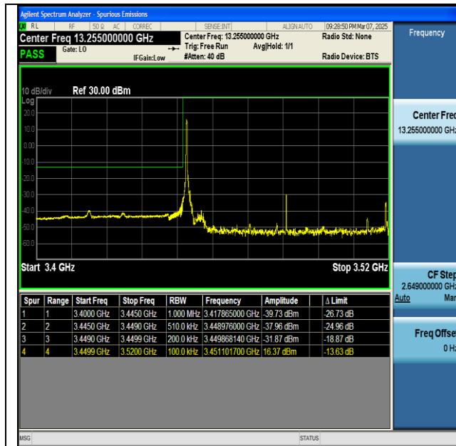
NTNV-n77(3450-3550)-PC2-30-70-L-DFT-BPSK- Edge_1RB_Left-PASS
