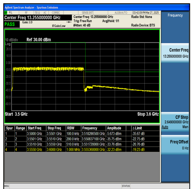
NTNV-n77(3450-3550)-PC2-30-50-H-CP-QPSK- Outer_Full-PASS
