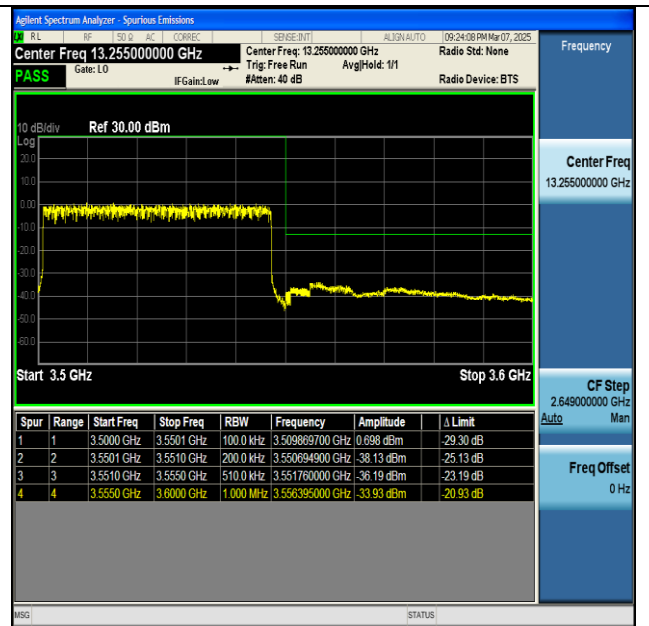
NTNV-n77(3450-3550)-PC2-30-50-H-DFT-BPSK- Outer_Full-PASS
