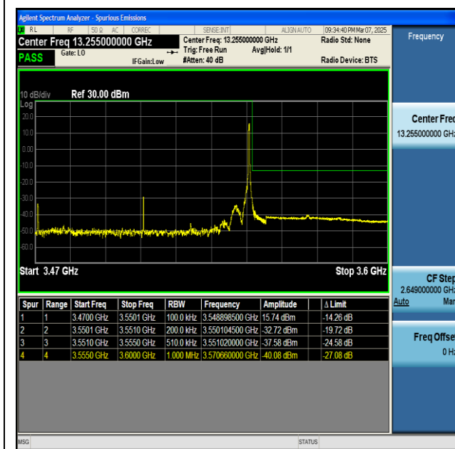
NTNV-n77(3450-3550)-PC2-30-80-H-CP-QPSK- Edge_1RB_Right-PASS
