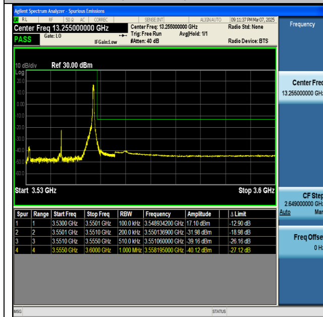
NTNV-n77(3450-3550)-PC2-30-20-H-CP-QPSK- Edge_1RB_Right-PASS
