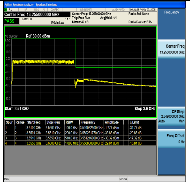
NTNV-n77(3450-3550)-PC2-30-40-H-CP-QPSK- Outer_Full-PASS
