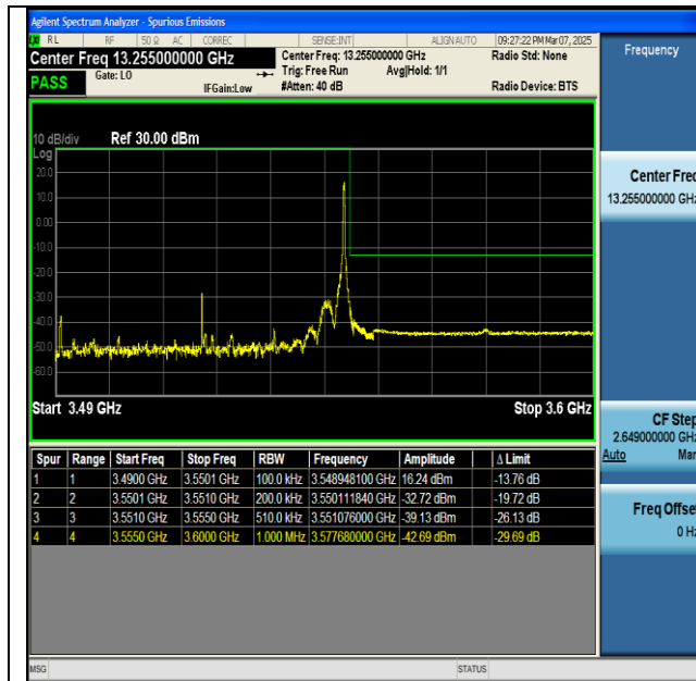
NTNV-n77(3450-3550)-PC2-30-60-H-DFT-BPSK- Edge_1RB_Right-PASS
