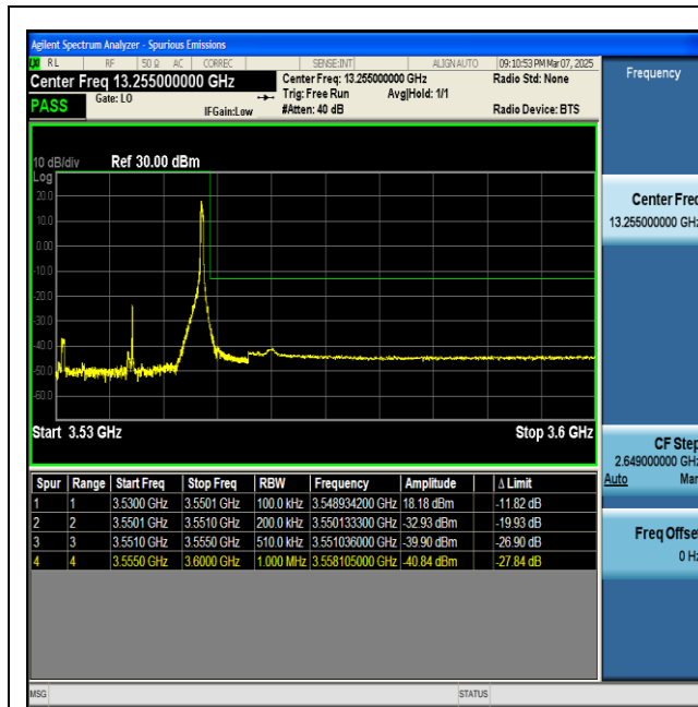
NTNV-n77(3450-3550)-PC2-30-20-H-DFT-BPSK- Edge_1RB_Right-PASS
