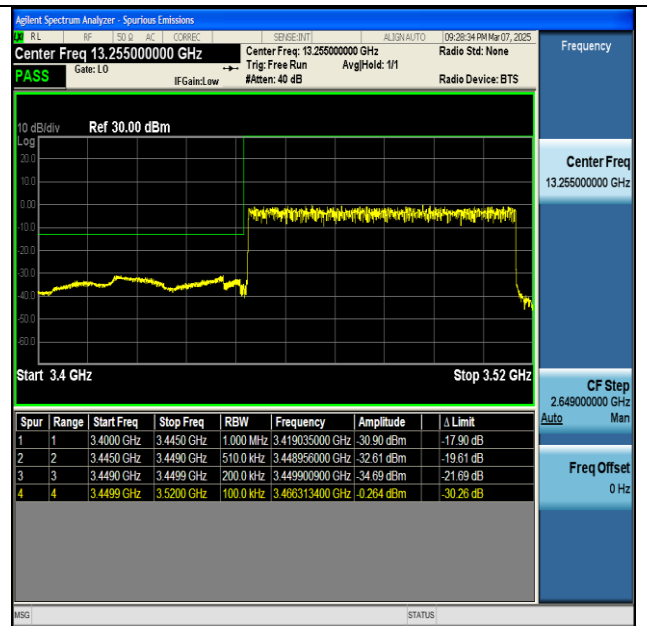
NTNV-n77(3450-3550)-PC2-30-70-L-DFT-BPSK- Outer_Full-PASS
