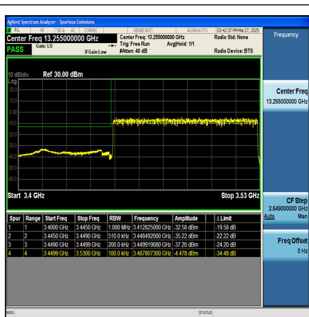
NTNV-n77(3450-3550)-PC2-30-80-L-DFT-BPSK- Outer_Full-PASS
