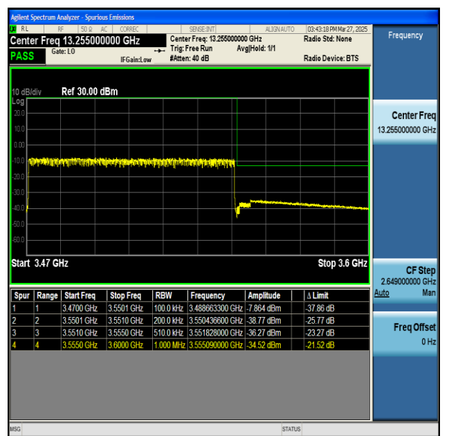
NTNV-n77(3450-3550)-PC2-30-80-H-CP-QPSK- Outer_Full-PASS
