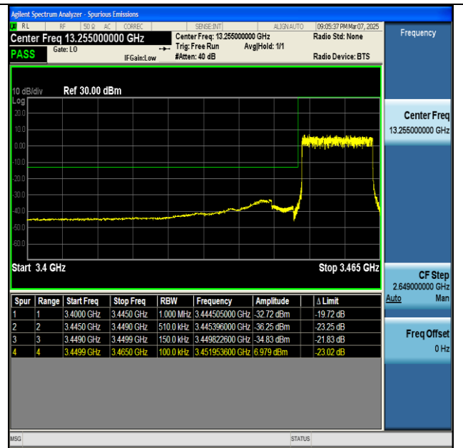
NTNV-n77(3450-3550)-PC2-30-15-L-DFT-BPSK- Outer_Full-PASS
