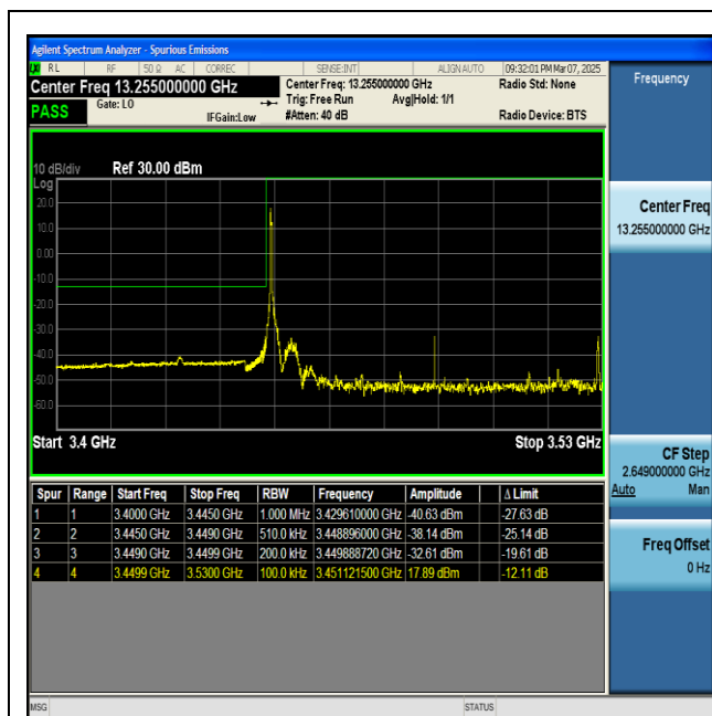
NTNV-n77(3450-3550)-PC2-30-80-L-DFT-BPSK- Edge_1RB_Left-PASS
