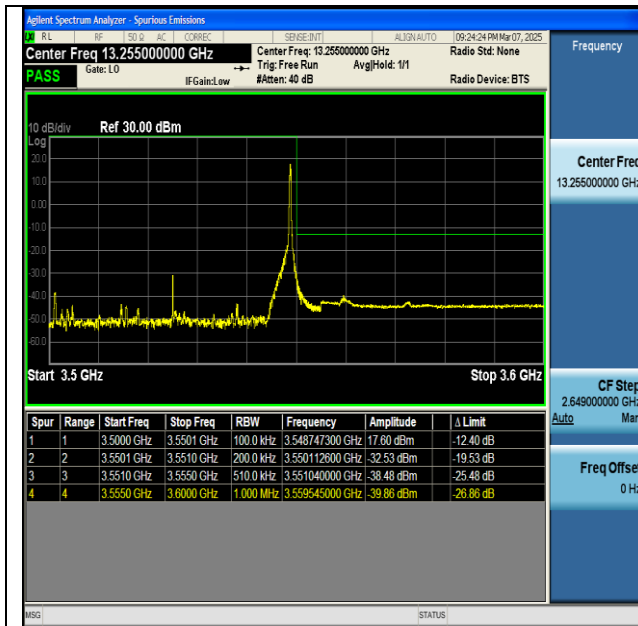
NTNV-n77(3450-3550)-PC2-30-50-H-DFT-BPSK- Edge_1RB_Right-PASS
