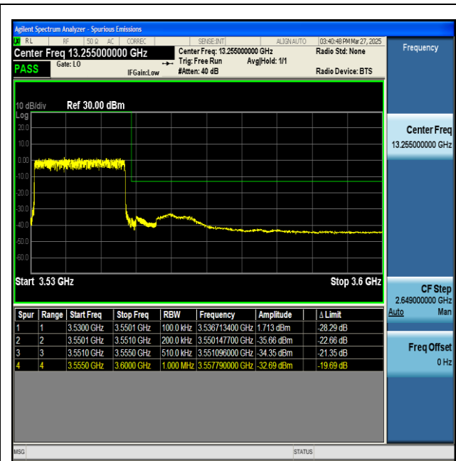
NTNV-n77(3450-3550)-PC2-30-20-H-DFT-BPSK- Outer_Full-PASS
