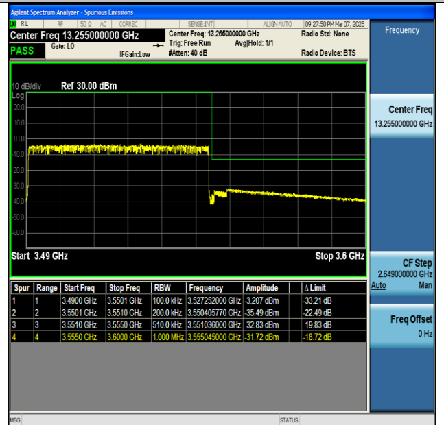
NTNV-n77(3450-3550)-PC2-30-60-H-CP-QPSK- Outer_Full-PASS
