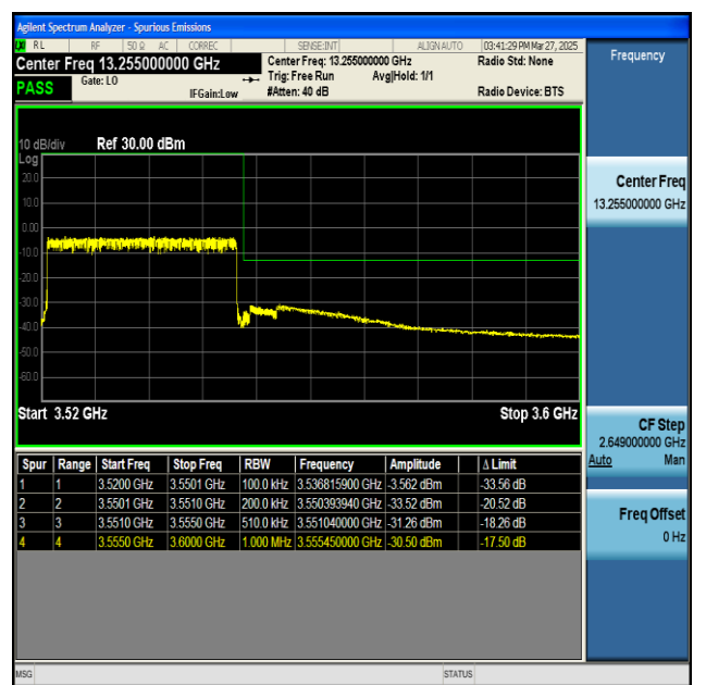
NTNV-n77(3450-3550)-PC2-30-30-H-CP-QPSK- Outer_Full-PASS
