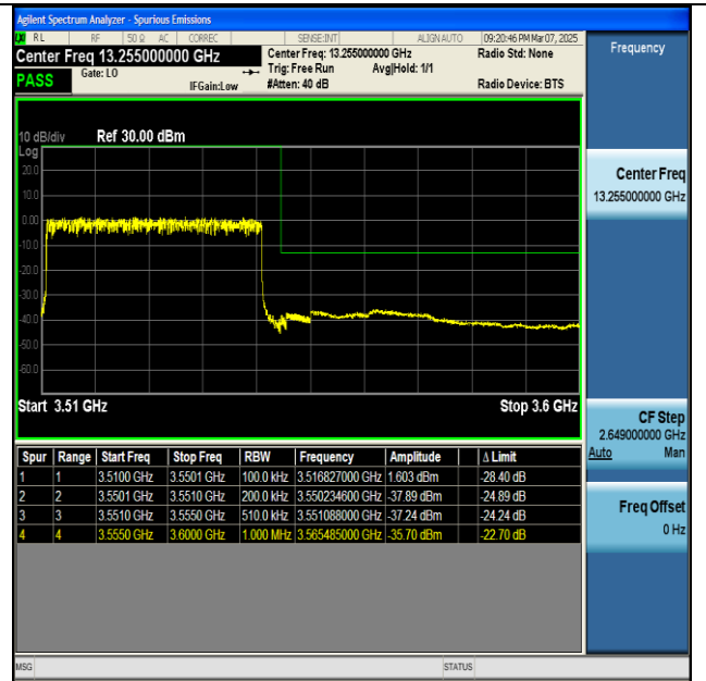
NTNV-n77(3450-3550)-PC2-30-40-H-DFT-BPSK- Outer_Full-PASS
