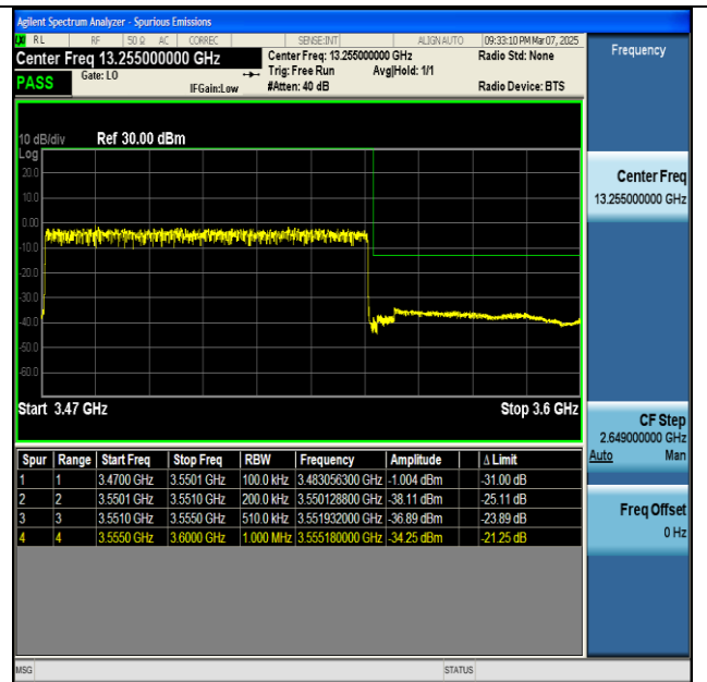
NTNV-n77(3450-3550)-PC2-30-80-H-DFT-BPSK- Outer_Full-PASS
