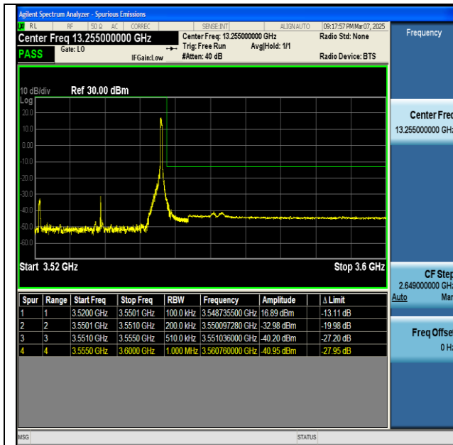
NTNV-n77(3450-3550)-PC2-30-30-H-DFT-BPSK- Edge_1RB_Right-PASS
