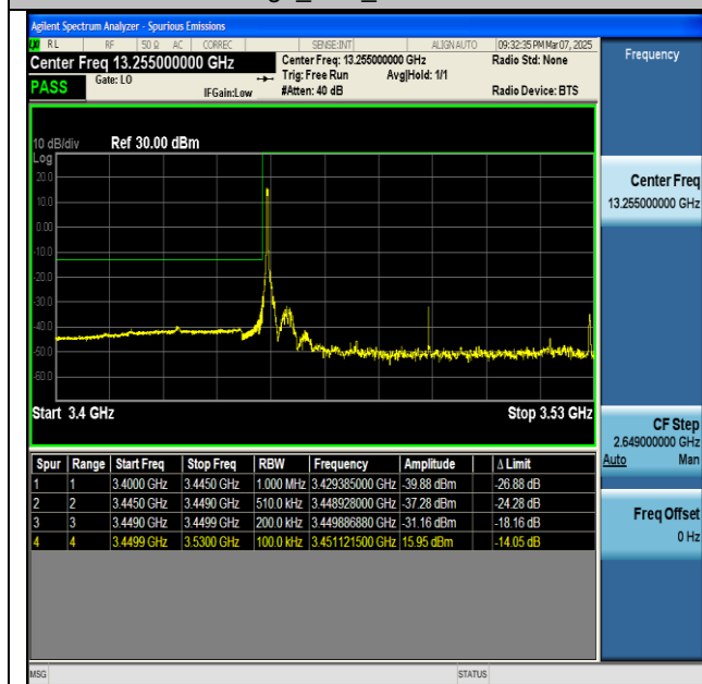
NTNV-n77(3450-3550)-PC2-30-80-L-CP-QPSK- Edge_1RB_Left-PASS
