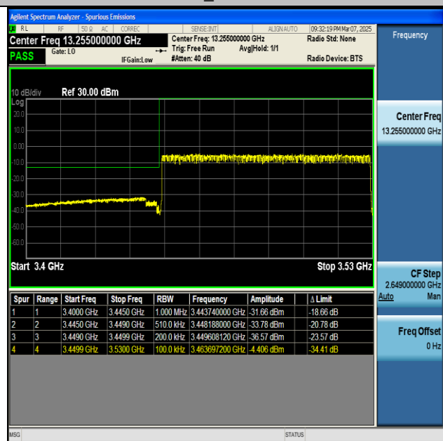
NTNV-n77(3450-3550)-PC2-30-80-L-CP-QPSK- Outer_Full-PASS
