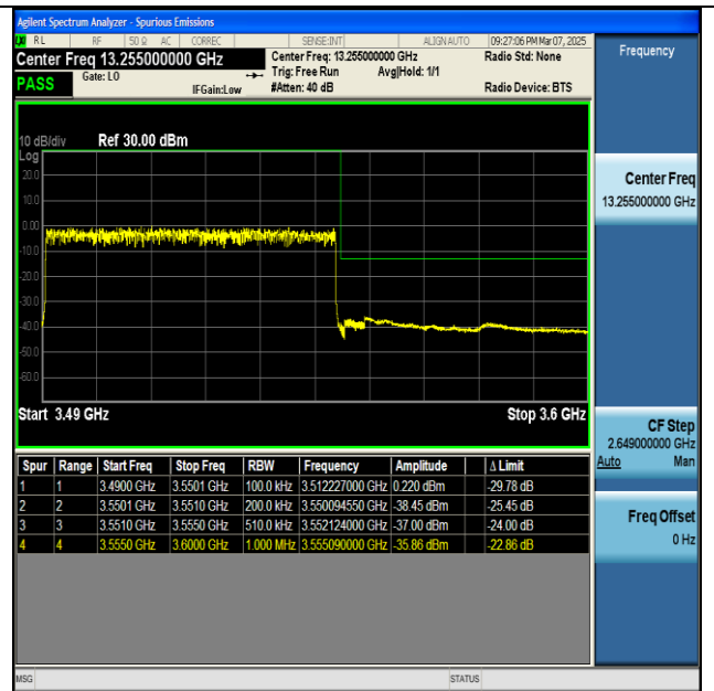
NTNV-n77(3450-3550)-PC2-30-60-H-DFT-BPSK- Outer_Full-PASS
