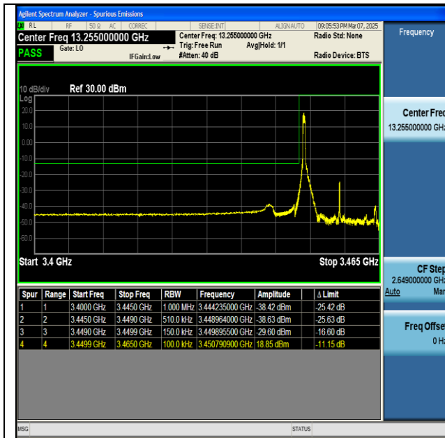
NTNV-n77(3450-3550)-PC2-30-15-L-DFT-BPSK- Edge_1RB_Left-PASS
