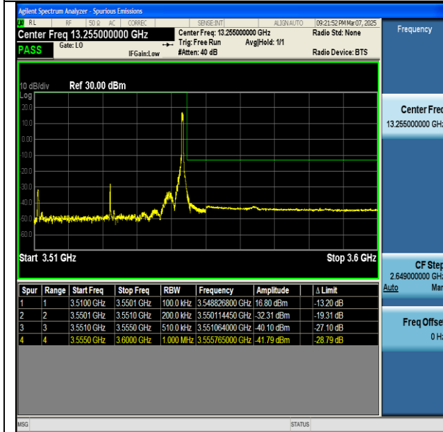
NTNV-n77(3450-3550)-PC2-30-40-H-CP-QPSK- Edge_1RB_Right-PASS
