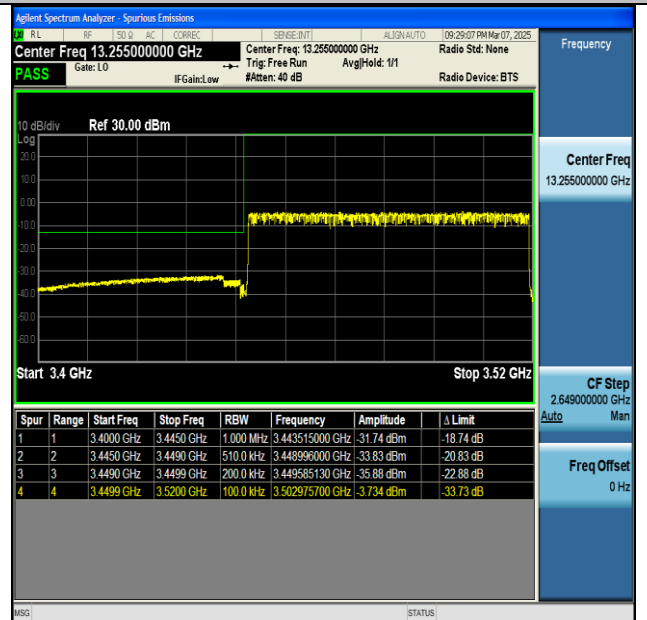
NTNV-n77(3450-3550)-PC2-30-70-L-CP-QPSK- Outer_Full-PASS
