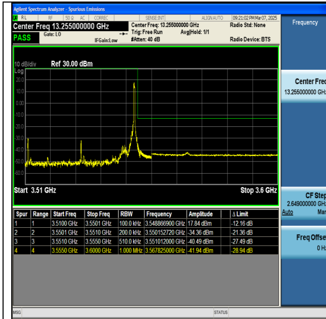
NTNV-n77(3450-3550)-PC2-30-40-H-DFT-BPSK- Edge_1RB_Right-PASS
