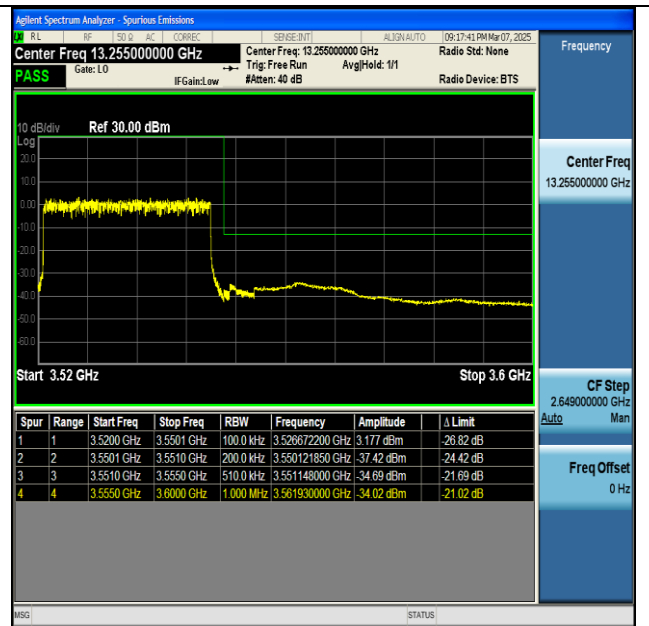
NTNV-n77(3450-3550)-PC2-30-30-H-DFT-BPSK- Outer_Full-PASS
