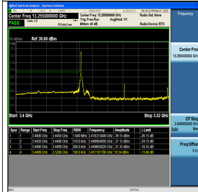
NTNV-n77(3450-3550)-PC2-30-70-L-CP-QPSK- Edge_1RB_Left-PASS
