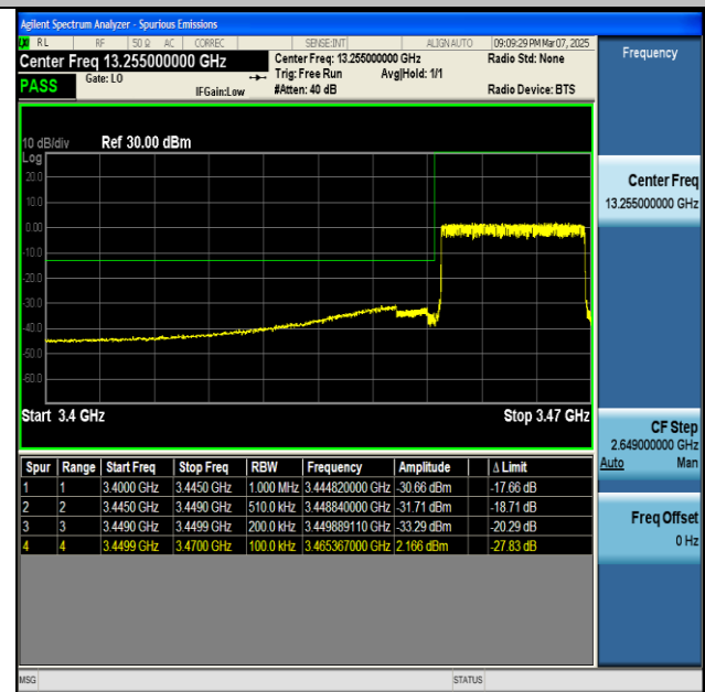
NTNV-n77(3450-3550)-PC2-30-20-L-CP-QPSK- Outer_Full-PASS
