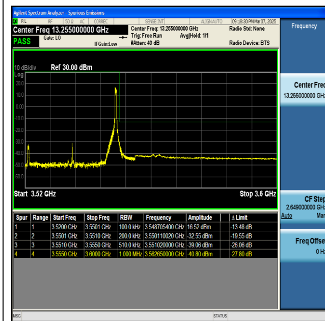
NTNV-n77(3450-3550)-PC2-30-30-H-CP-QPSK- Edge_1RB_Right-PASS
