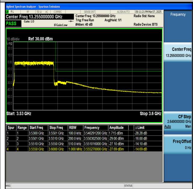
NTNV-n77(3450-3550)-PC2-30-20-H-CP-QPSK- Outer_Full-PASS
