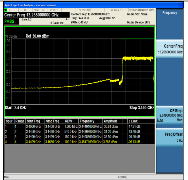
NTNV-n77(3450-3550)-PC2-30-15-L-CP-QPSK- Outer_Full-PASS
