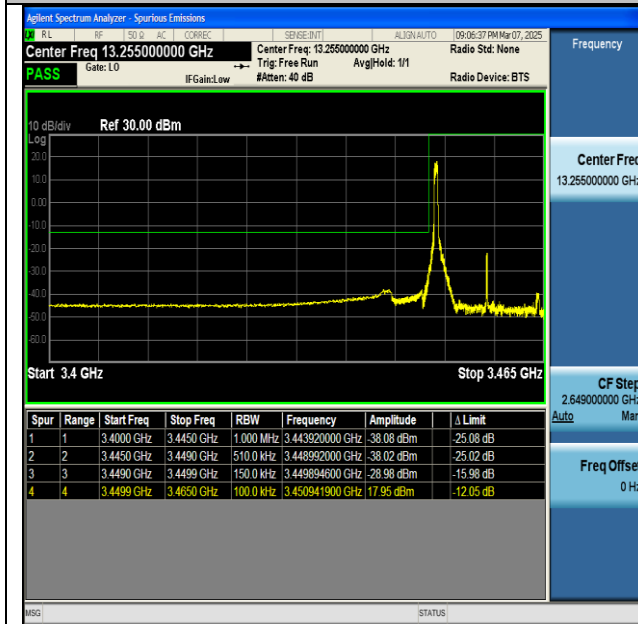
NTNV-n77(3450-3550)-PC2-30-15-L-CP-QPSK- Edge_1RB_Left-PASS
