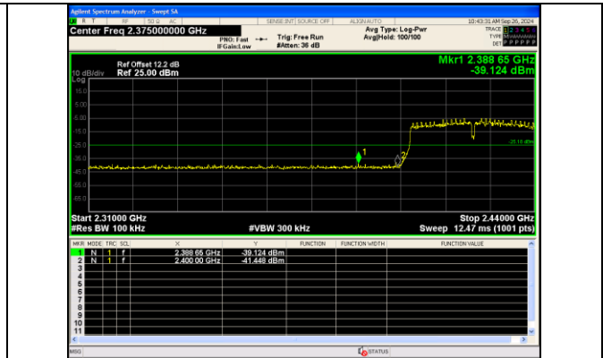
Out Of Band Emission IEEE 802.11n_Channel 3_40MHz_Antenna 0
