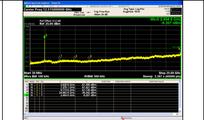
30.0 MHz - 25000.0 MHz IEEE 802.11n_Channel 9_40MHz_Antenna 0
