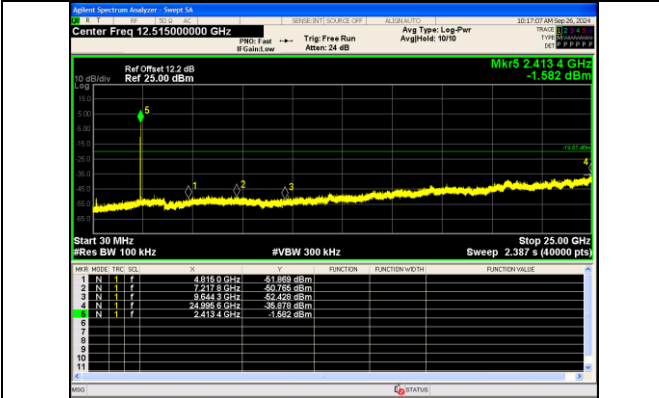
30.0 MHz - 25000.0 MHz IEEE 802.11b Channel 1 20MHz Antenna 0
