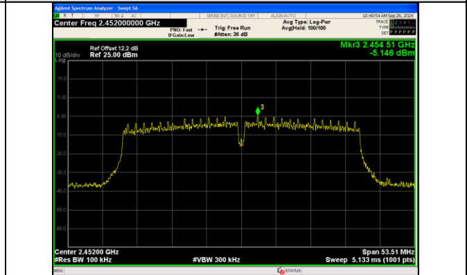
In-Band Reference Level IEEE 802.11n_Channel 9_40MHz_Antenna 0
