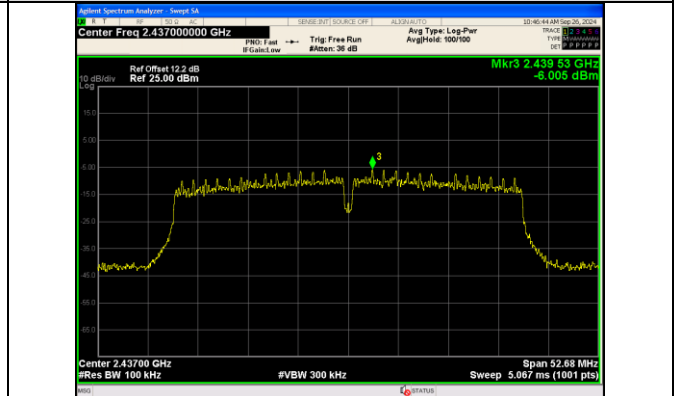
In-Band Reference Level IEEE 802.11n_Channel 6_40MHz_Antenna 0
