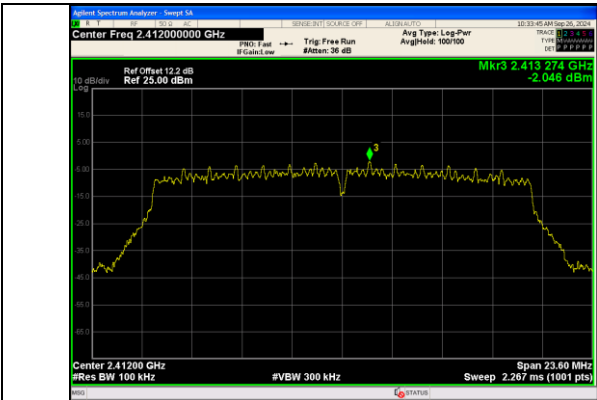
In-Band Reference Level IEEE 802.11n_Channel 1_20MHz_Antenna 0
