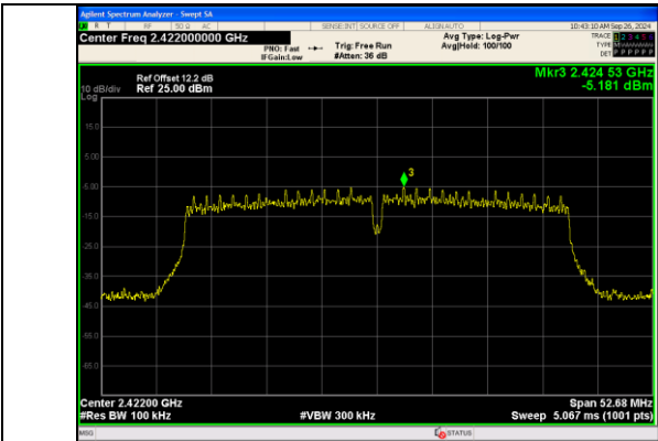
In-Band Reference Level IEEE 802.11n_Channel 3_40MHz_Antenna 0
