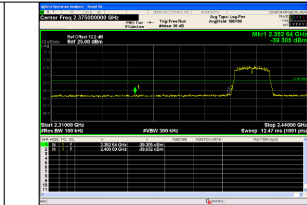
Out Of Band Emission IEEE 802.11n_Channel 1_20MHz_Antenna 0
