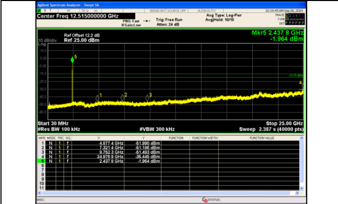
30.0 MHz - 25000.0 MHz IEEE 802.11b Channel 6 20MHz Antenna 0
