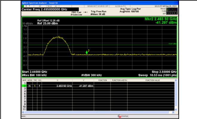
Out Of Band Emission IEEE 802.11b Channel 11 20MHz Antenna 0
