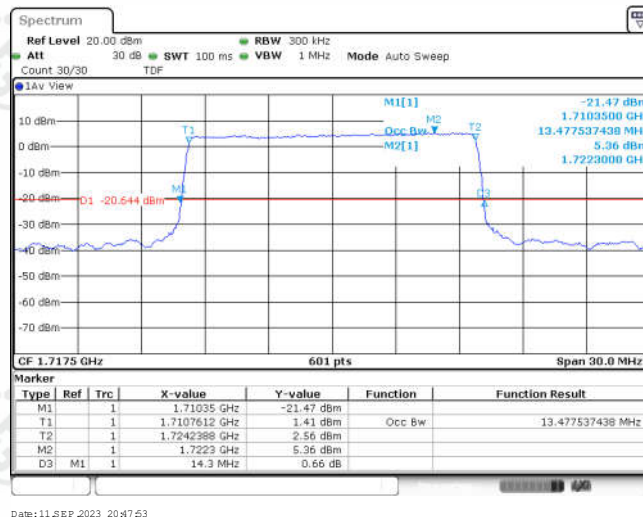
Band4-15MHz-QPSK-20175-75RB#0-13.478
