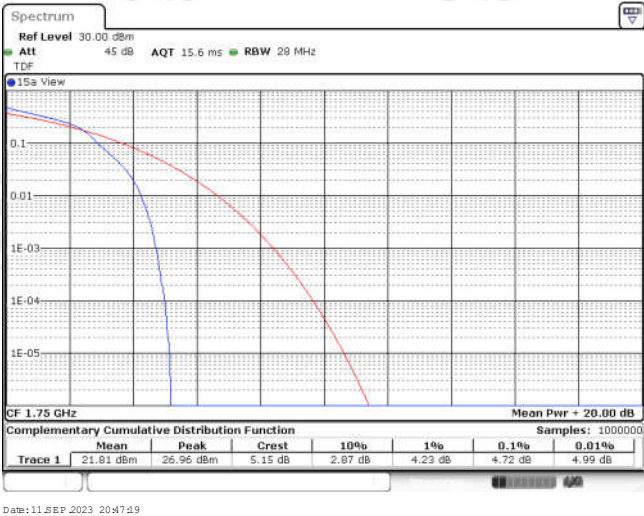
Band4-10MHz-16QAM-20350-50RB#0
