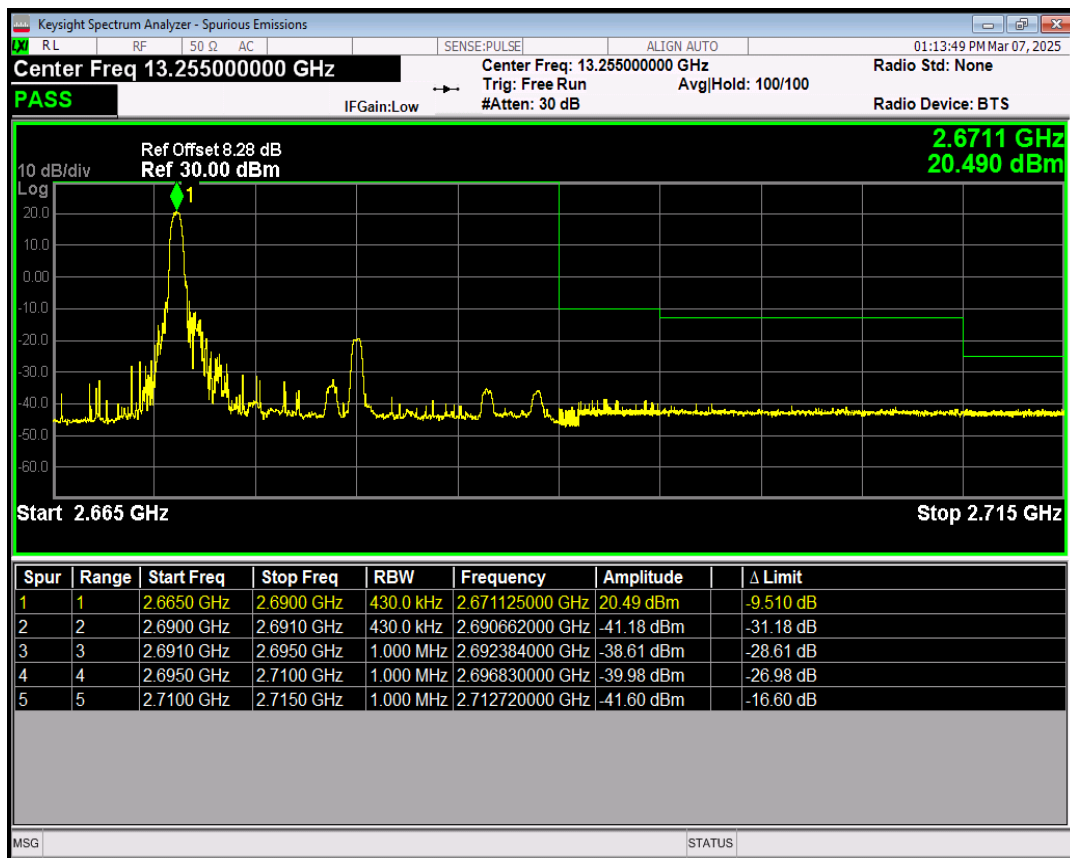
Band41 16QAM BW=20MHz Channel=41490 RB Size=1 Position=#Max
