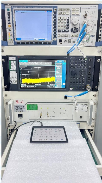
Photo of Setup for RF Conducted----GSM&WCDMA&LTE
