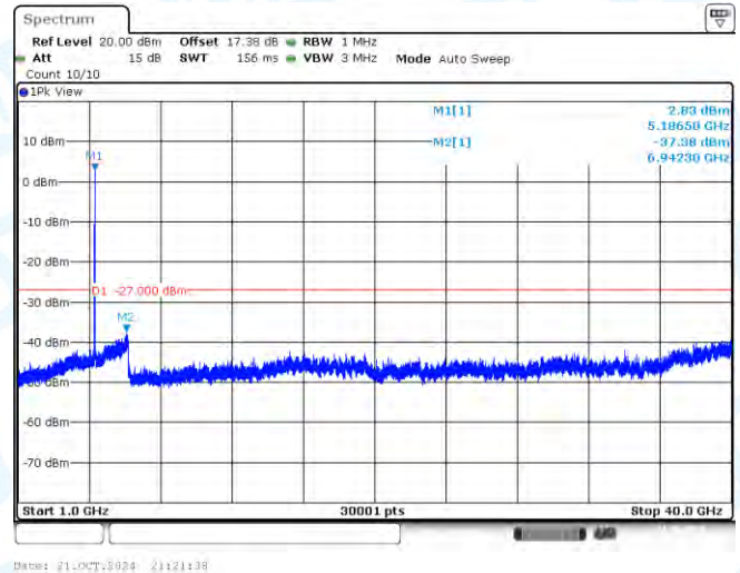
11AC40SISO-Ant1-5190-1000~40000-PASS
