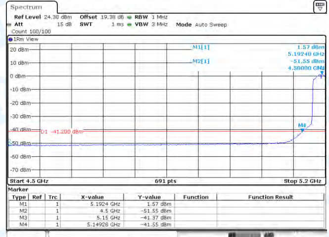
11AC40SISO-Ant1-5190-PASS
