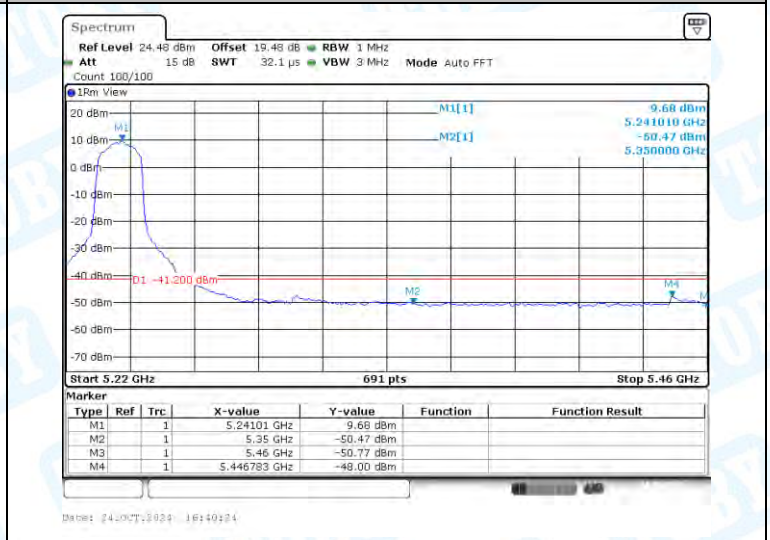
11A-Ant1-5240-PASS
