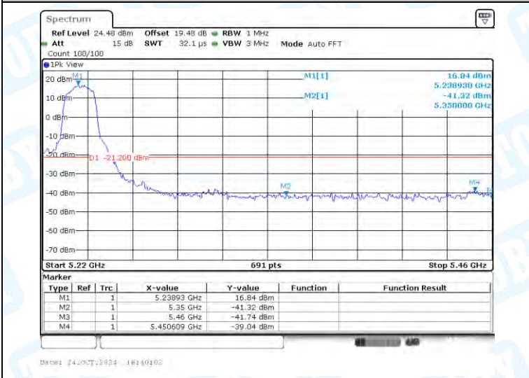
11A-Ant1-5240-PASS
