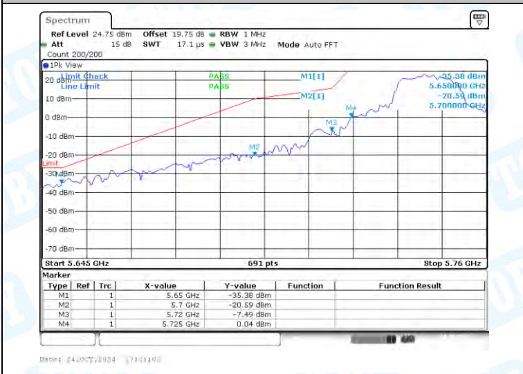
11A-Ant1-5745-PASS
