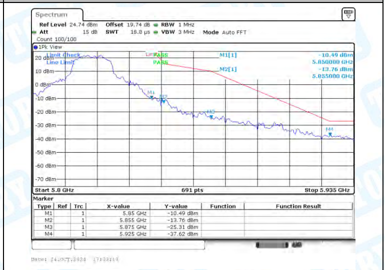
11A-Ant1-5825-PASS
