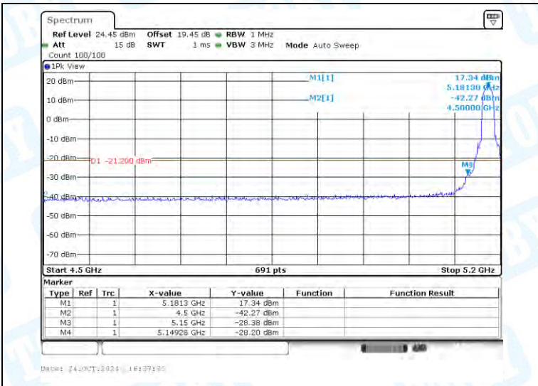
11A-Ant1-5180-PASS
