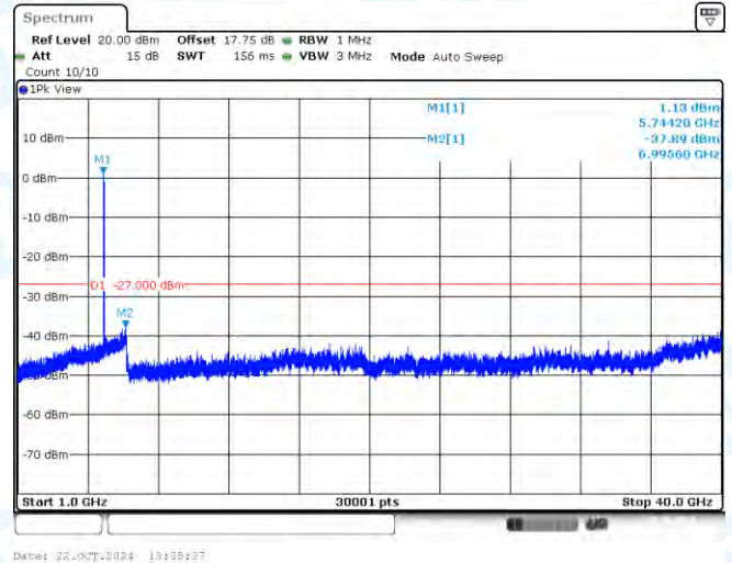
11AX40SISO-Ant1-5755-1000~40000-PASS
