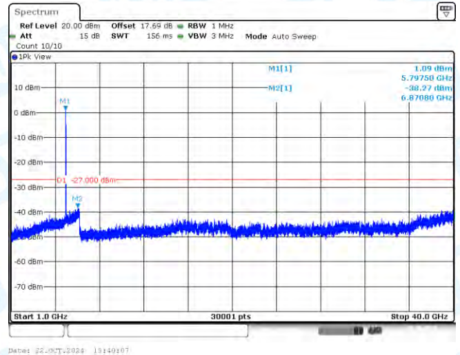
11AX40SISO-Ant1-5795-1000~40000-PASS
