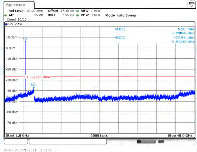
11AC20SISO-Ant1-5240-1000~40000-PASS
