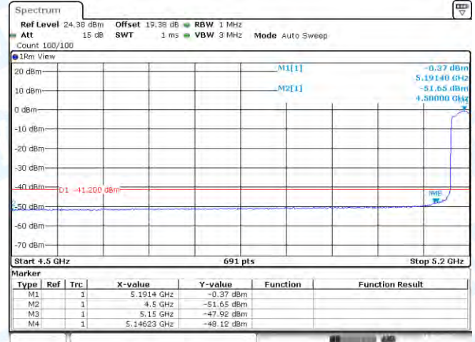
11AX40SISO-Ant1-5190-PASS
