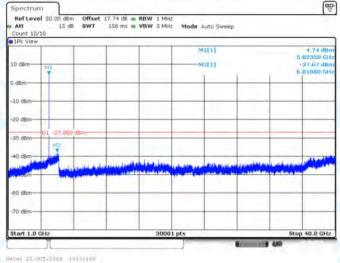
11AX20SISO-Ant1-5825-1000~40000-PASS
