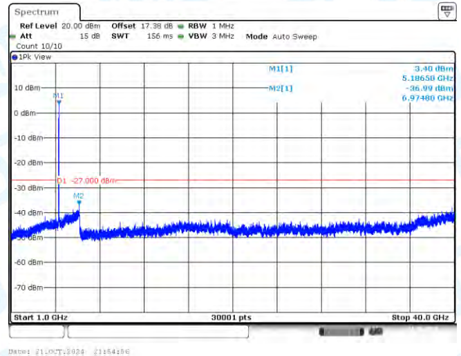
11AX40SISO-Ant1-5190-1000~40000-PASS
