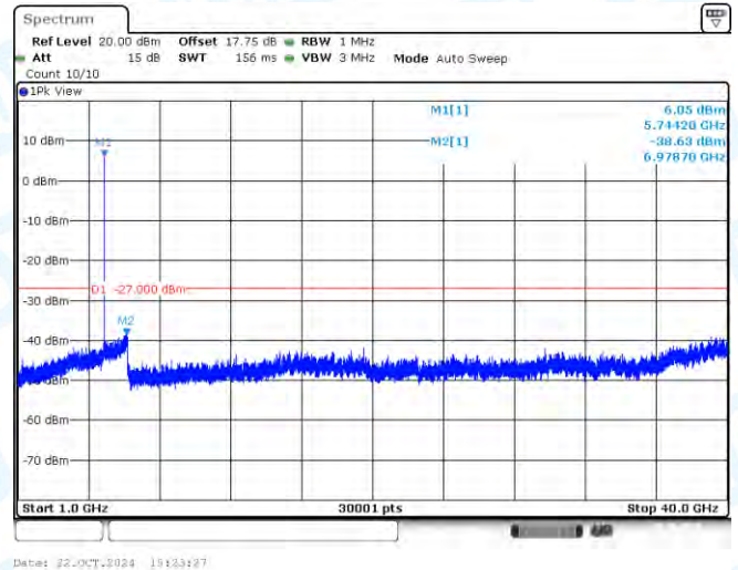
11AX20SISO-Ant1-5745-1000~40000-PASS
