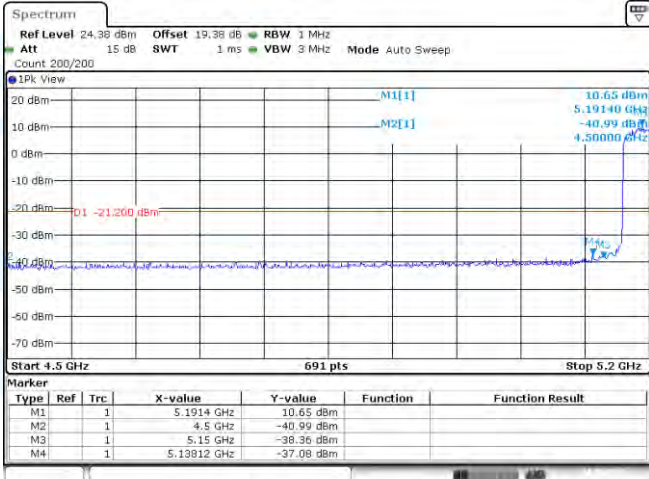
11AX40SISO-Ant1-5190-PASS
