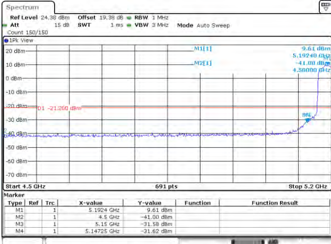
11AC40SISO-Ant1-5190-PASS
