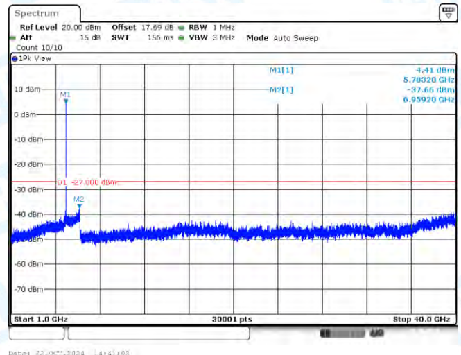
11AC20SISO-Ant1-5785-1000~40000-PASS
