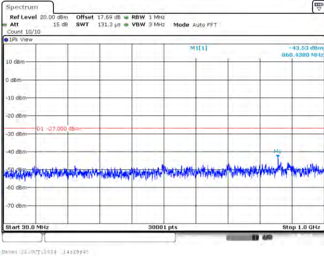
11N40SISO-Ant1-5795-30~1000-PASS
