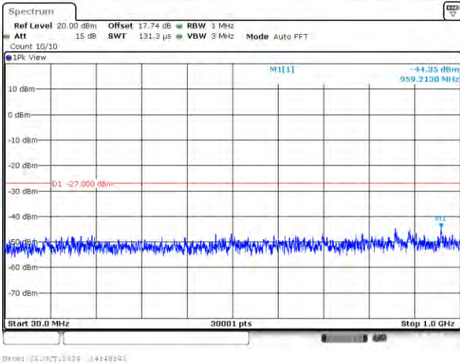
11AC20SISO-Ant1-5825-30~1000-PASS
