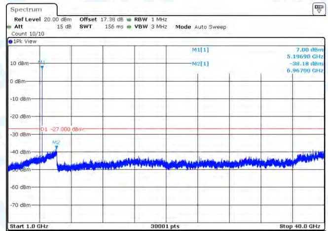
11AX20SISO-Ant1-5180-1000~40000-PASS
