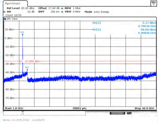
11N40SISO-Ant1-5795-1000~40000-PASS
