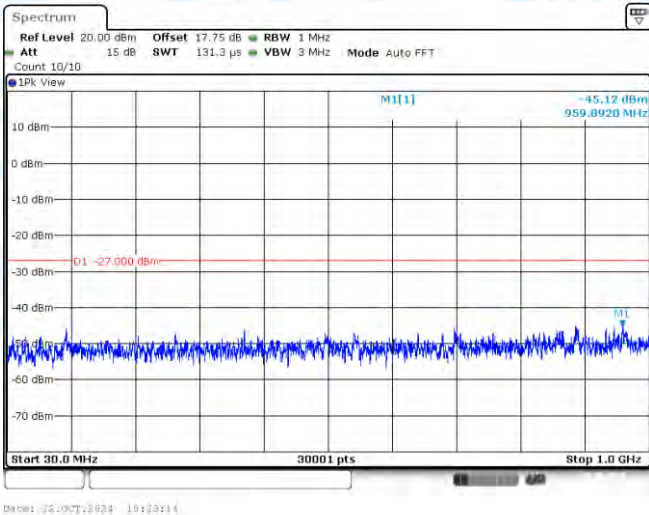
11AX20SISO-Ant1-5745-30~1000-PASS
