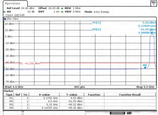
11AX20SISO-Ant1-5180-PASS
