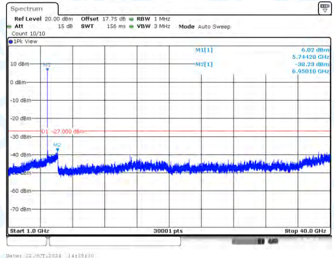
11AC20SISO-Ant1-5745-1000~40000-PASS
