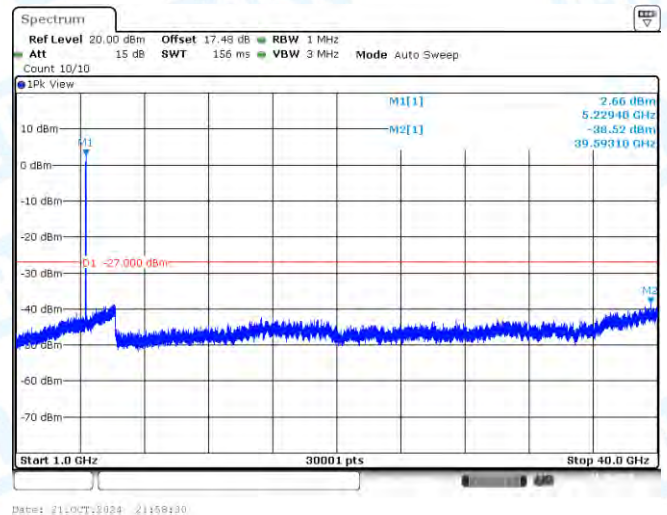
11AX40SISO-Ant1-5230-1000~40000-PASS
