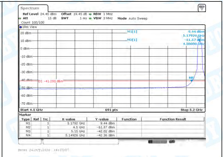
11A-Ant1-5180-PASS
