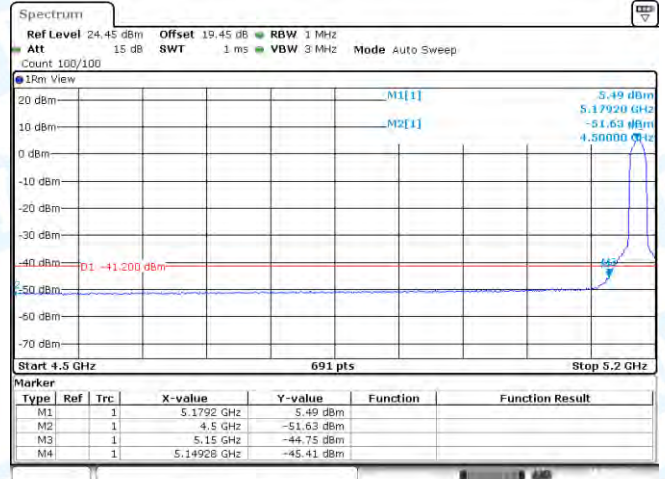
11AC20SISO-Ant1-5180-PASS
