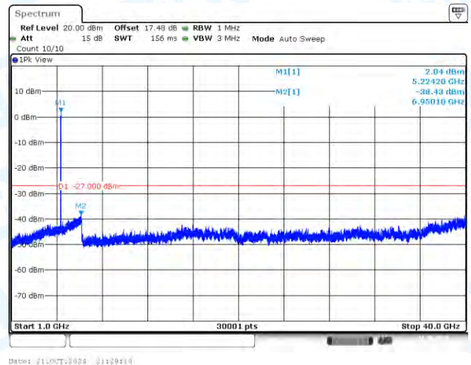
11AC40SISO-Ant1-5230-1000~40000-PASS
