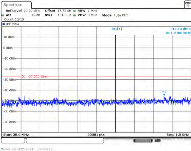
11AX40SISO-Ant1-5755-30~1000-PASS
