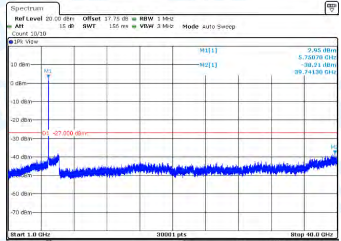
11AC40SISO-Ant1-5755-1000~40000-PASS
