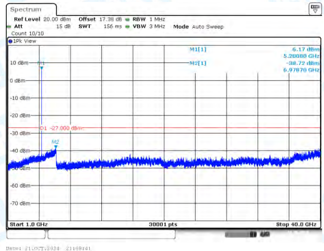
11AC20SISO-Ant1-5200-1000~40000-PASS
