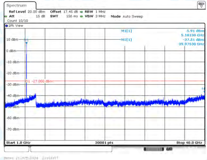
11AC20SISO-Ant1-5180-1000~40000-PASS
