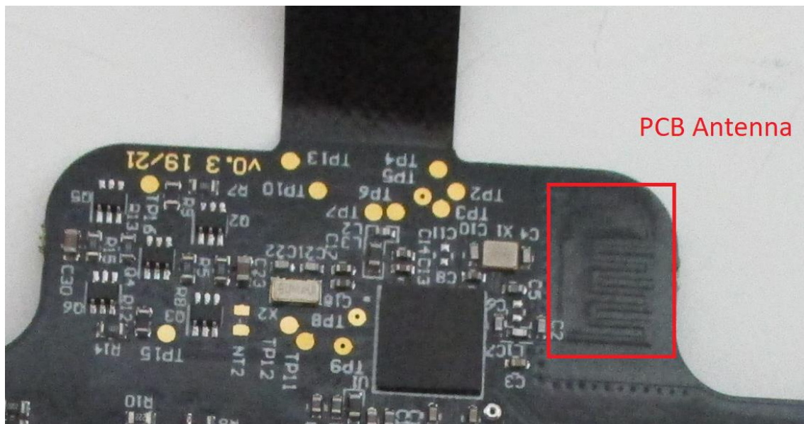
Figure 4: PCB Antenna location
