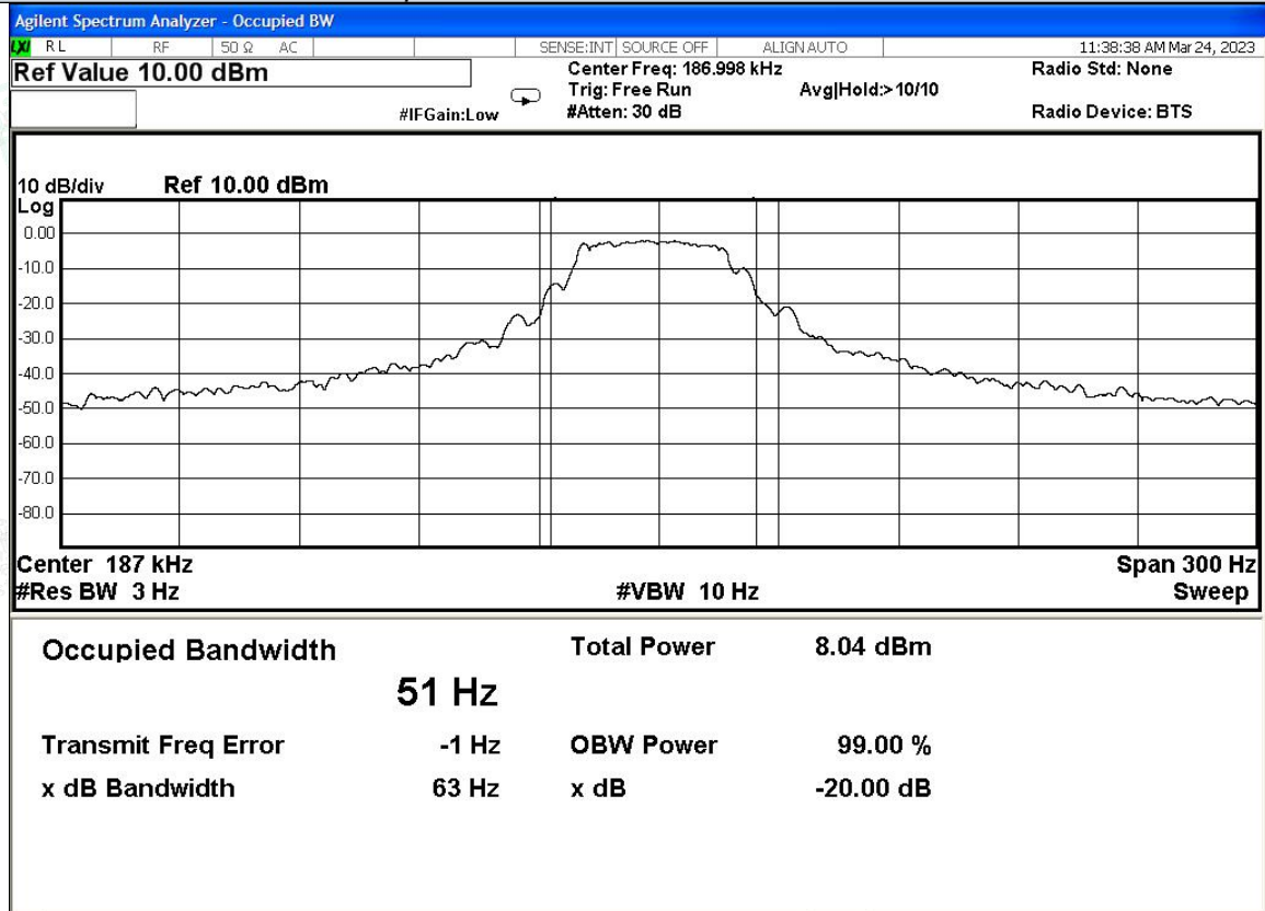
Test plot of 20 dB Bandwidth Measurement
