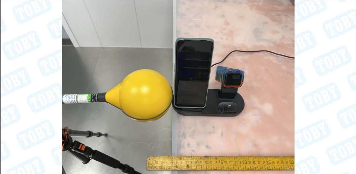
Test Position B - Exposure photo from side edge surface-Left
