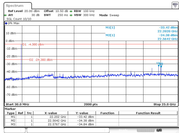
BLE_1M_Low_Channel
