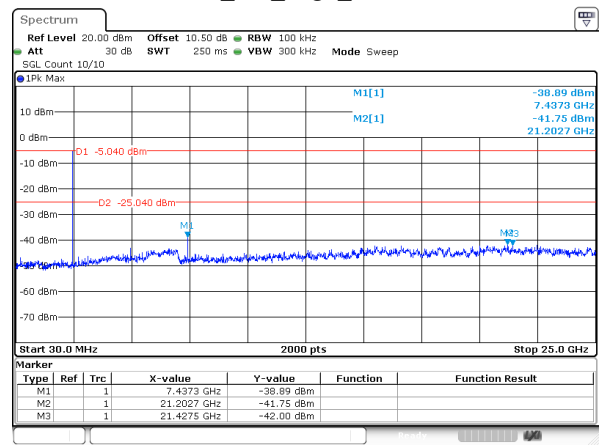
BLE_1M_High_Channel
