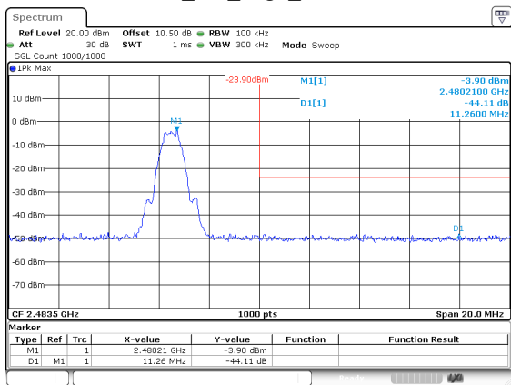
BLE_1M_High_Channel
