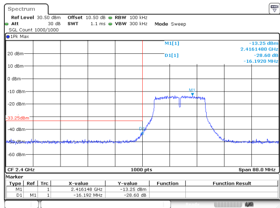
802.11g_2412MHz
