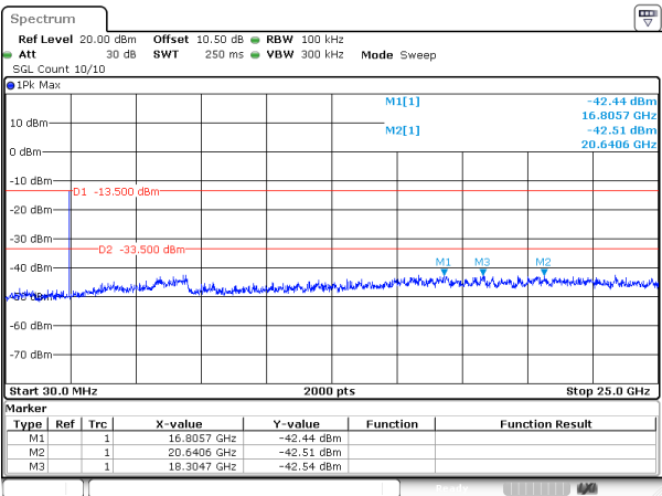
802.11g_2472MHz
