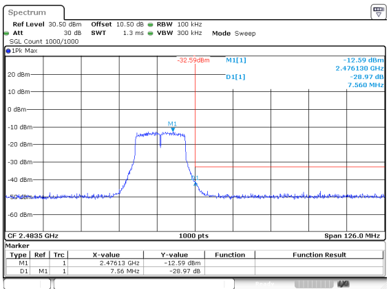
802.11g_2472MHz
