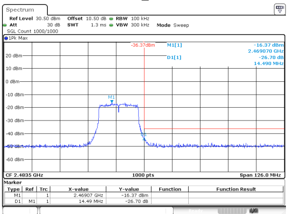
802.11n20_2472MHz
