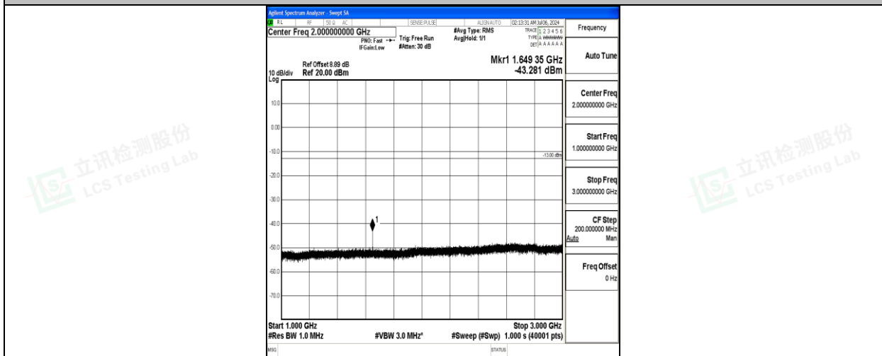
Band5_10MHz_16QAM_20450_1RB#0_1000~3000_1000~3000
