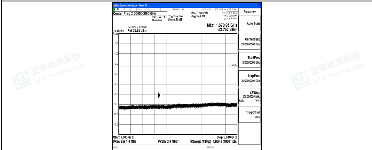
Band5_10MHz_QPSK_20600_1RB#0_1000~3000_1000~3000
