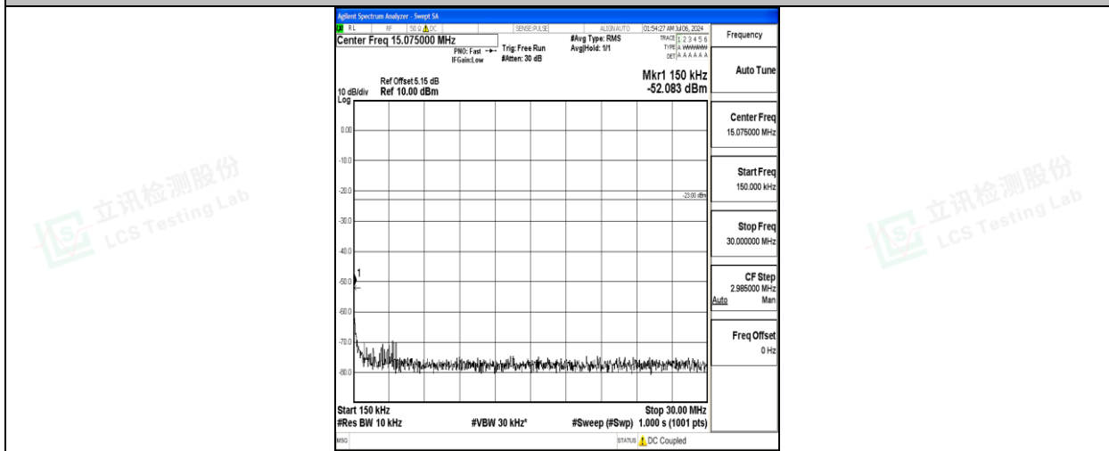
Band5_5MHz_16QAM_20625_1RB#0_0.15~30_0.15~30
