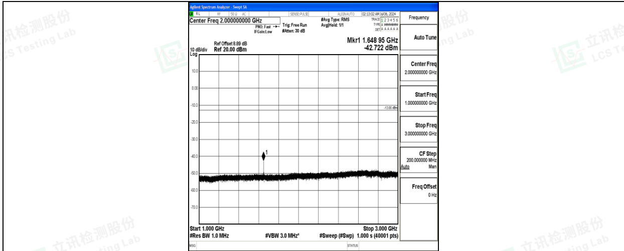
Band5_10MHz_QPSK_20450_1RB#0_1000~3000_1000~3000
