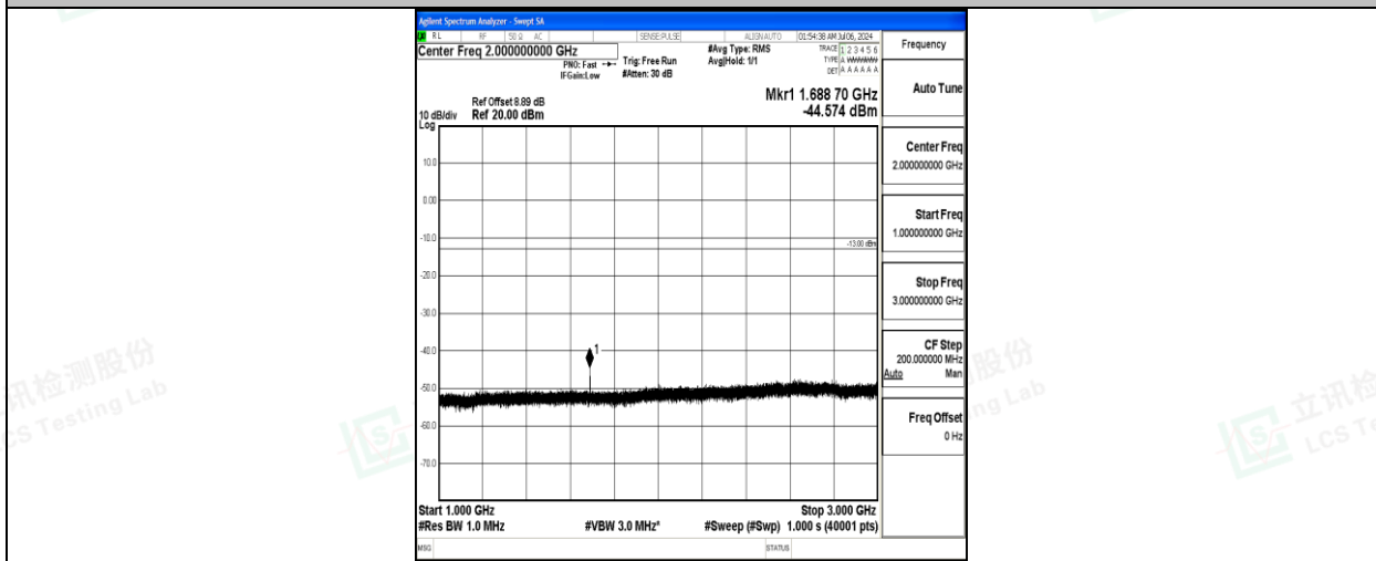
Band5_5MHz_16QAM_20625_1RB#0_1000~3000_1000~3000
