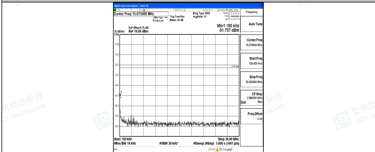
Band5_10MHz_16QAM_20525_1RB#0_0.15~30_0.15~30
