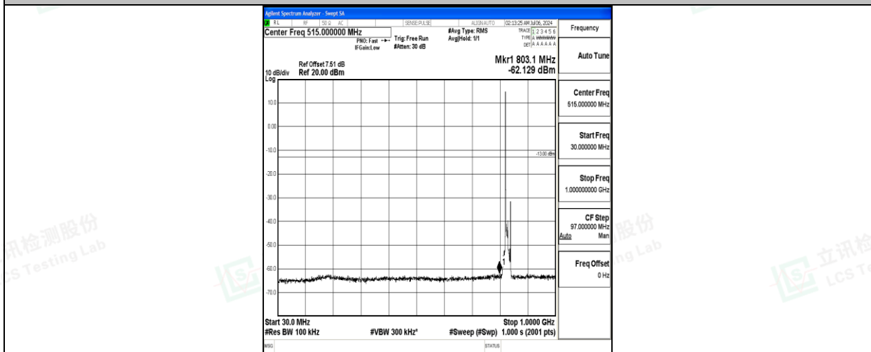
Band5_10MHz_16QAM_20450_1RB#0_30~1000_30~1000
