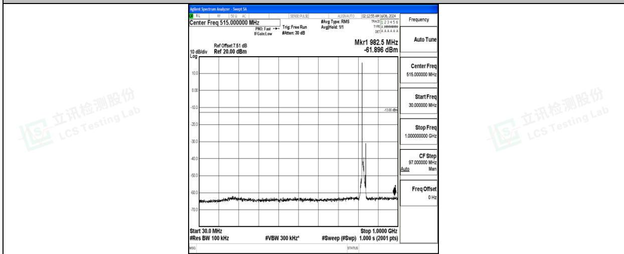
Band5_10MHz_QPSK_20450_1RB#0_30~1000_30~1000
