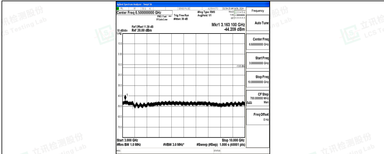
Band5_5MHz_QPSK_20625_1RB#0_3000~10000_3000~10000
