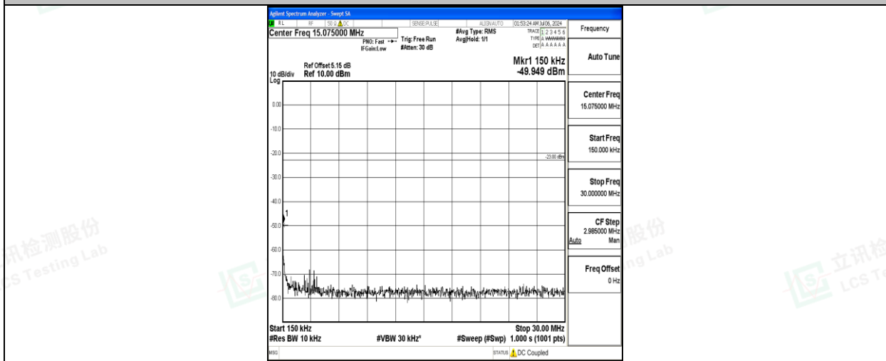
Band5_5MHz_16QAM_20525_1RB#0_0.15~30_0.15~30
