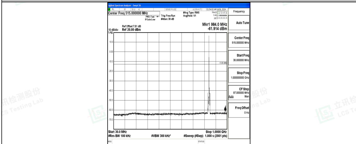
Band5_5MHz_QPSK_20625_1RB#0_30~1000_30~1000
