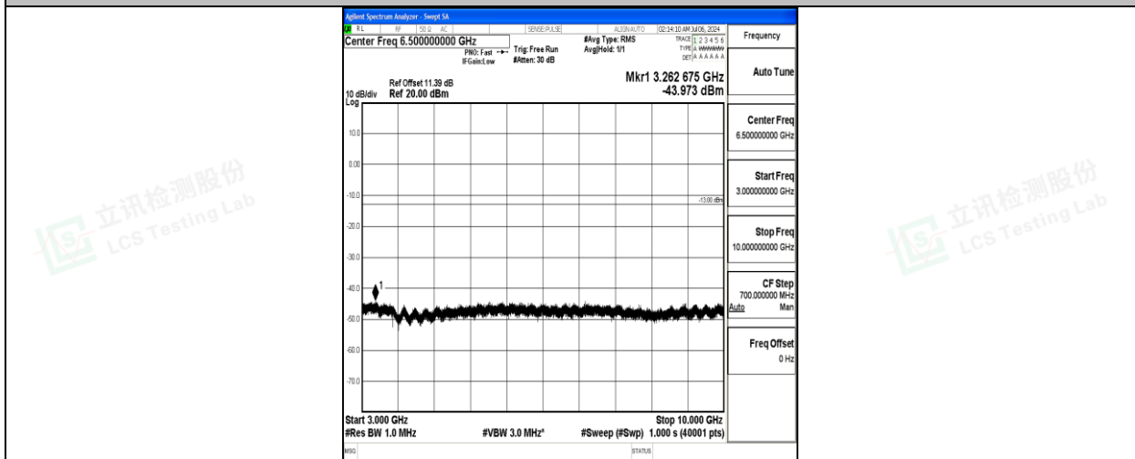
Band5_10MHz_QPSK_20525_1RB#0_3000~10000_3000~10000
