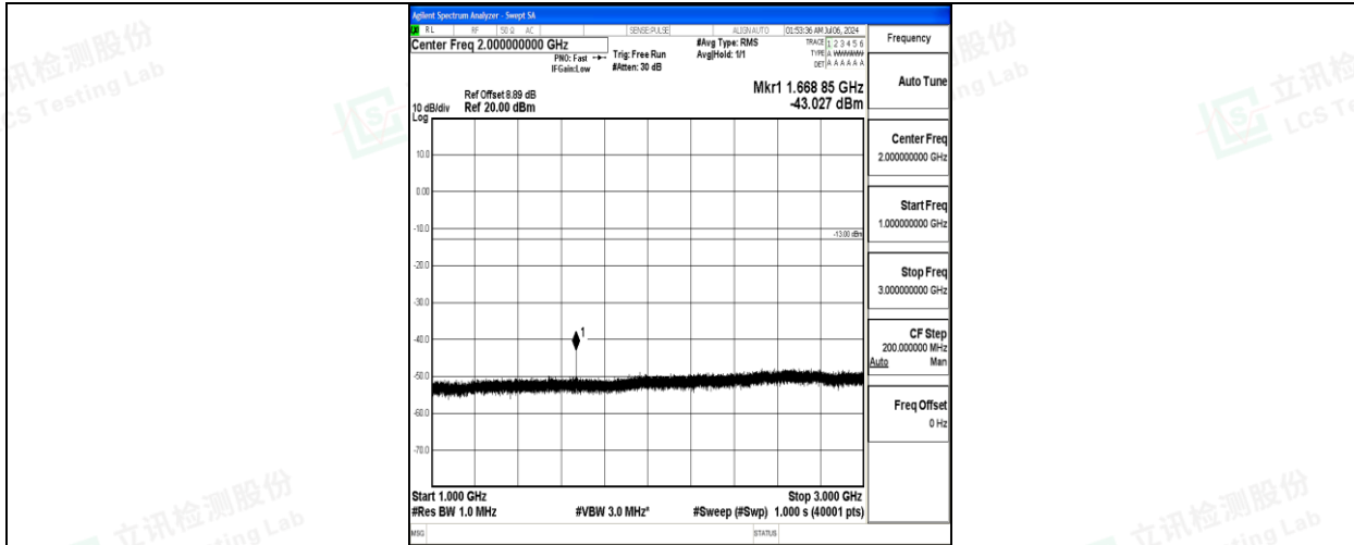
Band5_5MHz_16QAM_20525_1RB#0_1000~3000_1000~3000
