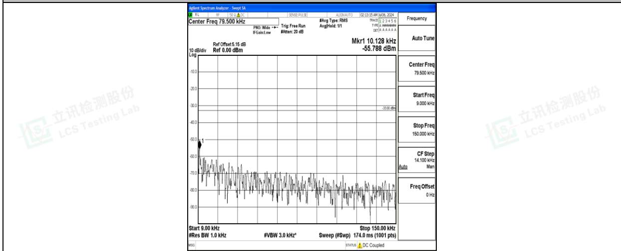
Band5_10MHz_16QAM_20450_1RB#0_0.009~0.15_0.009~0.15
