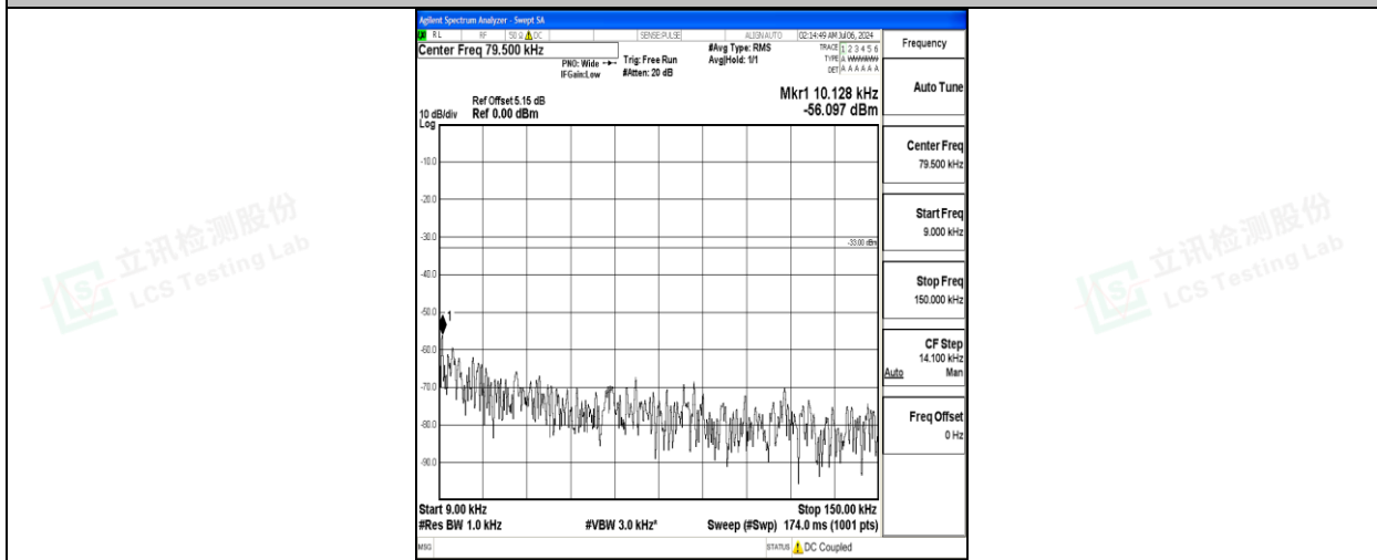
Band5_10MHz_QPSK_20600_1RB#0_0.009~0.15_0.009~0.15
