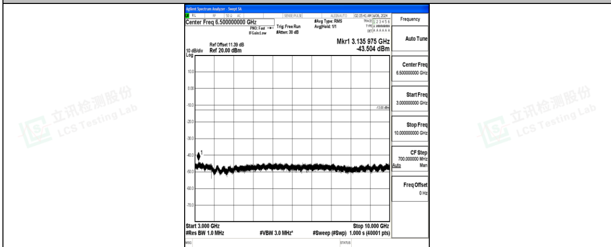
Band5_10MHz_16QAM_20600_1RB#0_3000~10000_3000~10000
