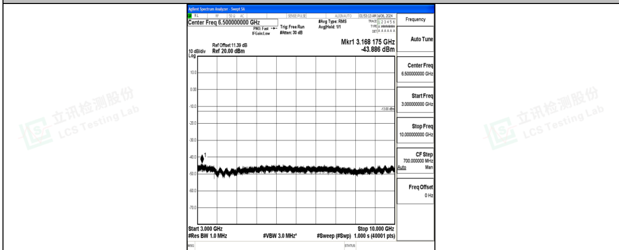
Band5_5MHz_QPSK_20525_1RB#0_3000~10000_3000~10000
