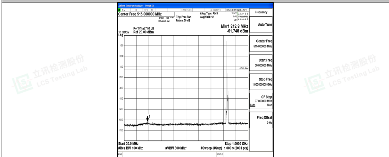
Band5_5MHz_16QAM_20525_1RB#0_30~1000_30~1000
