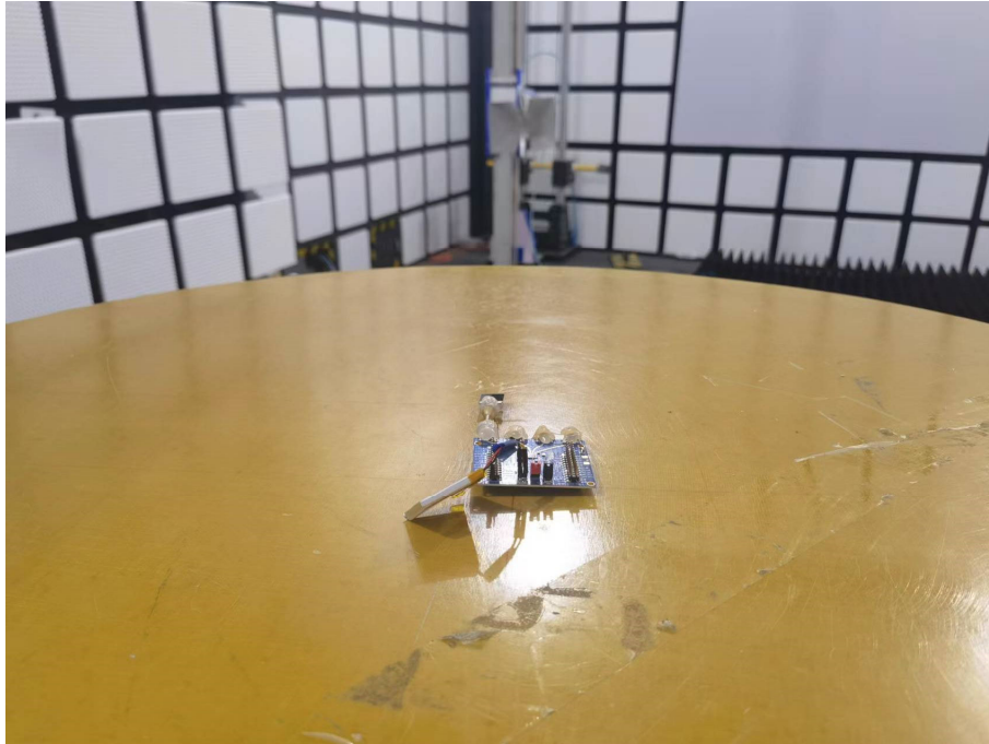
Antenna Mode 1 Lay down
