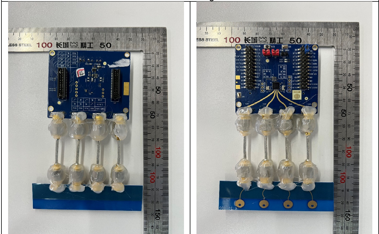
Antenna Mode 2: Array antenna
