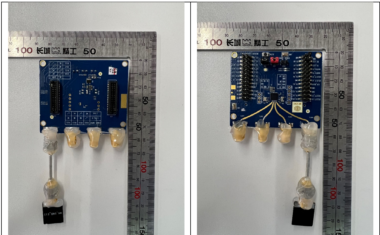
Antenna Mode 1: Single antenna
