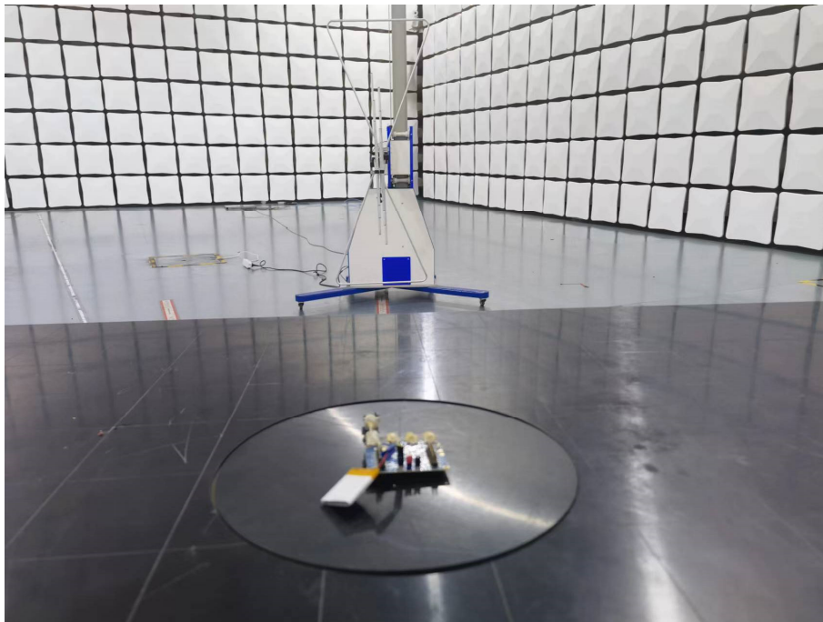
30MHz-1GHz Vertical
