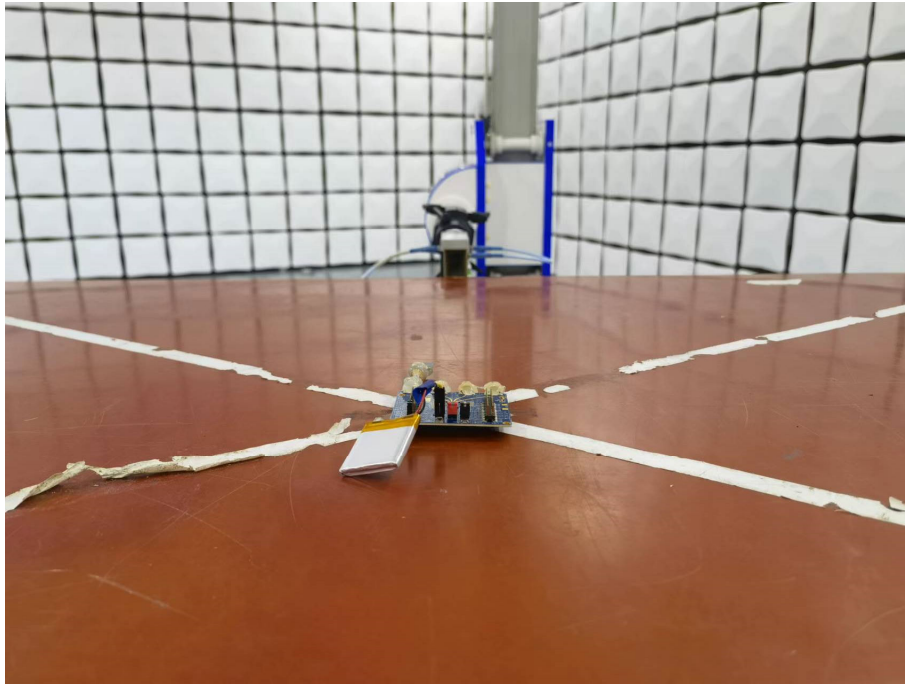
18GHz-40GHz Vertical
