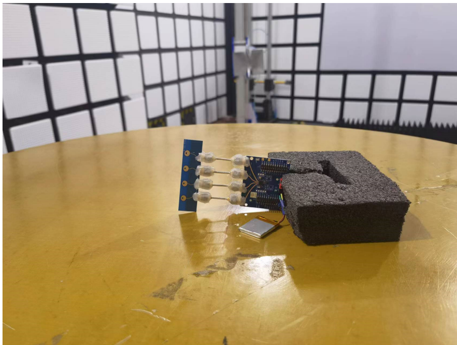
Antenna Mode 2 Side-standing
