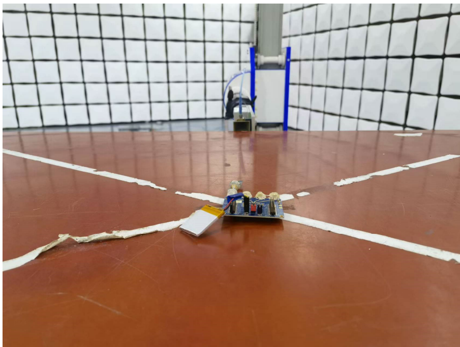
18GHz-40GHz Horizontal
