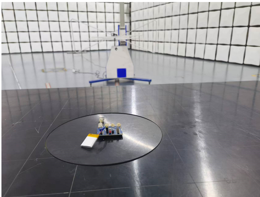
30MHz-1GHz Horizontal
