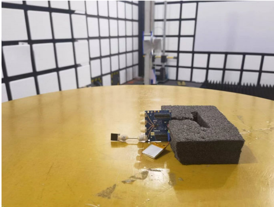
Antenna Mode 1 Side-standing
