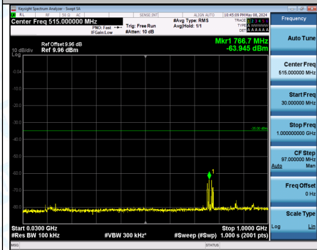
Band7_20MHz_QPSK_21350_1RB#0_20000~27000_20000~27000
