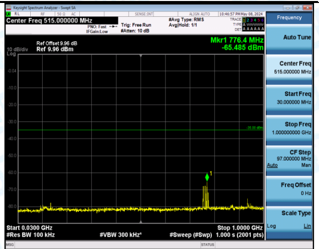
Band7_20MHz_QPSK_21350_1RB#99_20000~27000_20000~27000
