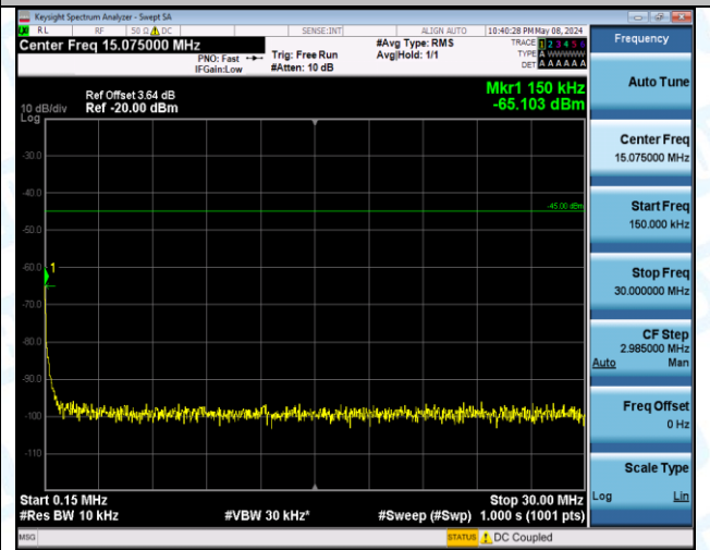
Band7_20MHz_16QAM_20850_1RB#99_1000~20000_1000~20000
