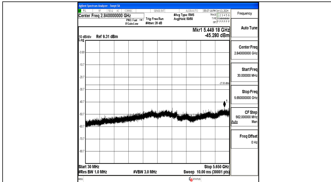
11AC80MIMO-Ant2-5775-30~5650-PASS
