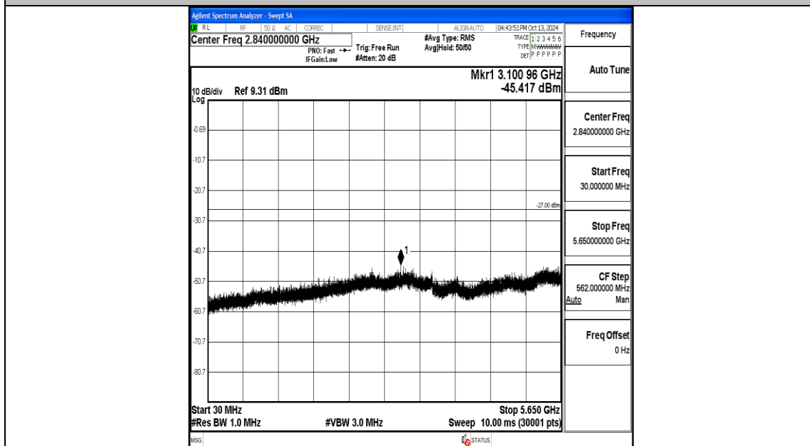
11AC20MIMO-Ant2-5745-30~5650-PASS
