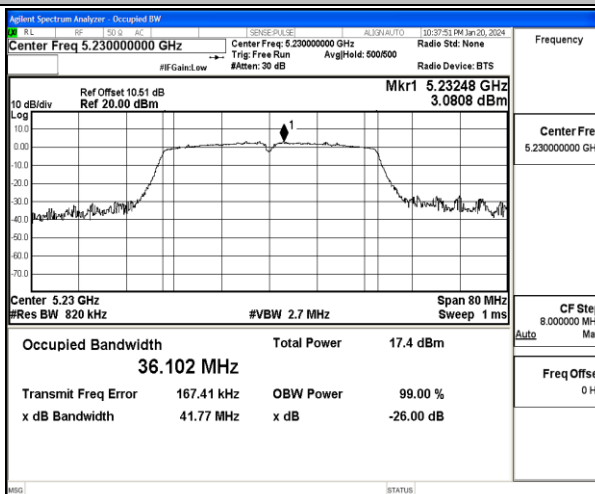
11AC40MIMO-Ant2-5230
