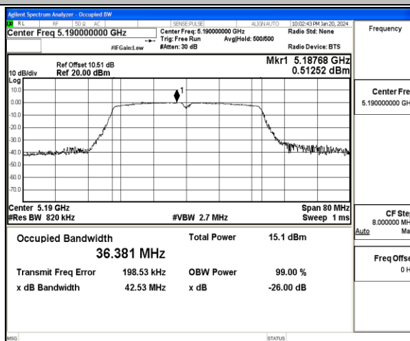
11N40MIMO-Ant2-5190
