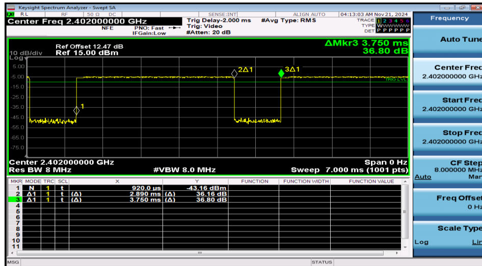
NTNV-3DH5-Ant1-2402
