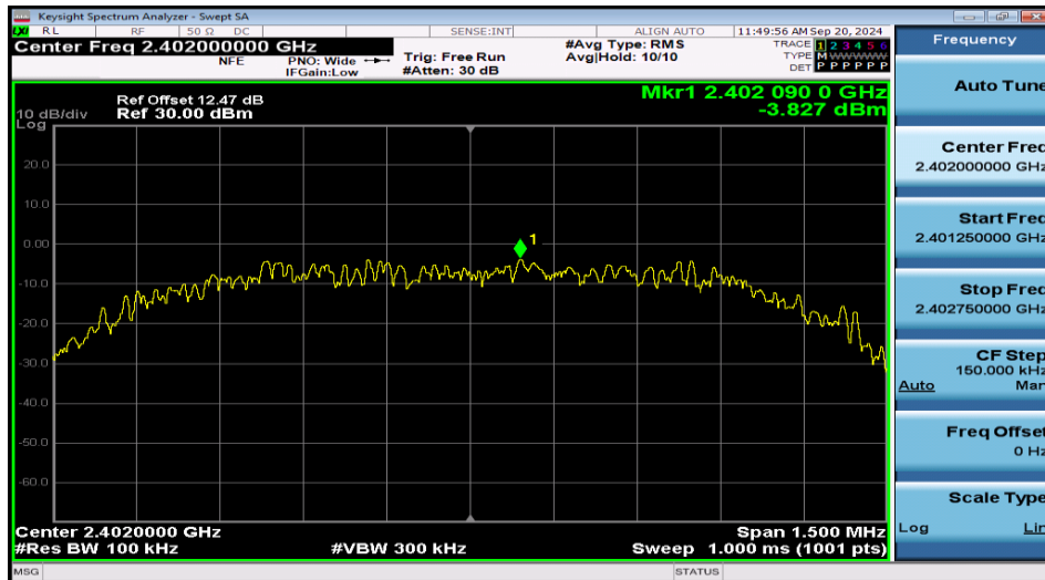
3DH5-Ant1-2402-0~Reference-PASS
