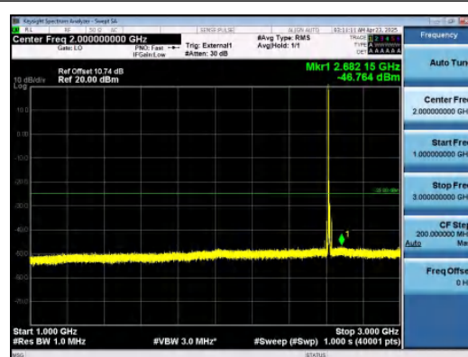
Band38-10MHz-QPSK-38200-1RB#0-1000~300 0-PASS
