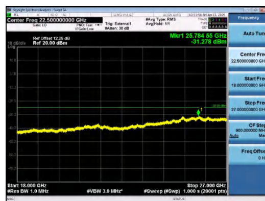
Band38-10MHz-QPSK-38200-1RB#0-18000~27 000-PASS
