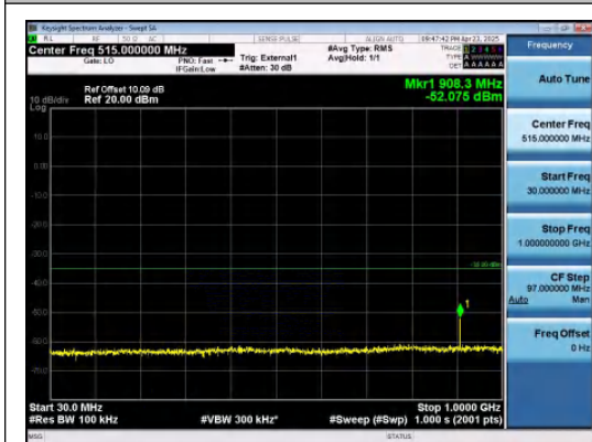
Band38-20MHz-QPSK-38150-1RB#99-30~1000-PASS
