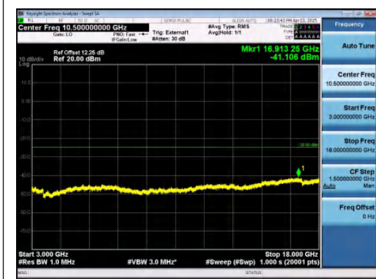
Band38-15MHz-QPSK-38175-75RB#0-3000~18000-PASS
