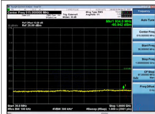
Band38-15MHz-QPSK-38000-1RB#0-30~1000-P ASS
