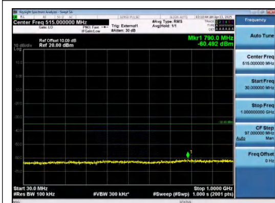
Band38-10MHz-QPSK-38200-1RB#0-30~1000-P ASS
