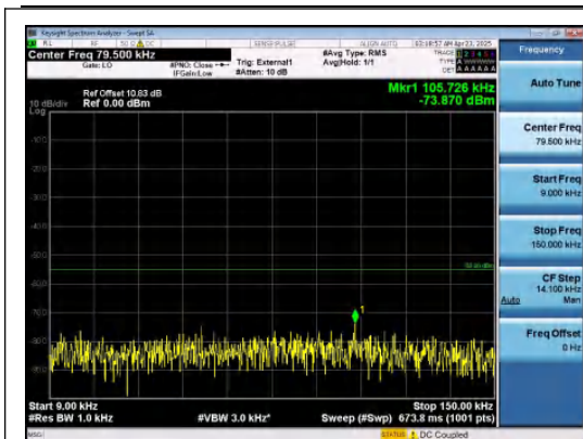
Band38-10MHz-QPSK-38200-50RB#0-0.009~0.15-PASS
