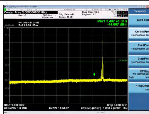
Band38-15MHz-16QAM-37825-1RB#0-1000~3000-PASS
