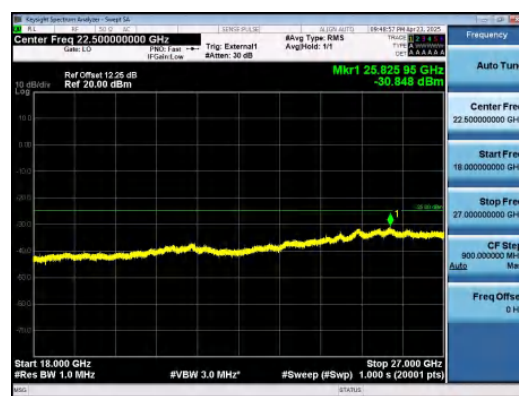
Band38-20MHz-QPSK-38150-1RB#99-18000~27000-PASS
