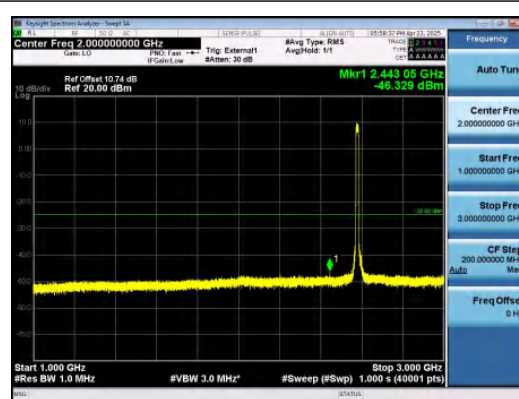
Band38-15MHz-16QAM-37825-75RB#0-1000~3-000-PASS
