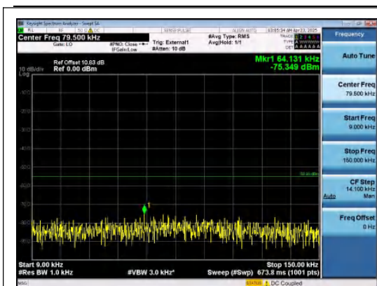
Band38-10MHz-QPSK-38000-50RB#0-0.009~0.15-PASS
