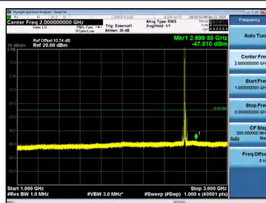
Band38-15MHz-QPSK-38000-1RB#0-1000~300 0-PASS
