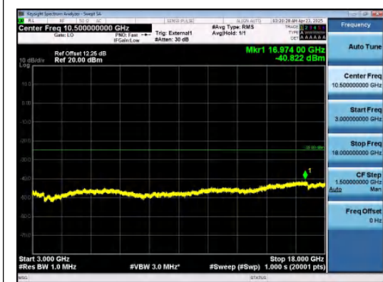
Band38-10MHz-QPSK-38200-50RB#0-3000~18000-PASS
