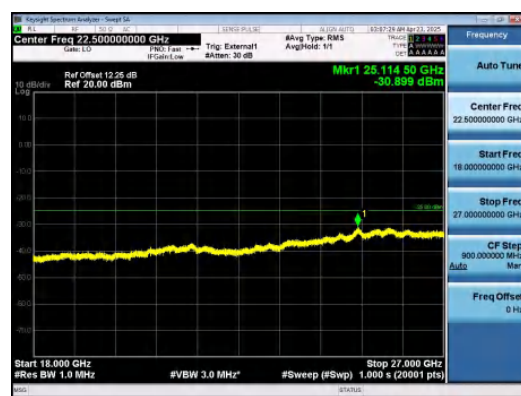
Band38-10MHz-QPSK-38000-50RB#0-18000~27000-PASS
