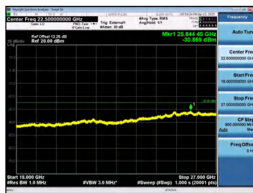
Band38-15MHz-16QAM-37825-75RB#0-18000~27000-PASS
