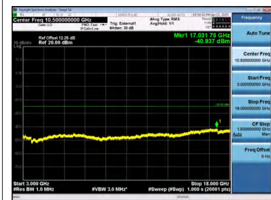
Band38-15MHz-16QAM-37825-1RB#0-3000~18000-PASS
