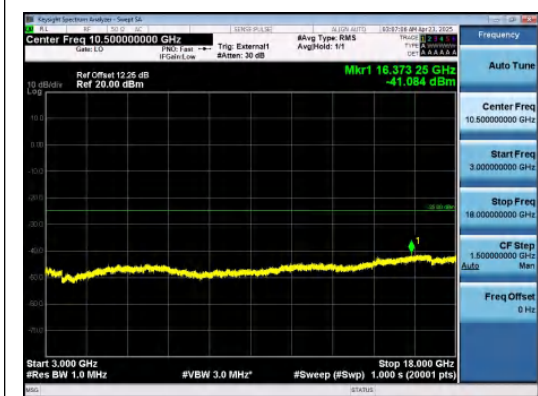
Band38-10MHz-QPSK-38000-50RB#0-3000~18000-PASS
