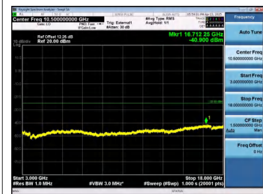
Band38-15MHz-16QAM-37825-75RB#0-3000~18000-PASS
