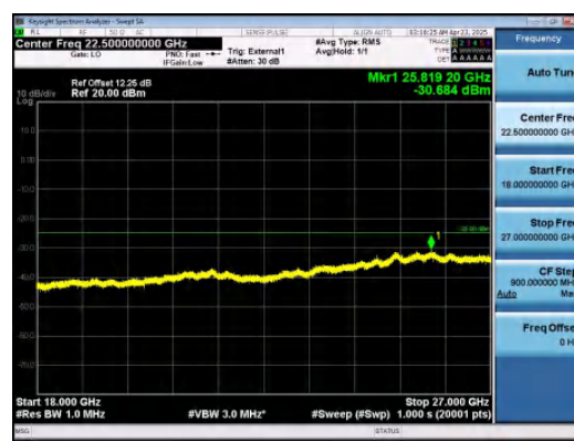
Band38-10MHz-QPSK-38200-1RB#49-18000~27000-PASS
