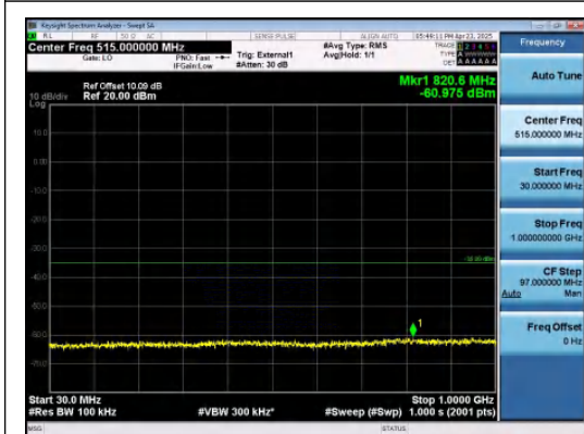
Band38-15MHz-16QAM-37825-1RB#0-30~1000-PASS
