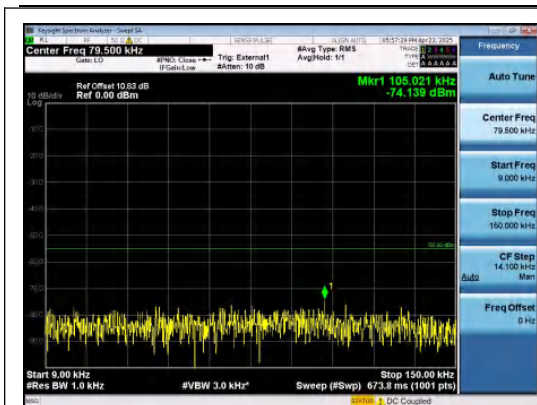
Band38-15MHz-16QAM-37825-75RB#0-0.009~0.15-PASS
