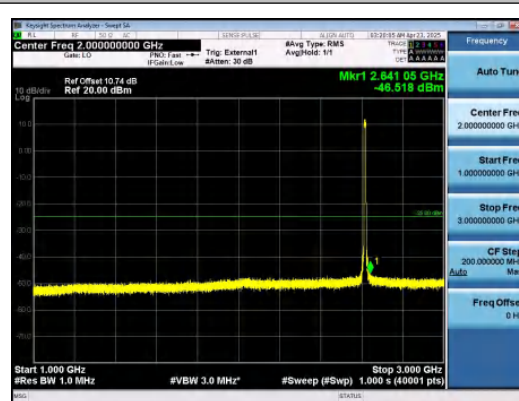
Band38-10MHz-QPSK-38200-50RB#0-1000~3000-PASS
