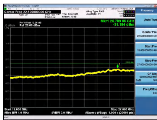
Band38-15MHz-QPSK-38175-75RB#0-18000~27000-PASS
