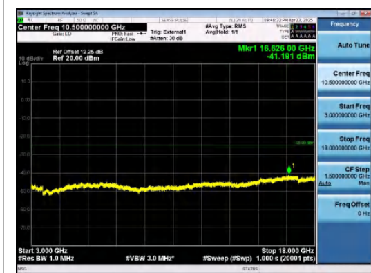
Band38-20MHz-QPSK-38150-1RB#99-3000~18000-PASS
