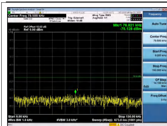
Band38-10MHz-QPSK-38200-1RB#0-0.009~0.1 5-PASS
