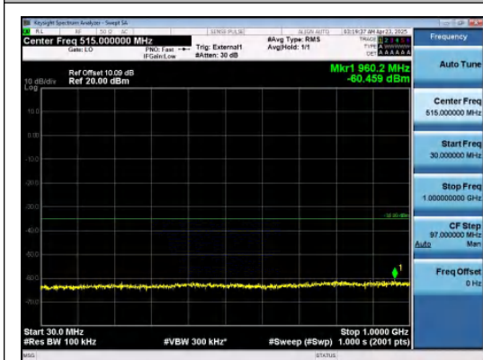
Band38-10MHz-QPSK-38200-50RB#0-30~1000-PASS
