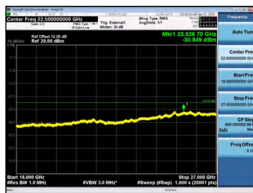
Band38-10MHz-QPSK-38200-50RB#0-18000~27000-PASS
