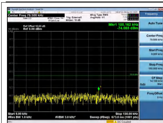
Band38-20MHz-QPSK-38150-1RB#99-0.009~0.15-PASS
