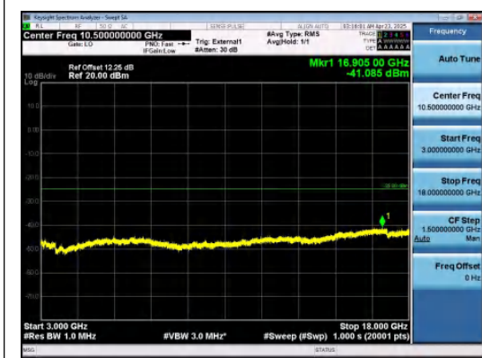
Band38-10MHz-QPSK-38200-1RB#49-3000~18000-PASS
