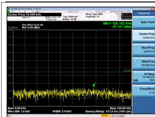
Band38-15MHz-QPSK-38000-1RB#0-0.009~0.1 5-PASS
