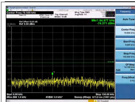
Band38-15MHz-QPSK-38175-75RB#0-0.009~0.15-PASS
