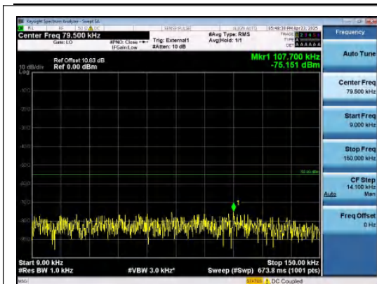
Band38-15MHz-16QAM-37825-1RB#0-0.009~0.15-PASS
