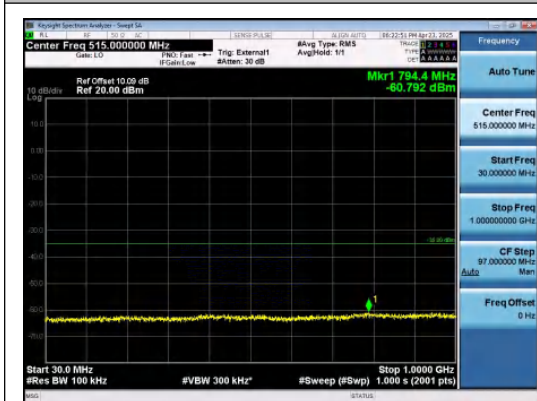
Band38-15MHz-QPSK-38175-75RB#0-30~1000-PASS
