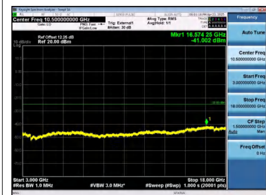
Band38-15MHz-QPSK-38000-1RB#0-3000~180 00-PASS
