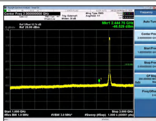
Band38-15MHz-QPSK-38175-75RB#0-1000~3000-PASS
