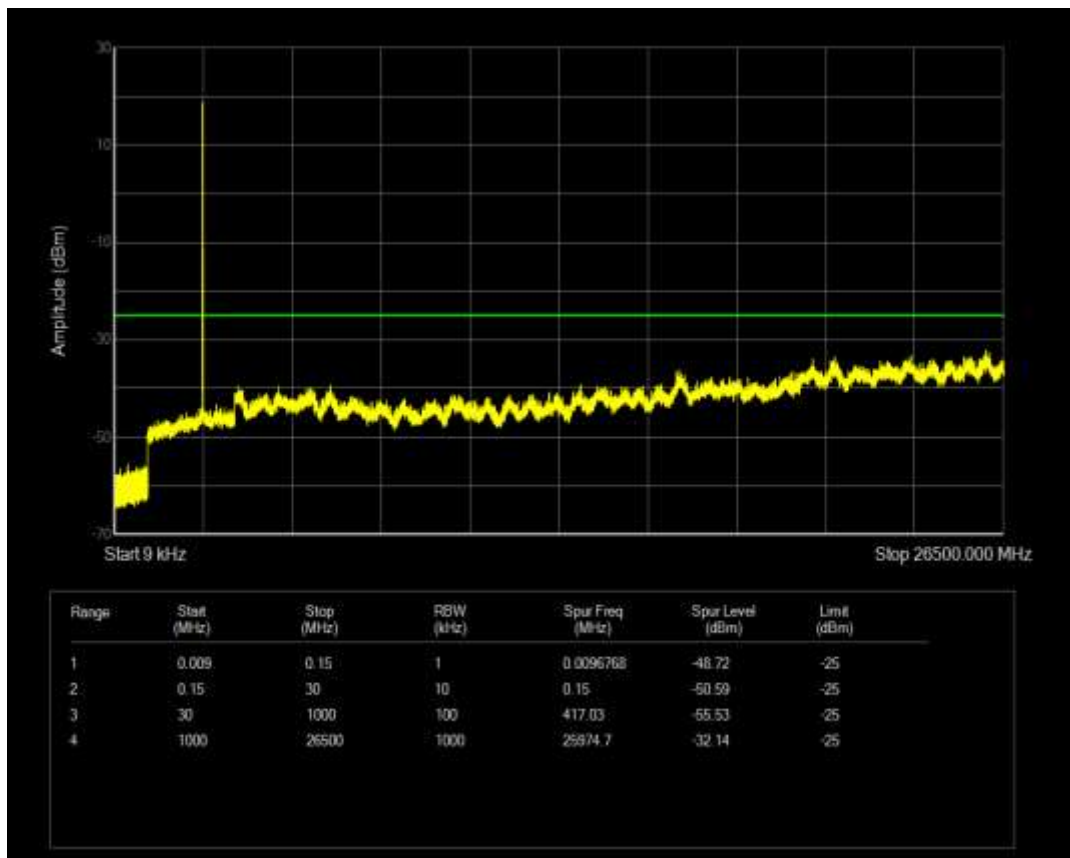
Band41 16QAM BW=10MHz Channel=41140 RB Size=50 Position=#0
