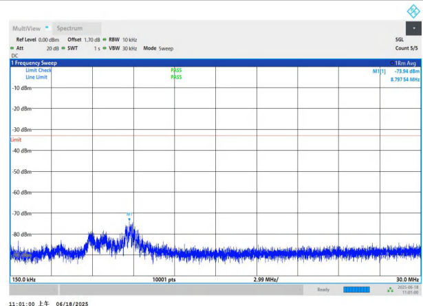
NTNV-n77(3700-3980)-PC3-30-15-H-DFT-BPSK-Edge_1RB_Left 0.15-30-PASS
