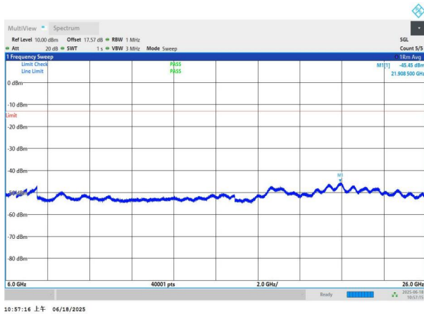
NTNV-n77(3700-3980)-PC3-30-15-L-DFT-QPSK-Edge_1RB_Left- 6000-26000-PASS
