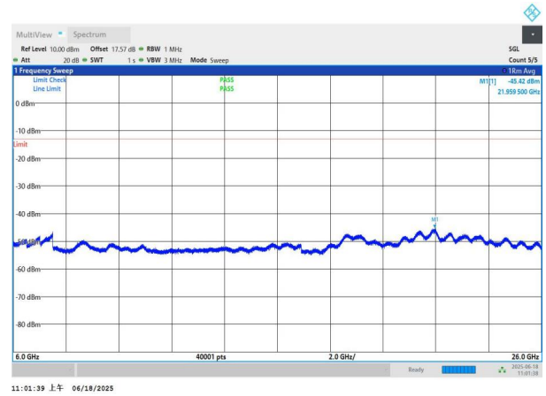
NTNV-n77(3700-3980)-PC3-30-15-H-DFT-BPSK-Edge_1RB_Left 6000-26000-PASS
