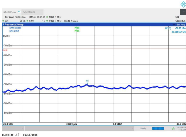
NTNV-n77(3700-3980)-PC3-30-20-M-DFT-BPSK-Edge_1RB_Left -26000-40000-PASS
