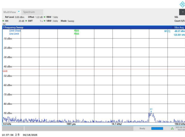
NTNV-n77(3700-3980)-PC3-30-15-M-DFT-BPSK-Edge_1RB_Left -0.009-0.15-PASS
