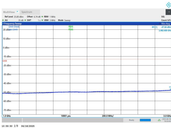
NTNV-n77(3700-3980)-PC3-30-15-M-DFT-QPSK-Edge_1RB_Left -1000-3000-PASS
