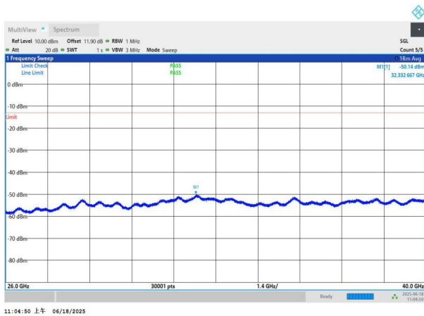
NTNV-n77(3700-3980)-PC3-30-20-L-DFT-BPSK-Edge_1RB_Left- 26000-40000-PASS
