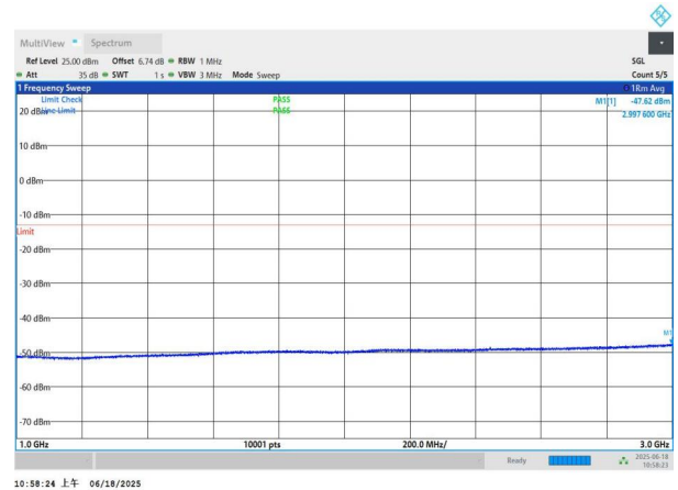
NTNV-n77(3700-3980)-PC3-30-15-M-DFT-BPSK-Edge_1RB_Left -1000-3000-PASS
