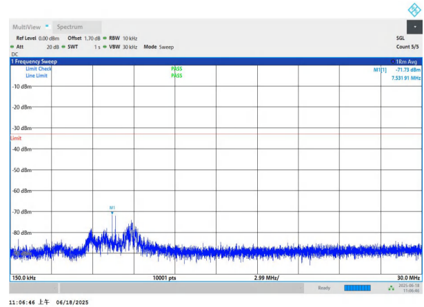
NTNV-n77(3700-3980)-PC3-30-20-M-DFT-BPSK-Edge_1RB_Left -0.15-30-PASS
