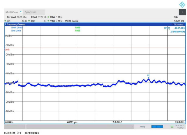
NTNV-n77(3700-3980)-PC3-30-20-M-DFT-BPSK-Edge_1RB_Left -6000-26000-PASS
