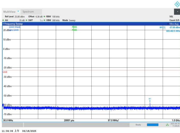
NTNV-n77(3700-3980)-PC3-30-20-L-DFT-BPSK-Edge_1RB_Left- 30-1000-PASS
