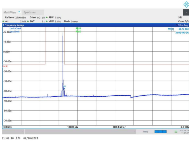
NTNV-n77(3700-3980)-PC3-30-15-H-DFT-BPSK-Edge_1RB_Left -3000-6000-PASS
