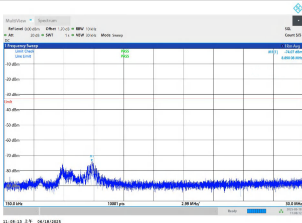
NTNV-n77(3700-3980)-PC3-30-20-M-DFT-QPSK-Edge_1RB_Left -0.15-30-PASS
