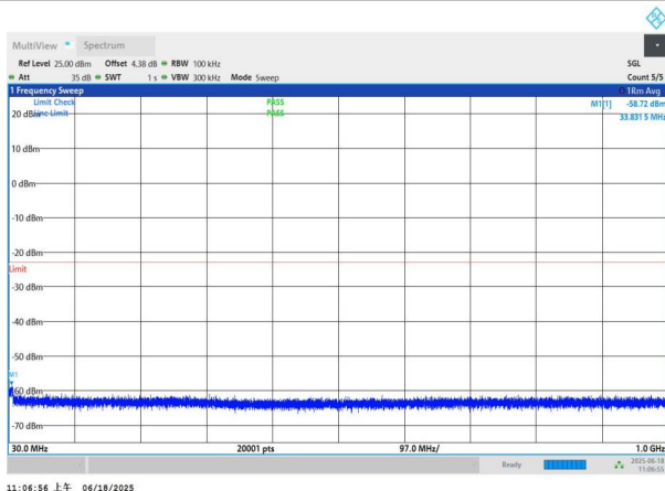
NTNV-n77(3700-3980)-PC3-30-20-M-DFT-BPSK-Edge_1RB_Left -30-1000-PASS
