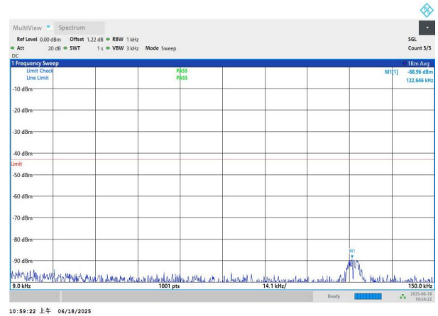
NTNV-n77(3700-3980)-PC3-30-15-M-DFT-QPSK-Edge_1RB_Left -0.009-0.15-PASS
