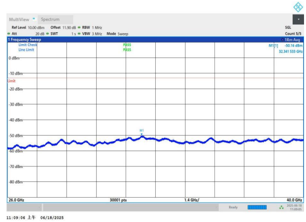
NTNV-n77(3700-3980)-PC3-30-20-M-DFT-QPSK-Edge_1RB_Left -26000-40000-PASS
