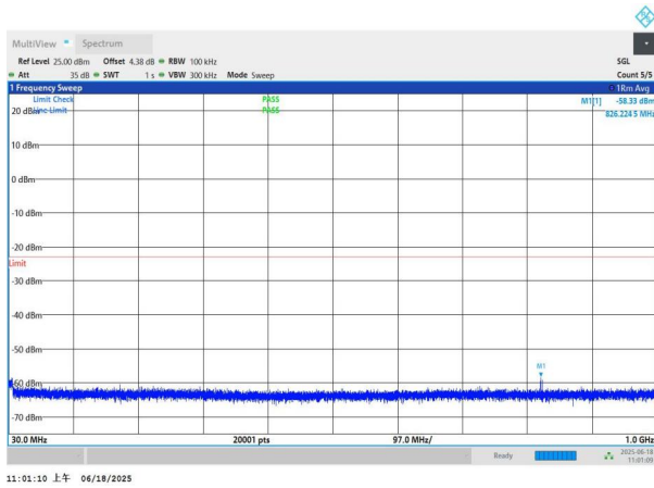
NTNV-n77(3700-3980)-PC3-30-15-H-DFT-BPSK-Edge_1RB_Left -30-1000-PASS
