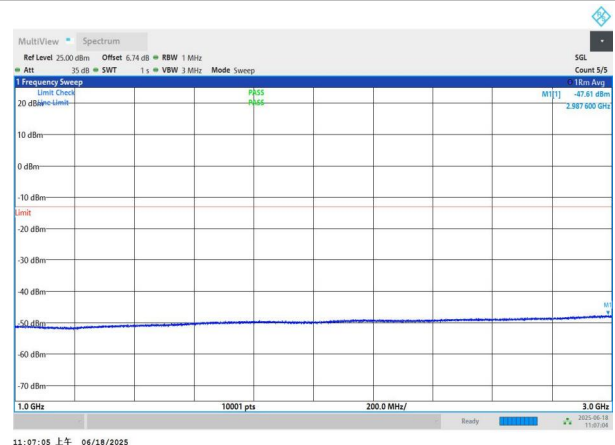
NTNV-n77(3700-3980)-PC3-30-20-M-DFT-BPSK-Edge_1RB_Left -1000-3000-PASS
