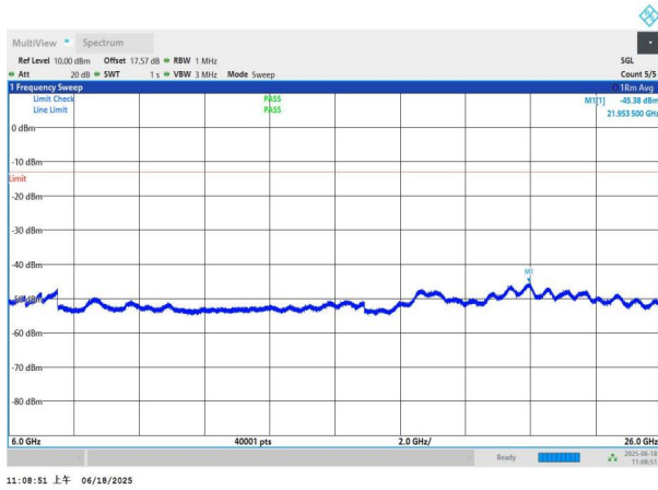
NTNV-n77(3700-3980)-PC3-30-20-M-DFT-QPSK-Edge_1RB_Left -6000-26000-PASS
