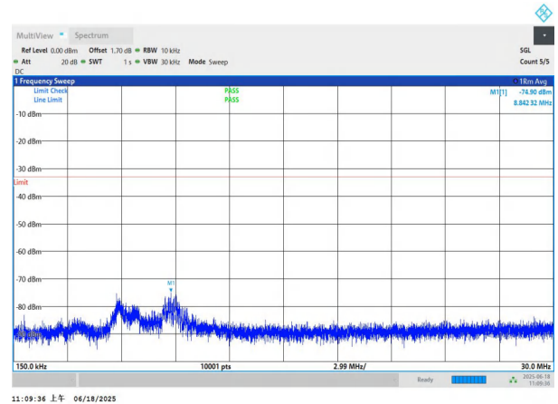
NTNV-n77(3700-3980)-PC3-30-20-H-DFT-BPSK-Edge_1RB_Left 0.15-30-PASS
