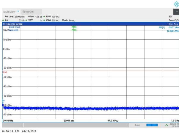
NTNV-n77(3700-3980)-PC3-30-15-M-DFT-BPSK-Edge_1RB_Left -30-1000-PASS
