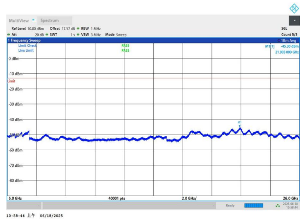
NTNV-n77(3700-3980)-PC3-30-15-M-DFT-BPSK-Edge_1RB_Left -6000-26000-PASS
