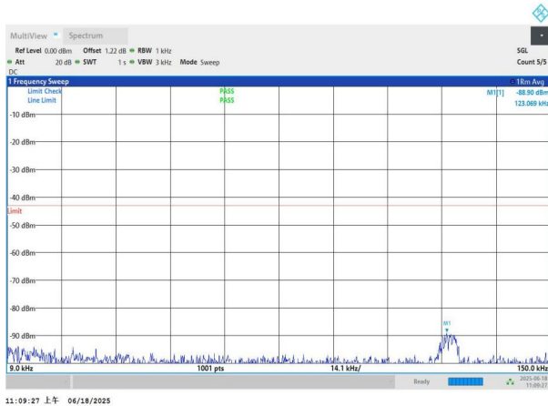
NTNV-n77(3700-3980)-PC3-30-20-H-DFT-BPSK-Edge_1RB_Left -0.009-0.15-PASS
