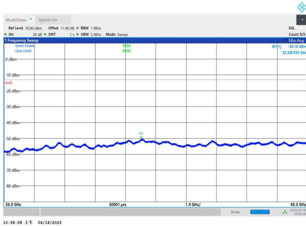
NTNV-n77(3700-3980)-PC3-30-15-M-DFT-BPSK-Edge_1RB_Left -26000-40000-PASS
