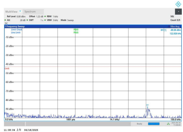
NTNV-n77(3700-3980)-PC3-30-20-M-DFT-QPSK-Edge_1RB_Left -0.009-0.15-PASS
