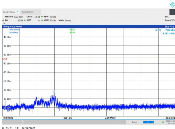
NTNV-n77(3700-3980)-PC3-30-15-M-DFT-QPSK-Edge_1RB_Left -0.15-30-PASS
