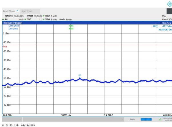
NTNV-n77(3700-3980)-PC3-30-15-H-DFT-BPSK-Edge_1RB_Left -26000-40000-PASS
