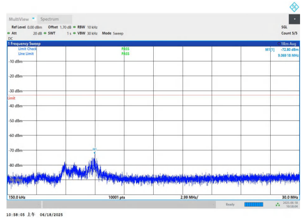
NTNV-n77(3700-3980)-PC3-30-15-M-DFT-BPSK-Edge_1RB_Left -0.15-30-PASS
