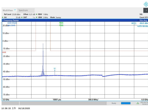
NTNV-n77(3700-3980)-PC3-30-15-M-DFT-BPSK-Edge_1RB_Left -3000-6000-PASS
