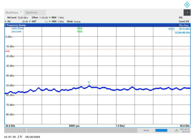
NTNV-n77(3700-3980)-PC3-30-15-L-DFT-QPSK-Edge_1RB_Left- 26000-40000-PASS
