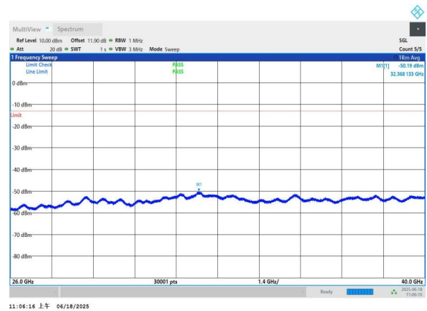
NTNV-n77(3700-3980)-PC3-30-20-L-DFT-QPSK-Edge_1RB_Left- 26000-40000-PASS
