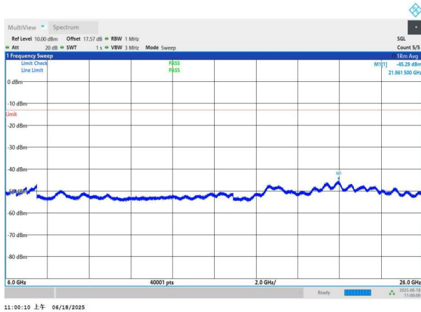
NTNV-n77(3700-3980)-PC3-30-15-M-DFT-QPSK-Edge_1RB_Left -6000-26000-PASS
