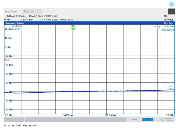
NTNV-n77(3700-3980)-PC3-30-15-H-DFT-BPSK-Edge_1RB_Left 1000-3000-PASS
