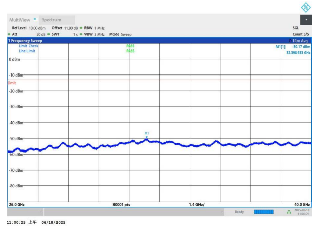
NTNV-n77(3700-3980)-PC3-30-15-M-DFT-QPSK-Edge_1RB_Left -26000-40000-PASS
