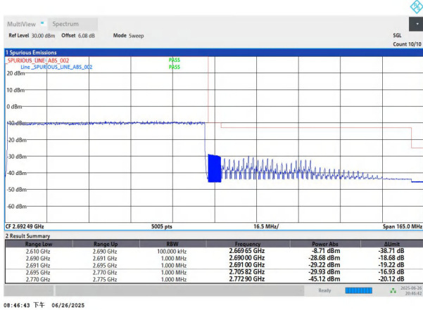
NTNV-n41-PC3-30-80-H-DFT-BPSK-Outer_Full-PASS
