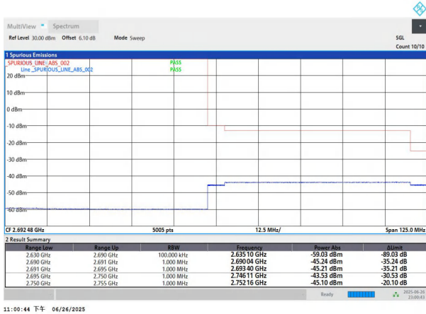
NTNV-n41-PC3-30-60-H-DFT-BPSK-Outer_Full-PASS
