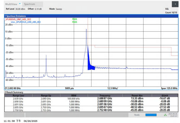
NTNV-n41-PC3-30-60-H-DFT-BPSK-Edge_1RB_Right-PASS
