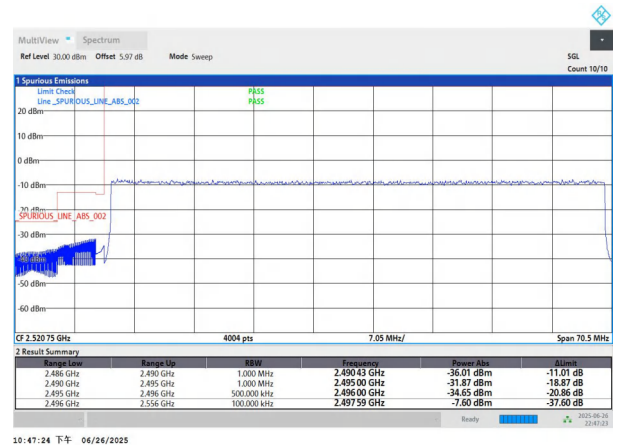
NTNV-n41-PC3-30-60-L-DFT-BPSK-Outer_Full-PASS
