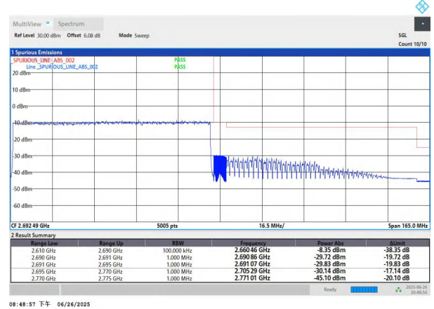
NTNV-n41-PC3-30-80-H-DFT-QPSK-Outer_Full-PASS
