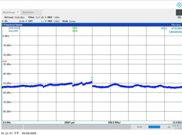
NTNV-n7-PC3-15-20-H-DFT-QPSK-Edge_1RB_Left-3000-12000-PASS
