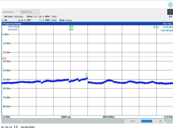
NTNV-n7-PC3-15-10-H-DFT-QPSK-Edge_1RB_Left-3000-12000-
