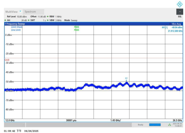
NTNV-n7-PC3-15-20-L-DFT-QPSK-Edge_1RB_Left-12000-26500
