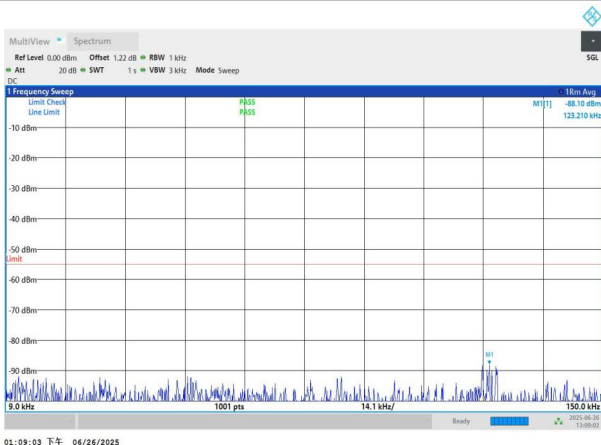
NTNV-n7-PC3-15-20-M-DFT-BPSK-Edge_1RB_Left-0.009-0.15-P
