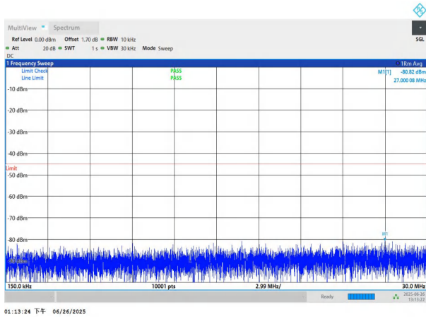
NTNV-n7-PC3-15-25-M-DFT-QPSK-Edge_1RB_Left-0.15-30-PAS S
