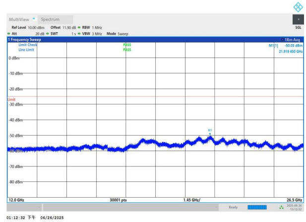
NTNV-n7-PC3-15-25-L-DFT-QPSK-Edge_1RB_Left-12000-26500-PASS
