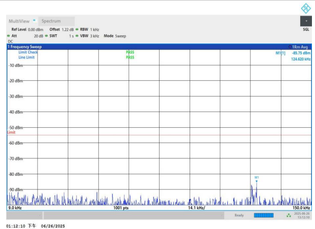
NTNV-n7-PC3-15-25-L-DFT-QPSK-Edge_1RB_Left-0.009-0.15-P ASS
