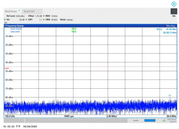
NTNV-n7-PC3-15-10-H-DFT-BPSK-Edge_1RB_Left-0.15-30-PAS S
