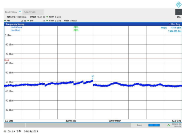
NTNV-n7-PC3-15-20-M-DFT-BPSK-Edge_1RB_Left-3000-12000-PASS PASS
