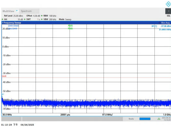
NTNV-n7-PC3-15-20-H-DFT-BPSK-Edge_1RB_Left-30-1000-PAS S
