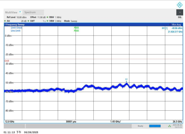
NTNV-n7-PC3-15-20-H-DFT-QPSK-Edge_1RB_Left-12000-26500
