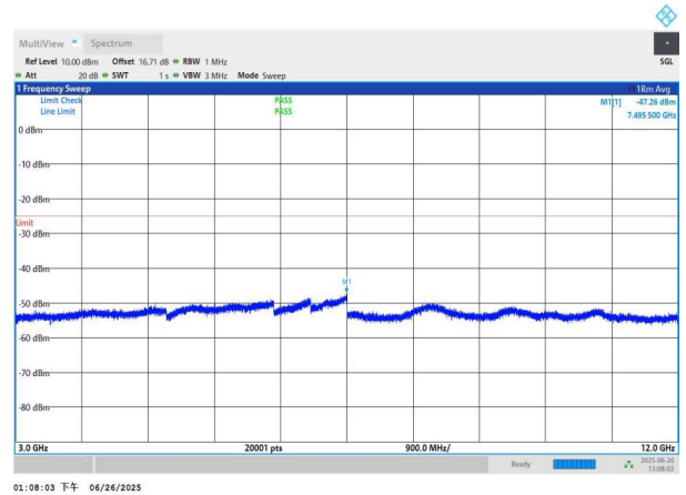
NTNV-n7-PC3-15-20-L-DFT-BPSK-Edge_1RB_Left-3000-12000-PASS PASS
