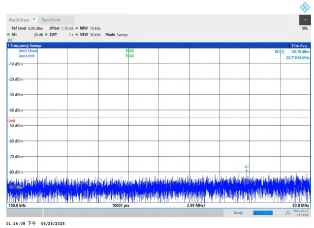
NTNV-n7-PC3-15-25-H-DFT-BPSK-Edge_1RB_Left-0.15-30-PASS
