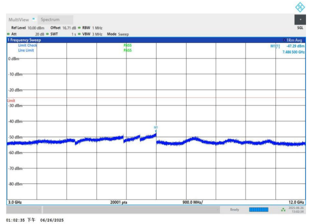
NTNV-n7-PC3-15-10-H-DFT-BPSK-Edge_1RB_Left-3000-12000- PASS
