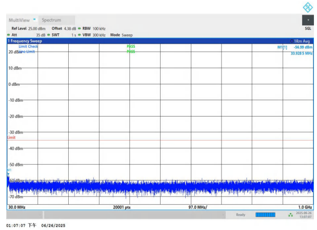
NTNV-n7-PC3-15-15-H-DFT-QPSK-Edge_1RB_Left-30-1000-PAS S
