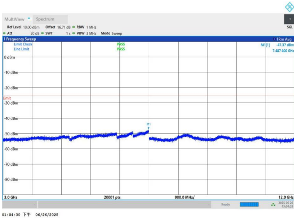
NTNV-n7-PC3-15-15-L-DFT-QPSK-Edge_1RB_Left-3000-12000-PASS
