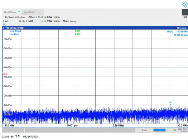
NTNV-n7-PC3-15-20-M-DFT-QPSK-Edge_1RB_Left-0.15-30-PASS S
