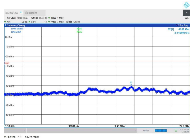
NTNV-n7-PC3-15-10-H-DFT-QPSK-Edge_1RB_Left-12000-26500
