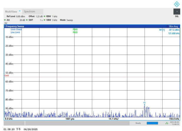
NTNV-n7-PC3-15-20-L-DFT-QPSK-Edge_1RB_Left-0.009-0.15-P ASS
