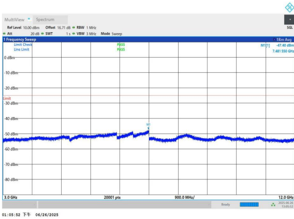
NTNV-n7-PC3-15-15-M-DFT-QPSK-Edge_1RB_Left-3000-12000- PASS
