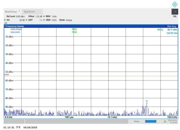
NTNV-n7-PC3-15-20-H-DFT-QPSK-Edge_1RB_Left-0.009-0.15-P ASS
