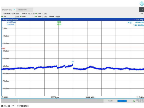
NTNV-n7-PC3-15-10-M-DFT-QPSK-Edge_1RB_Left-3000-12000- PASS
