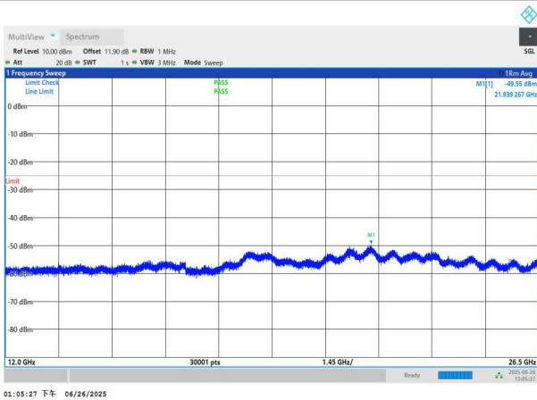
NTNV-n7-PC3-15-15-M-DFT-BPSK-Edge_1RB_Left-12000-2650 0-PASS
