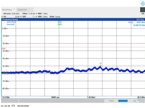
NTNV-n7-PC3-15-25-H-DFT-BPSK-Edge_1RB_Left-12000-26500 -PASS
