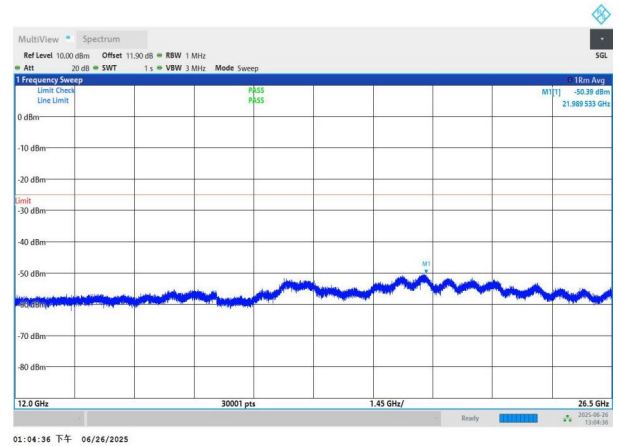
NTNV-n7-PC3-15-15-L-DFT-QPSK-Edge_1RB_Left-12000-26500-PASS
