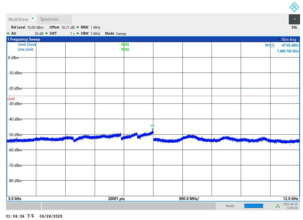
NTNV-n7-PC3-15-15-H-DFT-BPSK-Edge_1RB_Left-3000-12000- PASS
