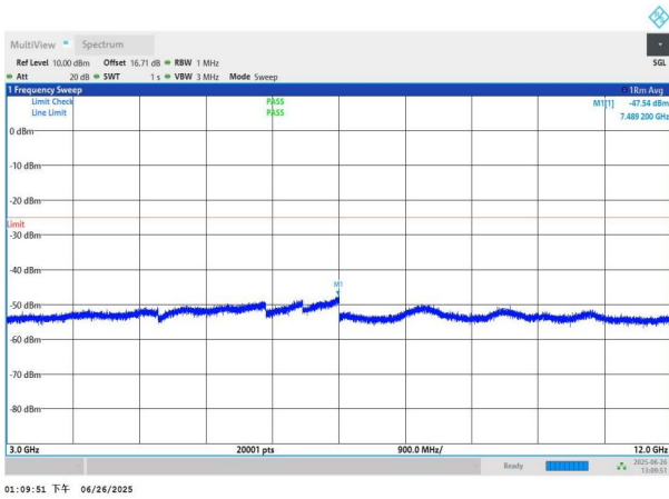
NTNV-n7-PC3-15-20-M-DFT-QPSK-Edge_1RB_Left-3000-12000- PASS
