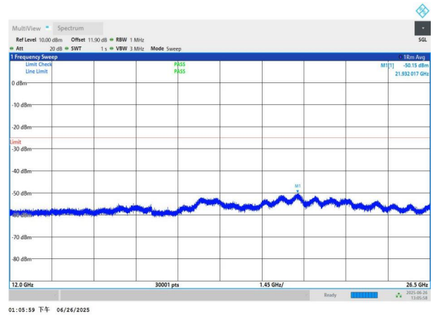
NTNV-n7-PC3-15-15-M-DFT-QPSK-Edge_1RB_Left-12000-2650 0-PASS
