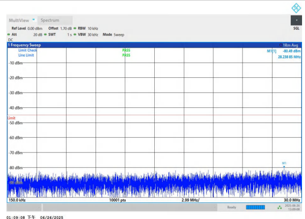
NTNV-n7-PC3-15-20-M-DFT-BPSK-Edge_1RB_Left-0.15-30-PAS
