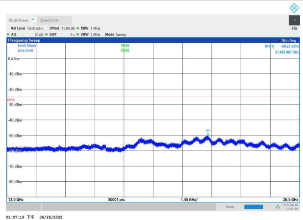
NTNV-n7-PC3-15-15-H-DFT-QPSK-Edge_1RB_Left-12000-26500
