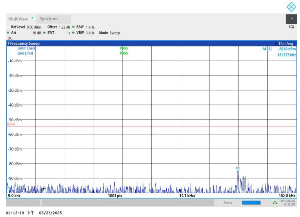
NTNV-n7-PC3-15-25-M-DFT-QPSK-Edge_1RB_Left-0.009-0.15-P ASS
