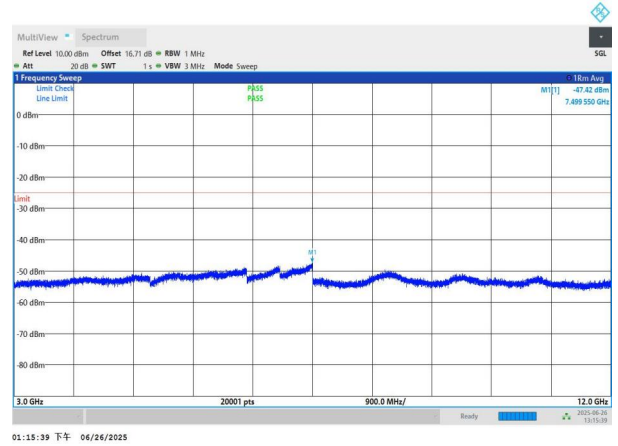
NTNV-n7-PC3-15-30-L-DFT-BPSK-Edge_1RB_Left-3000-12000-PASS PASS
