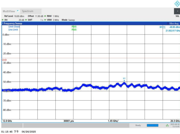
NTNV-n7-PC3-15-30-L-DFT-BPSK-Edge_1RB_Left-12000-26500 -PASS
