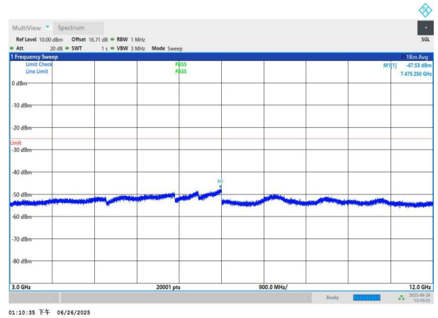
NTNV-n7-PC3-15-20-H-DFT-BPSK-Edge_1RB_Left-3000-12000- PASS
