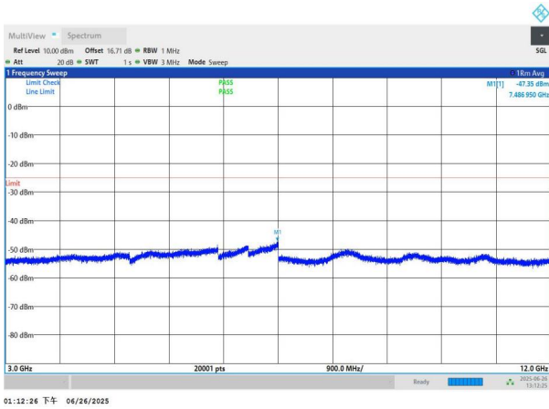
NTNV-n7-PC3-15-25-L-DFT-QPSK-Edge_1RB_Left-3000-12000-PASS
