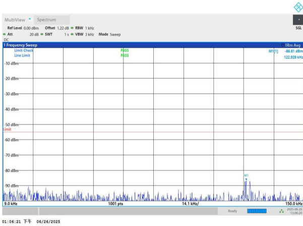
NTNV-n7-PC3-15-15-H-DFT-BPSK-Edge_1RB_Left-0.009-0.15-P ASS
