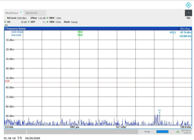
NTNV-n7-PC3-15-15-L-DFT-QPSK-Edge_1RB_Left-0.009-0.15-P ASS
