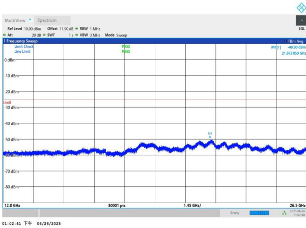
NTNV-n7-PC3-15-10-H-DFT-BPSK-Edge_1RB_Left-12000-26500
