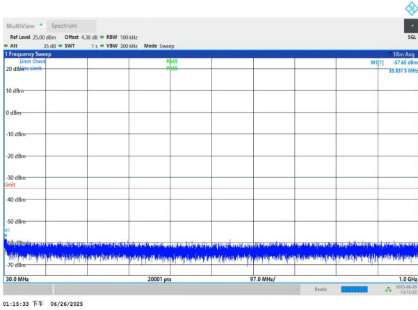
NTNV-n7-PC3-15-30-L-DFT-BPSK-Edge_1RB_Left-30-1000-PAS S
