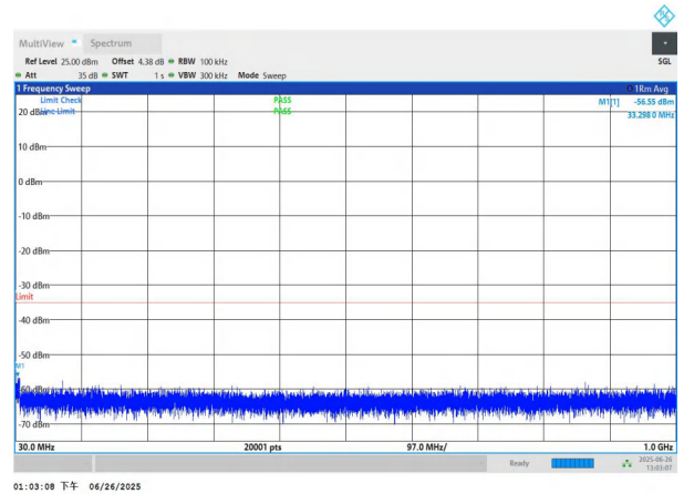
NTNV-n7-PC3-15-10-H-DFT-QPSK-Edge_1RB_Left-30-1000-PAS
