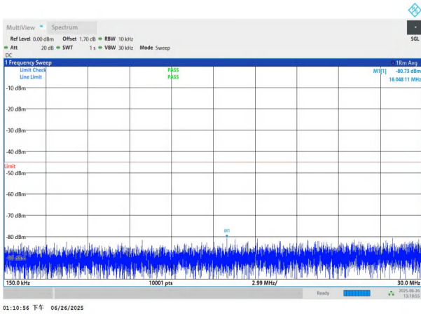
NTNV-n7-PC3-15-20-H-DFT-QPSK-Edge_1RB_Left-0.15-30-PAS S
