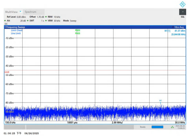
NTNV-n7-PC3-15-15-H-DFT-BPSK-Edge_1RB_Left-0.15-30-PAS S
