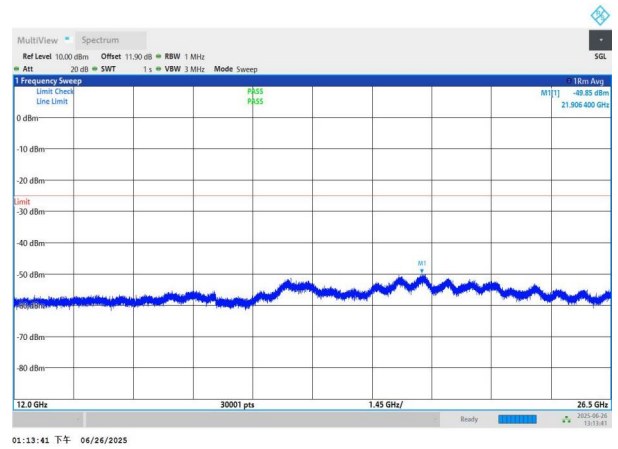
NTNV-n7-PC3-15-25-M-DFT-QPSK-Edge_1RB_Left-12000-2650-0-PASS
