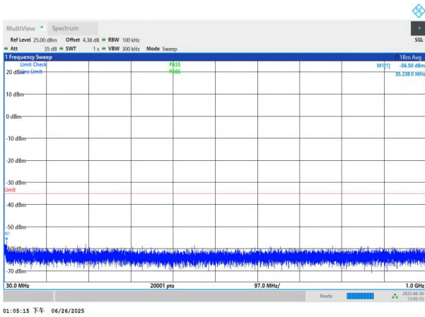
NTNV-n7-PC3-15-15-M-DFT-BPSK-Edge_1RB_Left-30-1000-PA SS
