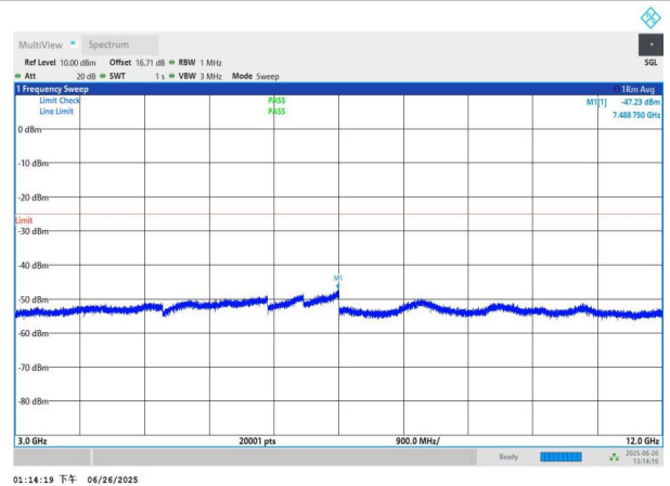
NTNV-n7-PC3-15-25-H-DFT-BPSK-Edge_1RB_Left-3000-12000-PASS
