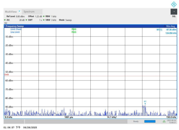
NTNV-n7-PC3-15-15-H-DFT-QPSK-Edge_1RB_Left-0.009-0.15-P ASS
