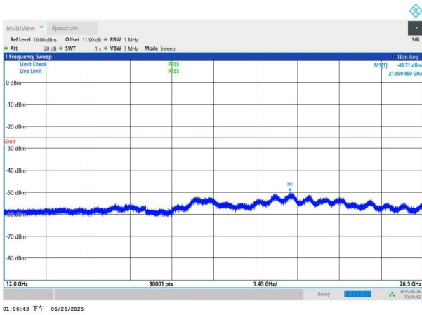
NTNV-n7-PC3-15-15-H-DFT-BPSK-Edge_1RB_Left-12000-26500
