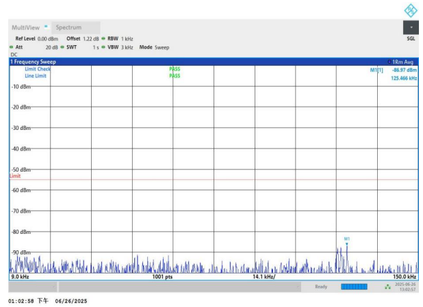
NTNV-n7-PC3-15-10-H-DFT-QPSK-Edge_1RB_Left-0.009-0.15-P
