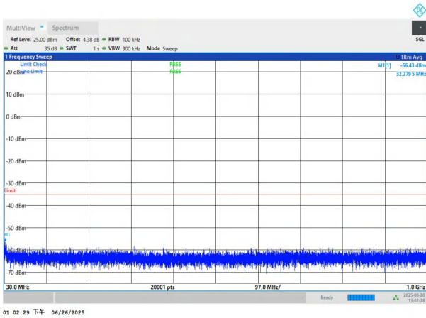
NTNV-n7-PC3-15-10-H-DFT-BPSK-Edge_1RB_Left-30-1000-PAS S
