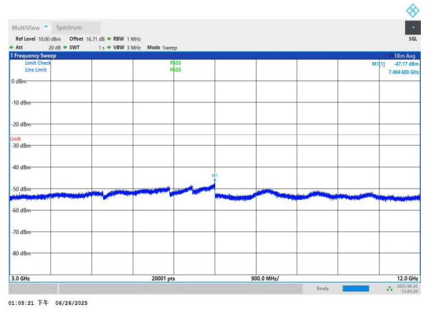
NTNV-n7-PC3-15-15-M-DFT-BPSK-Edge_1RB_Left-3000-12000-PASS PASS
