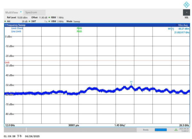
NTNV-n7-PC3-15-20-M-DFT-QPSK-Edge_1RB_Left-12000-2650 0-PASS
