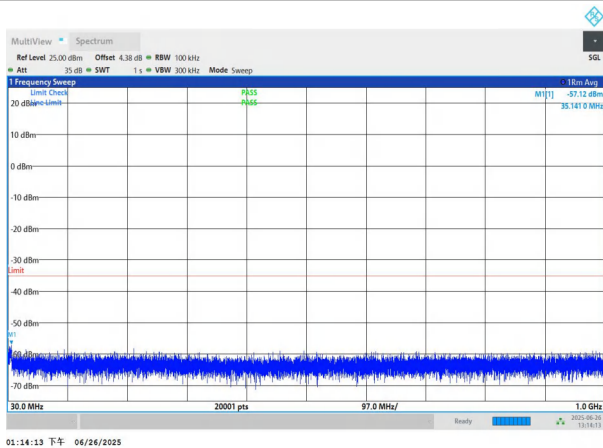
NTNV-n7-PC3-15-25-H-DFT-BPSK-Edge_1RB_Left-30-1000-PASS
