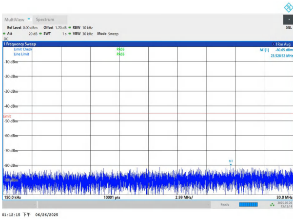
NTNV-n7-PC3-15-25-L-DFT-QPSK-Edge_1RB_Left-0.15-30-PAS
