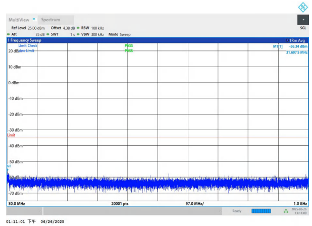
NTNV-n7-PC3-15-20-H-DFT-QPSK-Edge_1RB_Left-30-1000-PAS S
