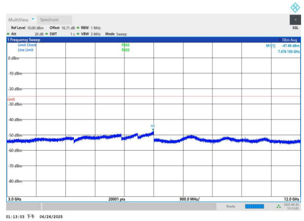
NTNV-n7-PC3-15-25-M-DFT-BPSK-Edge_1RB_Left-3000-12000- PASS
