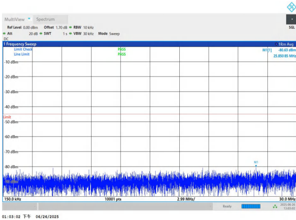
NTNV-n7-PC3-15-10-H-DFT-QPSK-Edge_1RB_Left-0.15-30-PAS
