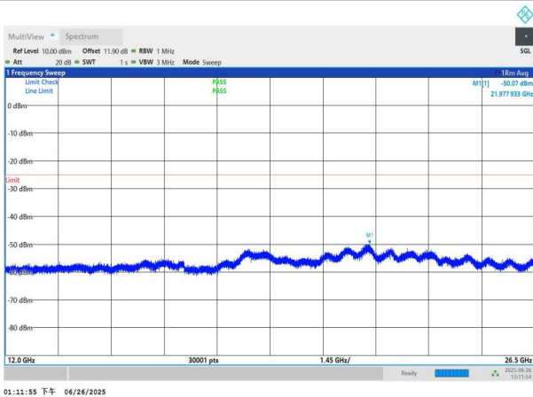
NTNV-n7-PC3-15-25-L-DFT-BPSK-Edge_1RB_Left-12000-26500 -PASS
