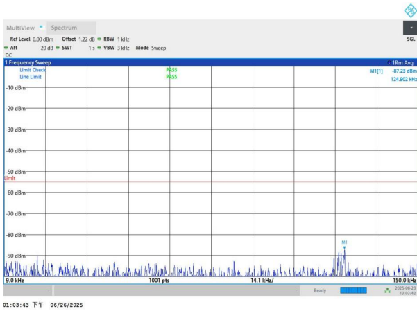
NTNV-n7-PC3-15-15-L-DFT-BPSK-Edge_1RB_Left-0.009-0.15-P ASS
