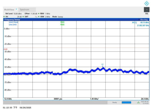
NTNV-n7-PC3-15-25-H-DFT-QPSK-Edge_1RB_Left-12000-26500 -PASS
