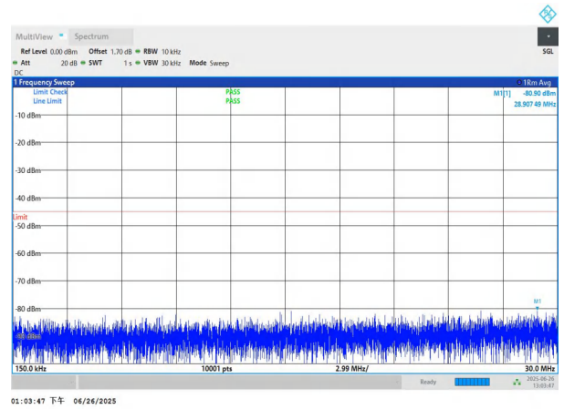
NTNV-n7-PC3-15-15-L-DFT-BPSK-Edge_1RB_Left-0.15-30-PAS S
