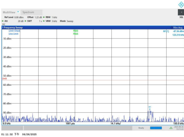
NTNV-n7-PC3-15-25-L-DFT-BPSK-Edge_1RB_Left-0.009-0.15-P ASS
