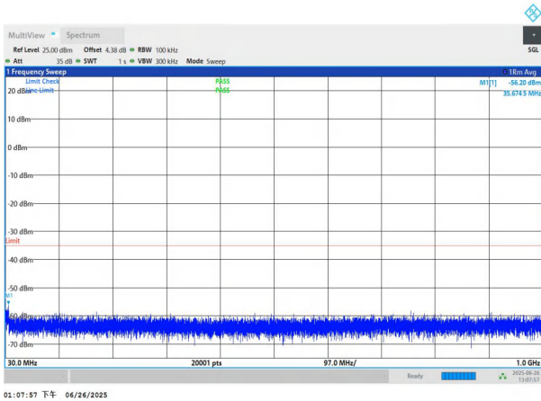
NTNV-n7-PC3-15-20-L-DFT-BPSK-Edge_1RB_Left-30-1000-PAS S
