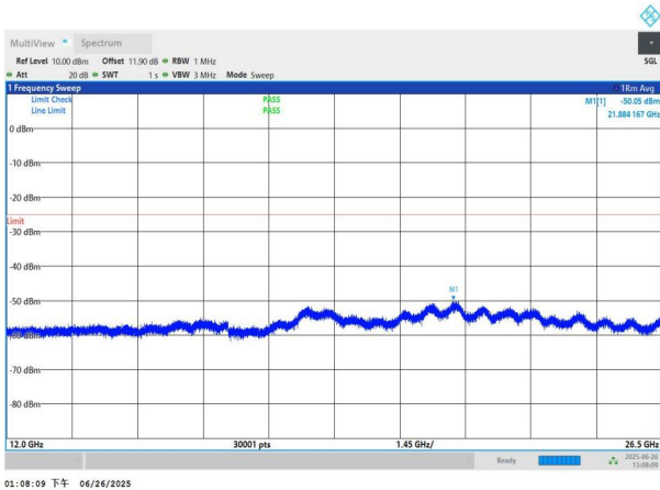
NTNV-n7-PC3-15-20-L-DFT-BPSK-Edge_1RB_Left-12000-26500 -PASS
