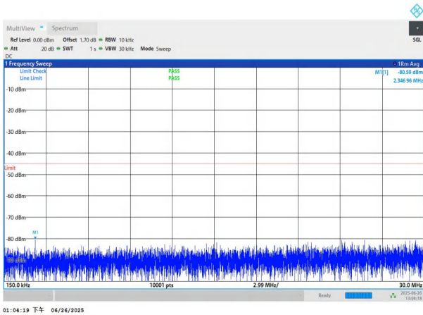
NTNV-n7-PC3-15-15-L-DFT-QPSK-Edge_1RB_Left-0.15-30-PAS
