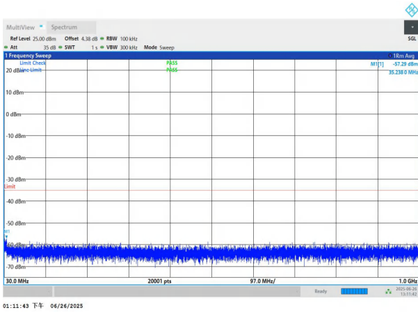
NTNV-n7-PC3-15-25-L-DFT-BPSK-Edge_1RB_Left-30-1000-PAS S
