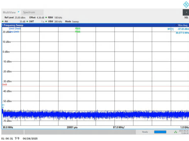
NTNV-n7-PC3-15-15-H-DFT-BPSK-Edge_1RB_Left-30-1000-PAS S
