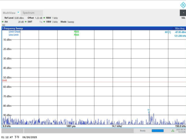
NTNV-n7-PC3-15-25-M-DFT-BPSK-Edge_1RB_Left-0.009-0.15-PASS
