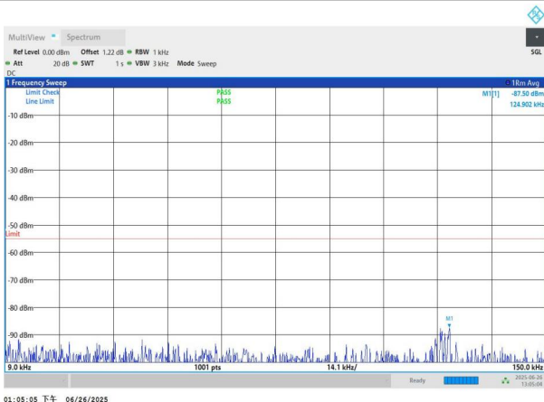
NTNV-n7-PC3-15-15-M-DFT-BPSK-Edge_1RB_Left-0.009-0.15-PASS
