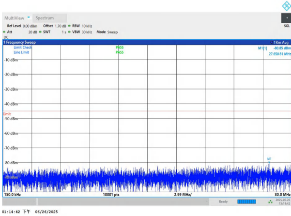
NTNV-n7-PC3-15-25-H-DFT-QPSK-Edge_1RB_Left-0.15-30-PAS S
