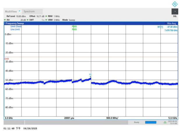
NTNV-n7-PC3-15-25-L-DFT-BPSK-Edge_1RB_Left-3000-12000-PASS PASS
