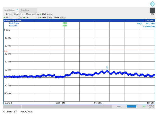
NTNV-n7-PC3-15-10-M-DFT-QPSK-Edge_1RB_Left-12000-2650 0-PASS
