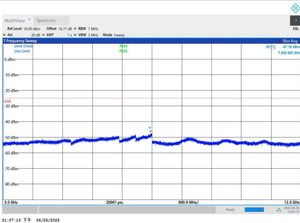
NTNV-n7-PC3-15-15-H-DFT-QPSK-Edge_1RB_Left-3000-12000-PASS
