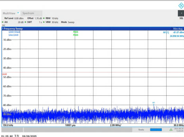
NTNV-n7-PC3-15-15-M-DFT-QPSK-Edge_1RB_Left-0.15-30-PAS S
