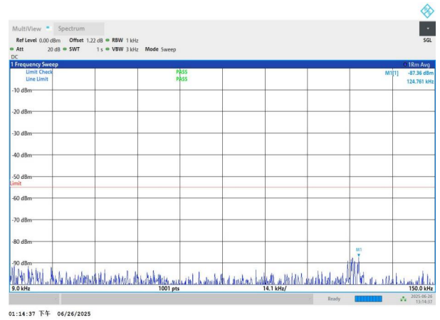
NTNV-n7-PC3-15-25-H-DFT-QPSK-Edge_1RB_Left-0.009-0.15-P ASS
