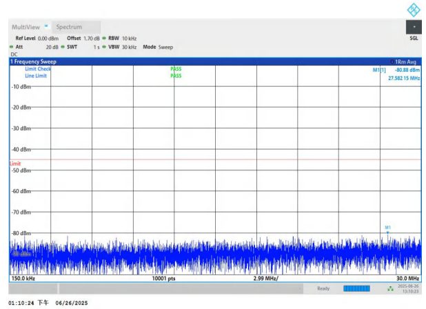
NTNV-n7-PC3-15-20-H-DFT-BPSK-Edge_1RB_Left-0.15-30-PAS S
