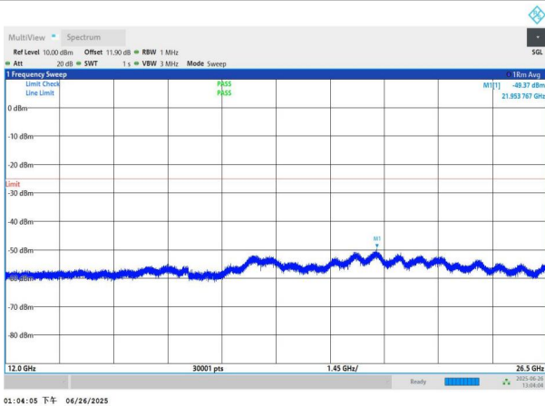
NTNV-n7-PC3-15-15-L-DFT-BPSK-Edge_1RB_Left-12000-26500 -PASS
