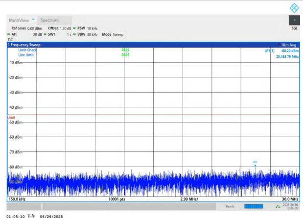
NTNV-n7-PC3-15-15-M-DFT-BPSK-Edge_1RB_Left-0.15-30-PAS
