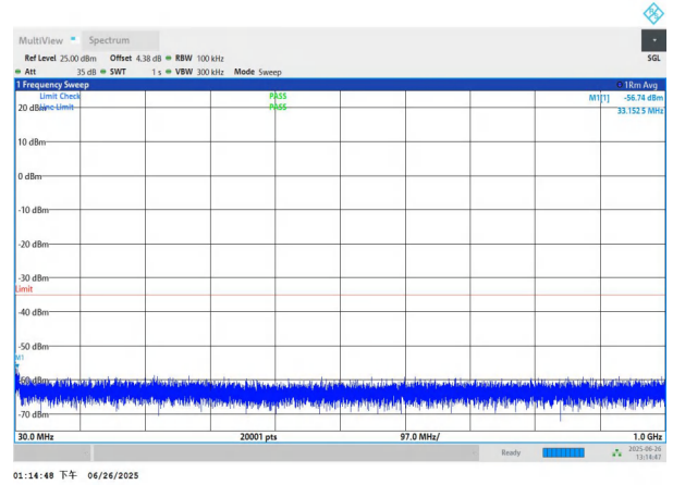
NTNV-n7-PC3-15-25-H-DFT-QPSK-Edge_1RB_Left-30-1000-PAS S
