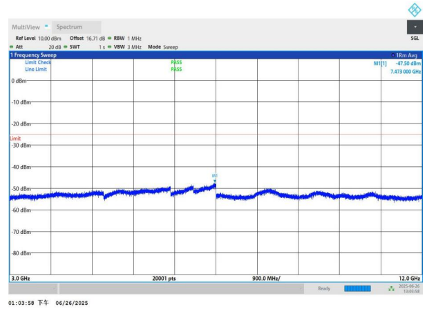
NTNV-n7-PC3-15-15-L-DFT-BPSK-Edge_1RB_Left-3000-12000-PASS PASS
