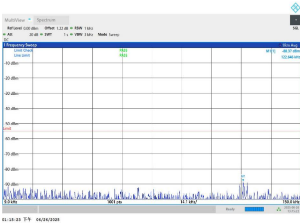
NTNV-n7-PC3-15-30-L-DFT-BPSK-Edge_1RB_Left-0.009-0.15-P ASS
