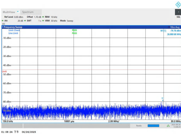
NTNV-n7-PC3-15-20-L-DFT-QPSK-Edge_1RB_Left-0.15-30-PAS
