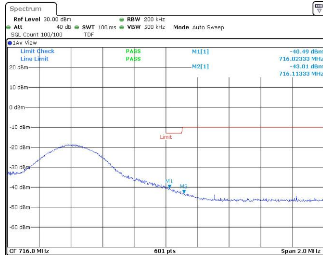
Band12-10MHz-16QAM-23130-1RB#49
