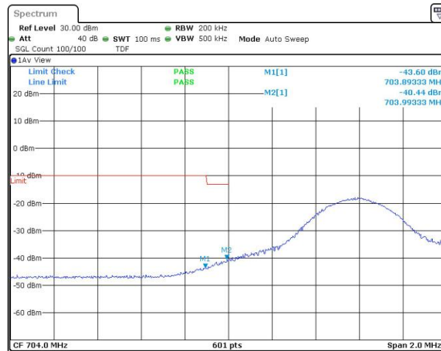
Band17-10MHz-16QAM-23780-50RB#0
