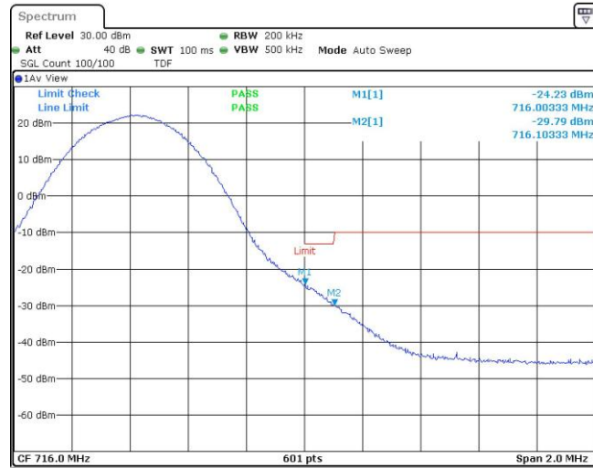
Band12-10MHz-16QAM-23130-50RB#0
