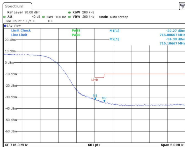
Band12-10MHz-16QAM-23060-1RB#0
