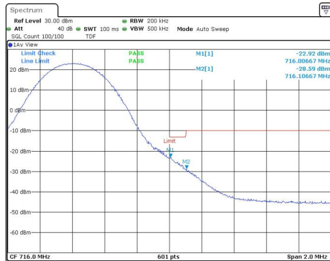
Band17-10MHz-QPSK-23800-50RB#0
