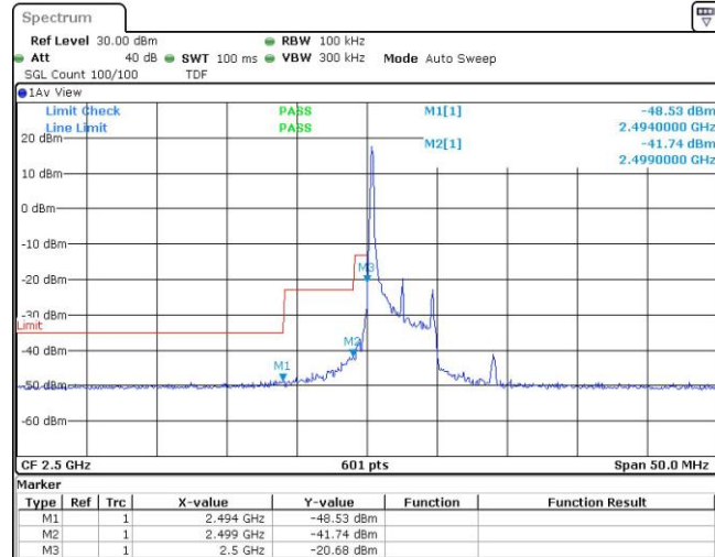
Band41-5MHz-16QAM-39715-1RB#24
