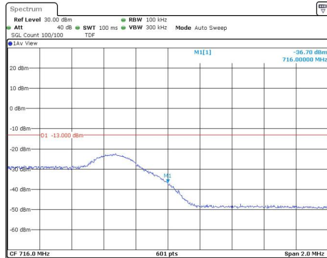
Band17-5MHz-QPSK-23825-1RB#24
