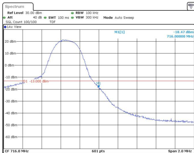
Band12-5MHz-16QAM-23155-25RB#0
