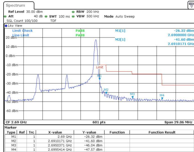
Band41-10MHz-QPSK-41540-50RB#0
