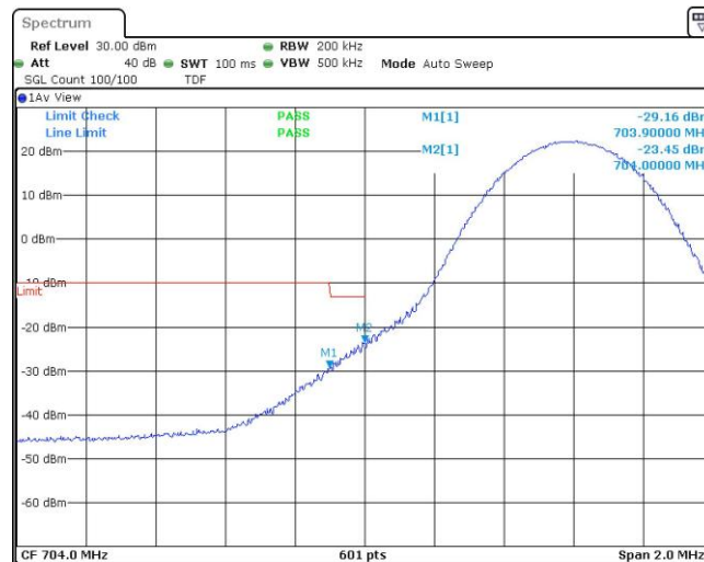
Band17-10MHz-16QAM-23780-1RB#49
