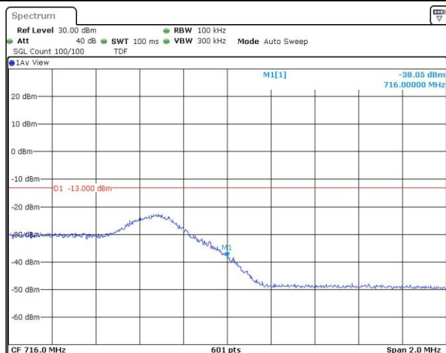
Band12-5MHz-16QAM-23155-1RB#24
