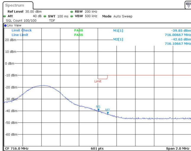
Band12-10MHz-QPSK-23130-1RB#49
