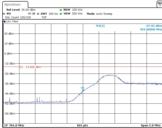
Band17-5MHz-16QAM-23755-25RB#0
