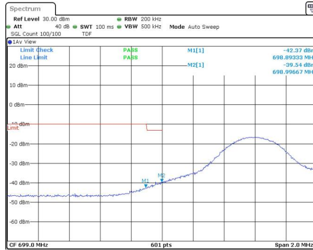
Band12-10MHz-QPSK-23060-50RB#0
