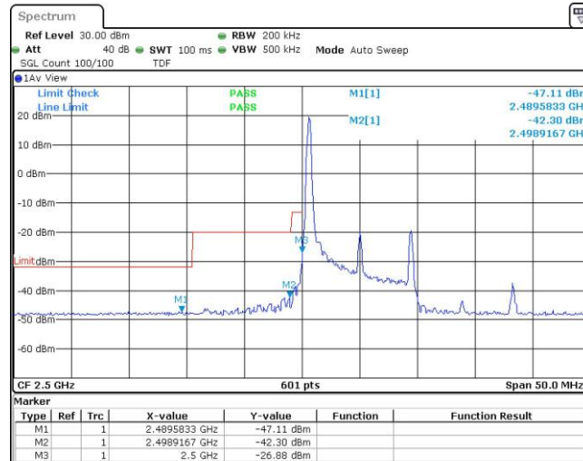
Band41-10MHz-16QAM-39740-1RB#49
