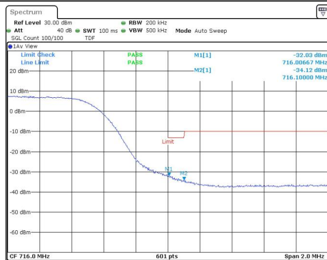
Band17-10MHz-16QAM-23780-1RB#0
