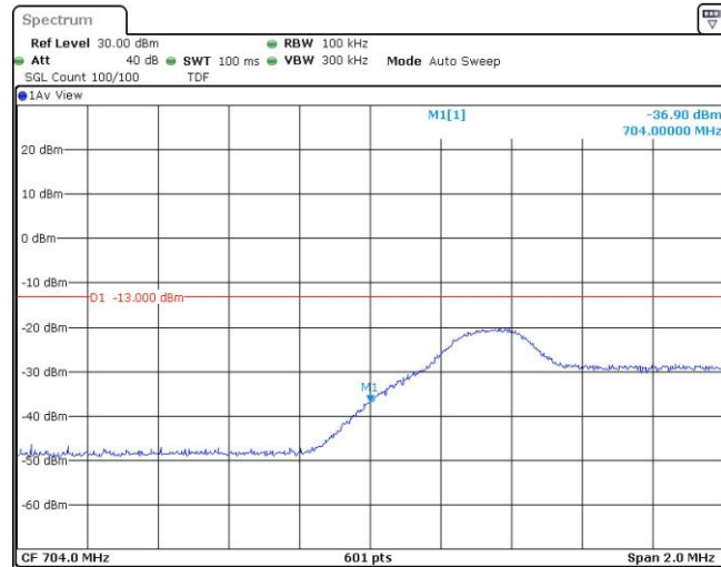
Band17-5MHz-QPSK-23755-25RB#0
