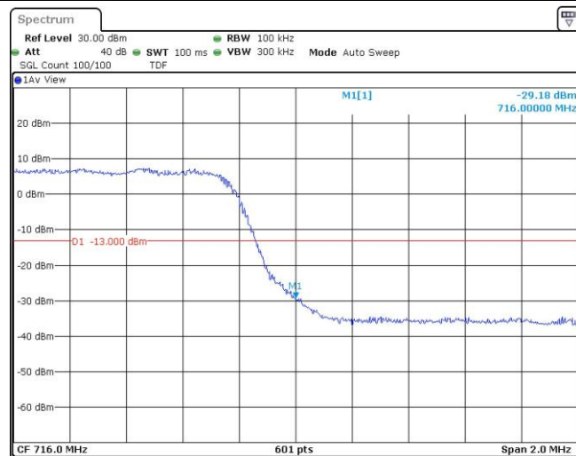
Band17-10MHz-QPSK-23780-1RB#0
