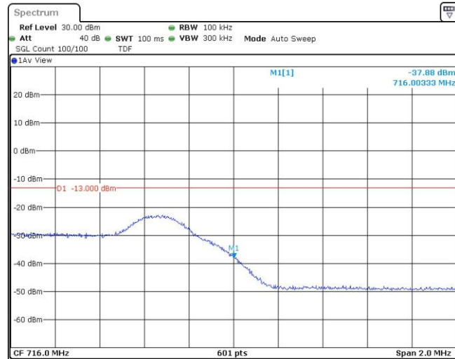
Band17-5MHz-16QAM-23825-1RB#24
