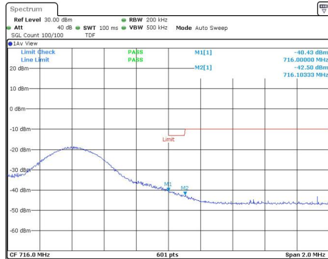
Band17-10MHz-16QAM-23800-1RB#49
