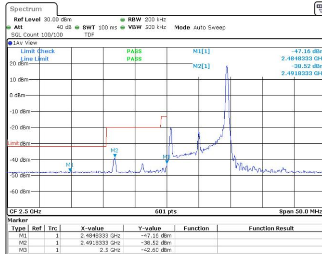
Band41-10MHz-16QAM-39740-50RB#0
