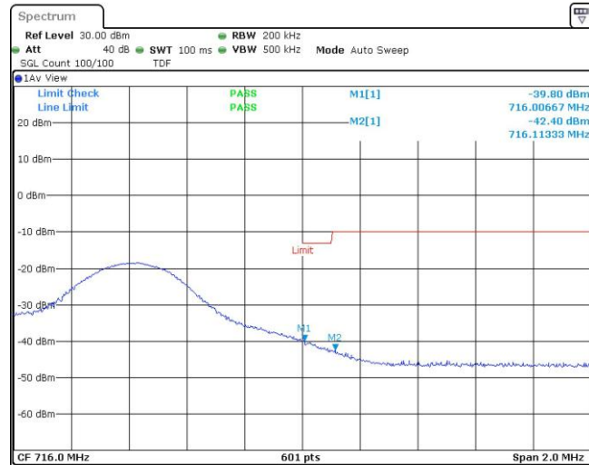
Band17-10MHz-QPSK-23800-1RB#49
