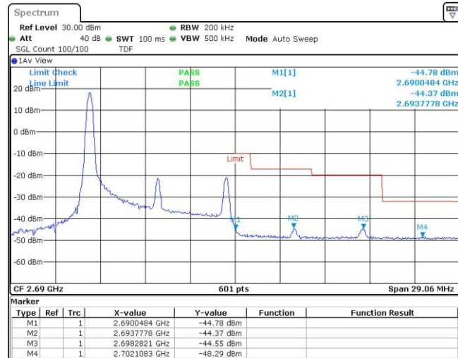
Band41-10MHz-QPSK-41540-1RB#49
