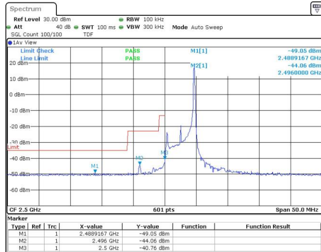
Band41-5MHz-16QAM-39715-25RB#0
