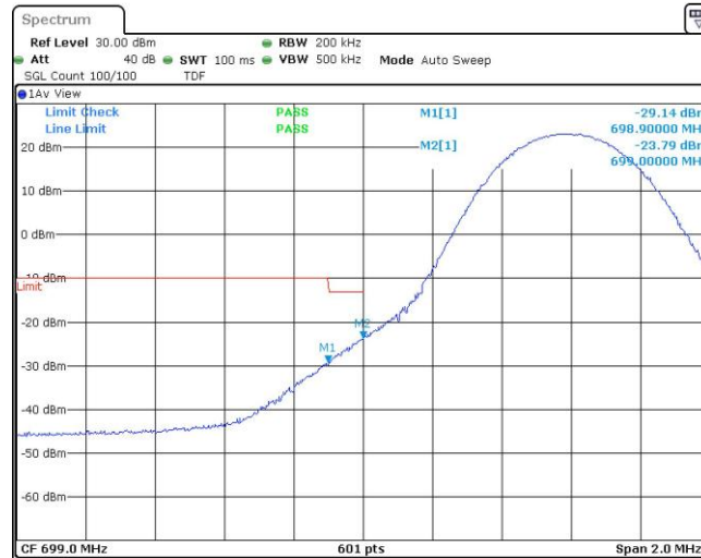
Band12-10MHz-QPSK-23060-1RB#49
