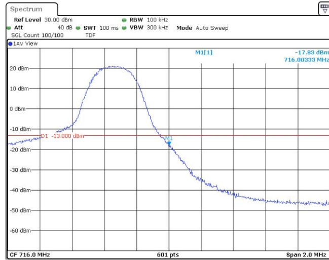
Band17-5MHz-16QAM-23825-25RB#0
