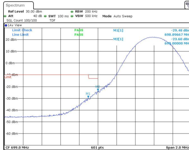
Band12-10MHz-16QAM-23060-1RB#49
