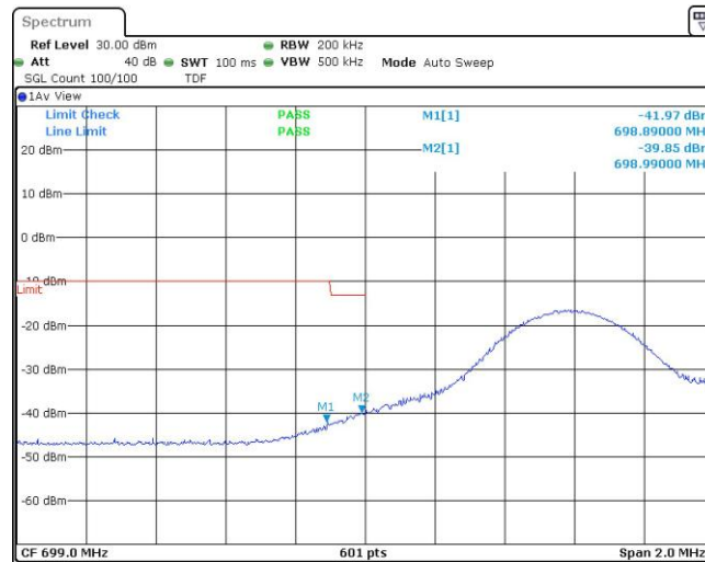
Band12-10MHz-16QAM-23060-50RB#0
