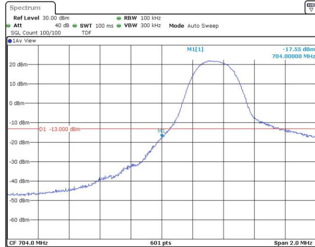
Band17-5MHz-QPSK-23755-1RB#24
