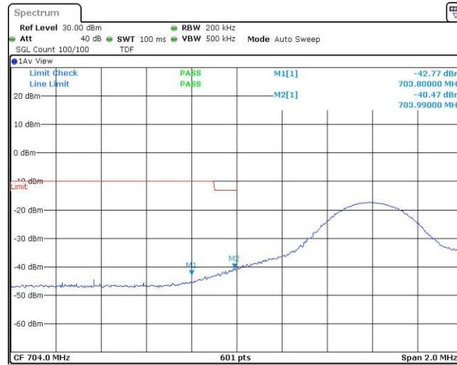
Band17-10MHz-QPSK-23780-50RB#0
