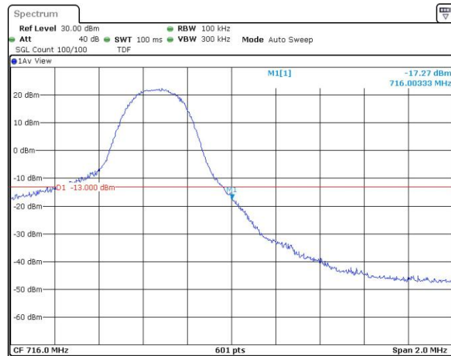
Band17-5MHz-QPSK-23825-25RB#0
