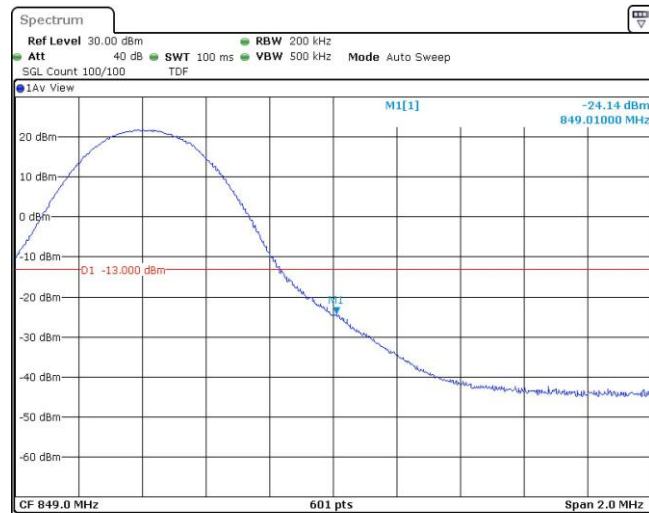
Band5-10MHz-QPSK-20600-50RB#0
