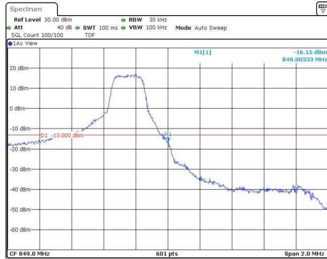
Band5-1.4MHz-16QAM-20643-6RB#0
