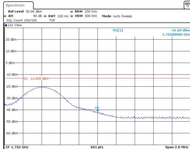
Band4-10MHz-16QAM-20350-1RB#49
