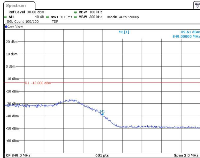
Band5-5MHz-16QAM-20625-1RB#24
