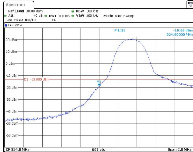
Band5-5MHz-QPSK-20425-1RB#24
