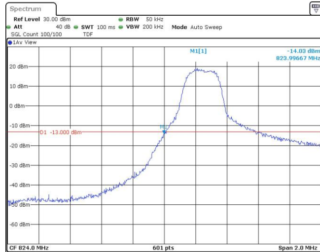
Band5-3MHz-16QAM-20415-1RB#14
