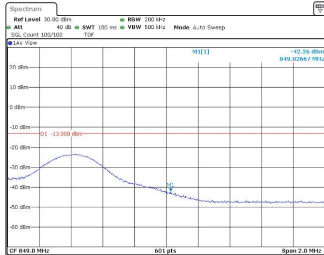
Band5-10MHz-QPSK-20600-1RB#49
