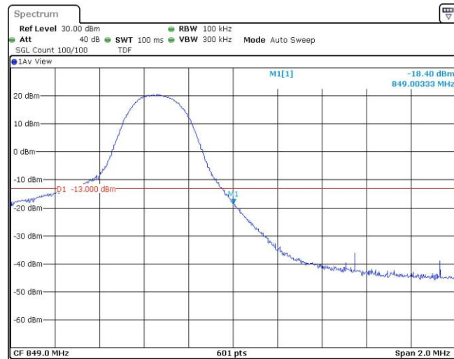
Band5-5MHz-QPSK-20625-25RB#0
