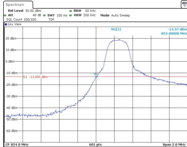
Band5-3MHz-QPSK-20415-1RB#14
