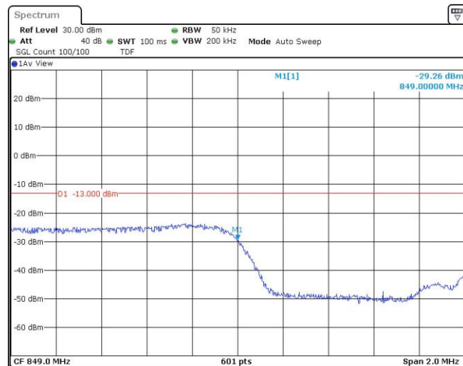
Band5-3MHz-16QAM-20635-1RB#14
