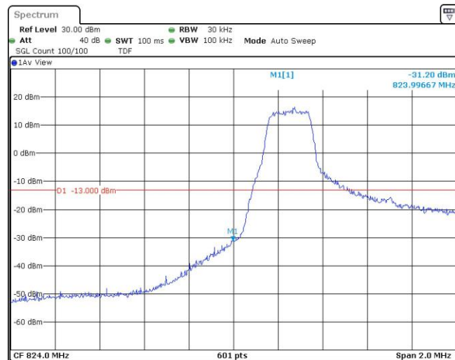
Band5-1.4MHz-16QAM-20407-1RB#5
