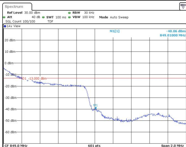
Band5-1.4MHz-QPSK-20643-1RB#5
