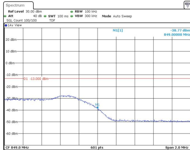
Band5-5MHz-QPSK-20625-1RB#24
