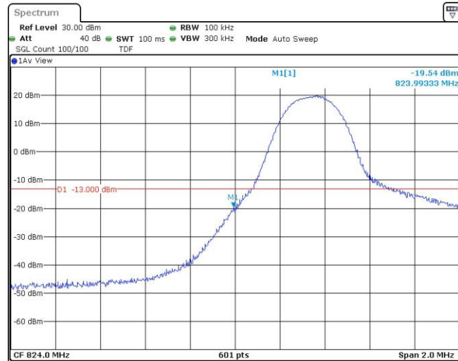
Band5-5MHz-16QAM-20425-1RB#24
