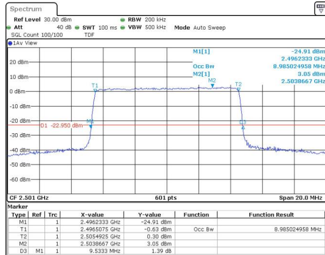
Band41-10MHz-16QAM-39740-50RB#0
