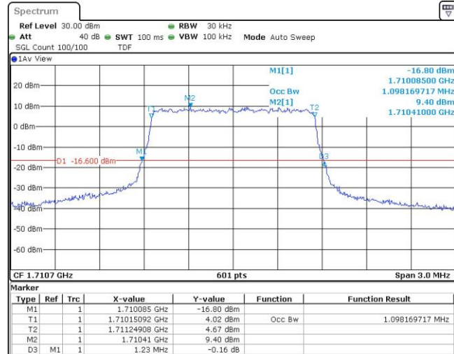
Band66-1.4MHz-QPSK-132322-6RB#0
