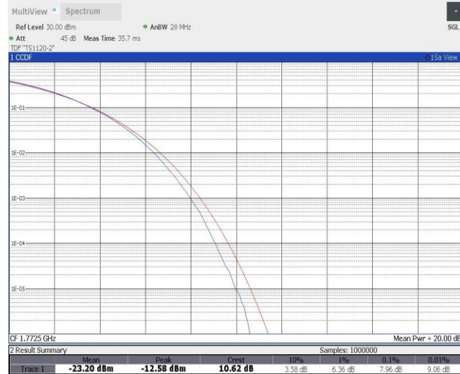
Band66-15MHz-QPSK-132597-75RB#0
