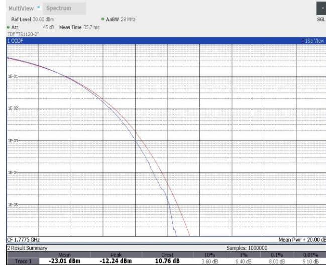
Band66-5MHz-16QAM-132647-25RB#0
