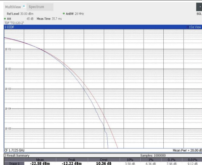
Band66-5MHz-QPSK-131997-25RB#0
