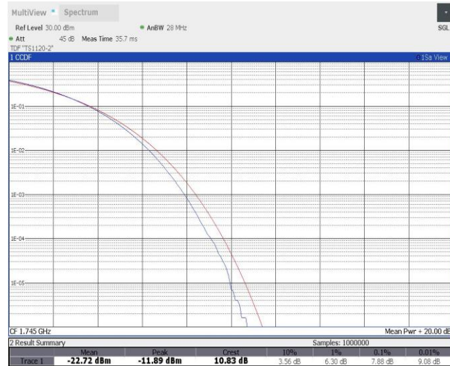
Band66-15MHz-QPSK-132322-75RB#0
