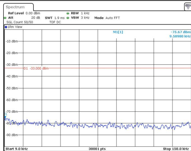
Band5-4132-2-0.009~0.15MHz
