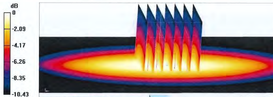
0 dB = 3.30 W/kg = 5.19 dBW/kg
