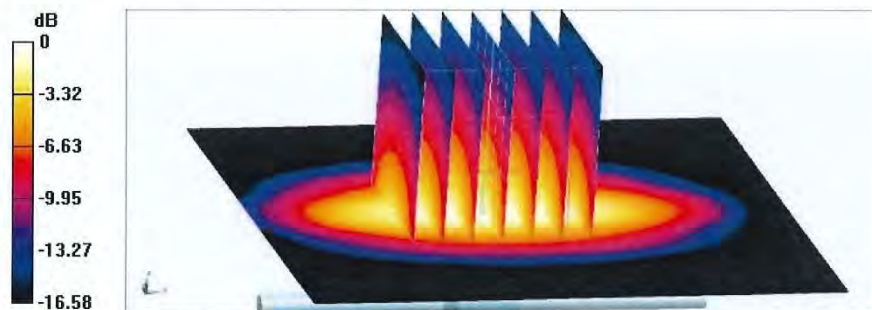
0 dB = 14.0 W/kg = 11.46 dBW/kg
