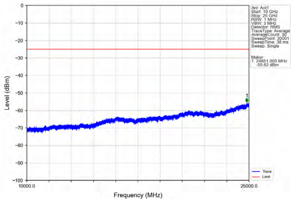
Band7 5MHz 16QAM LCH 2502.5MHz RB 1_0 NTNV
