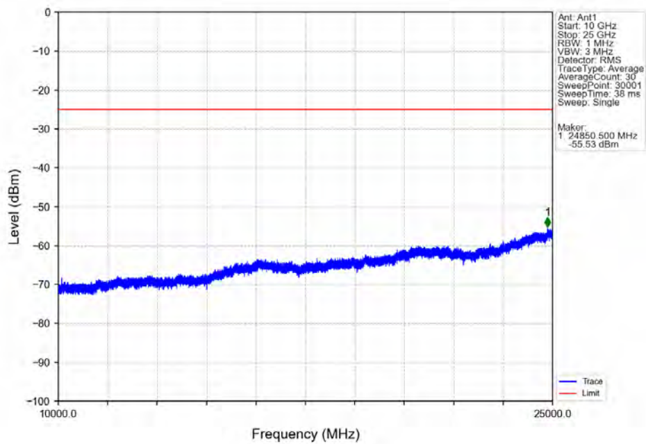
Band7 20MHz 16QAM MCH 2535MHz RB 1 0 NTV
