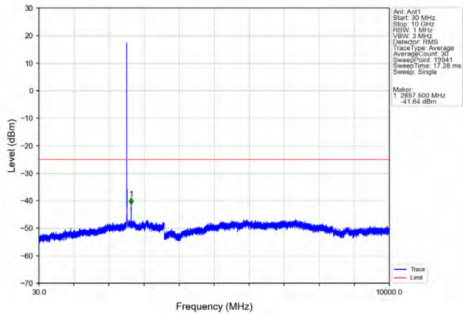
Band7 15MHz 16QAM MCH 2535MHz RB 1 0 NTV
