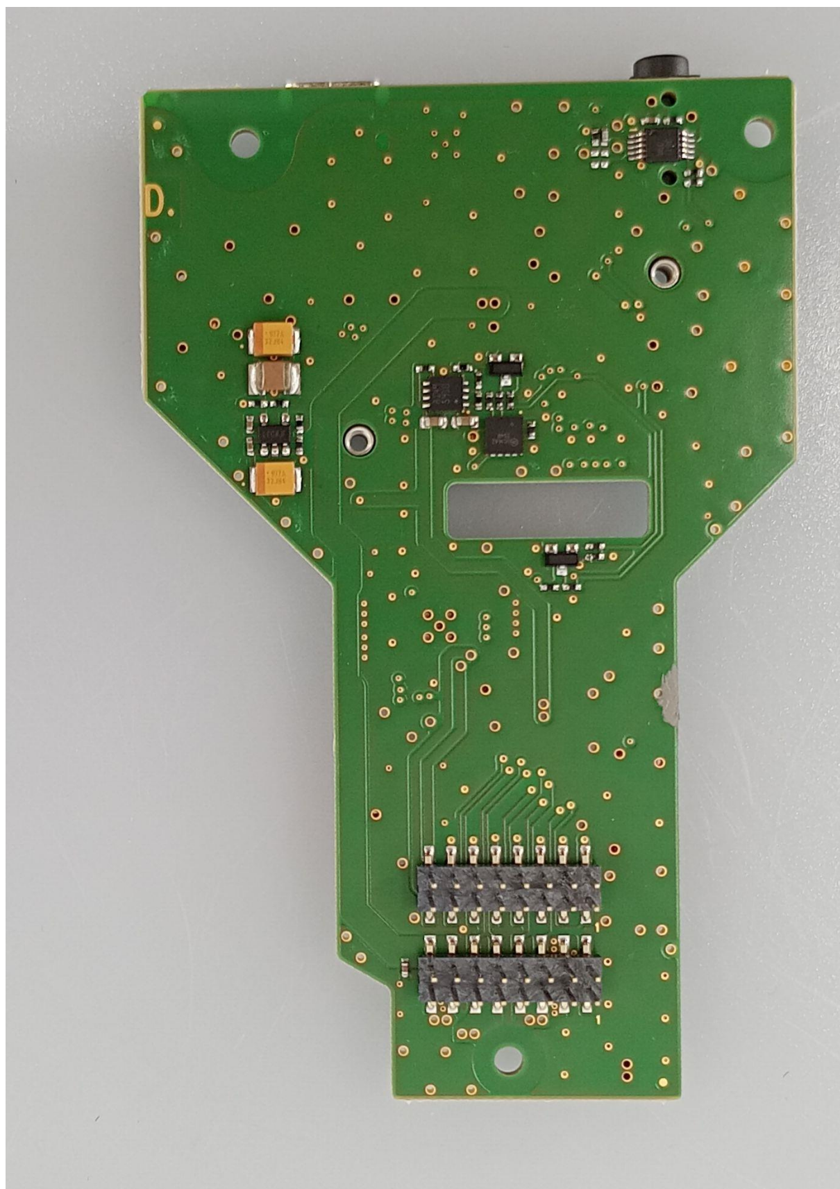
Figure 6 – DS24II-T (back)
