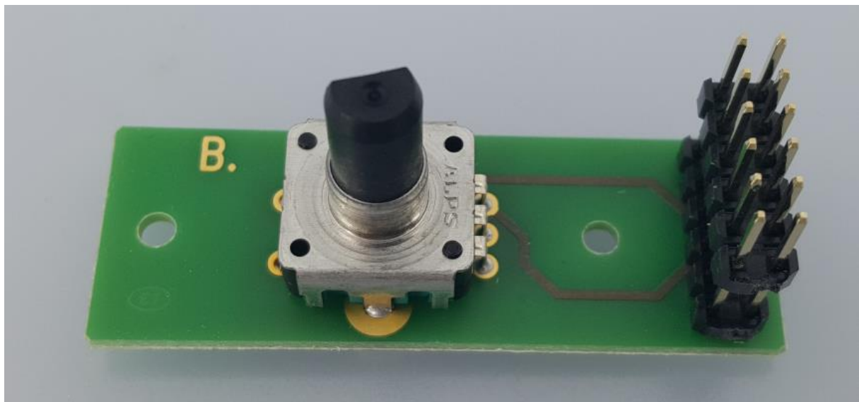
Figure 19 – DC-PW-E2 (back)
