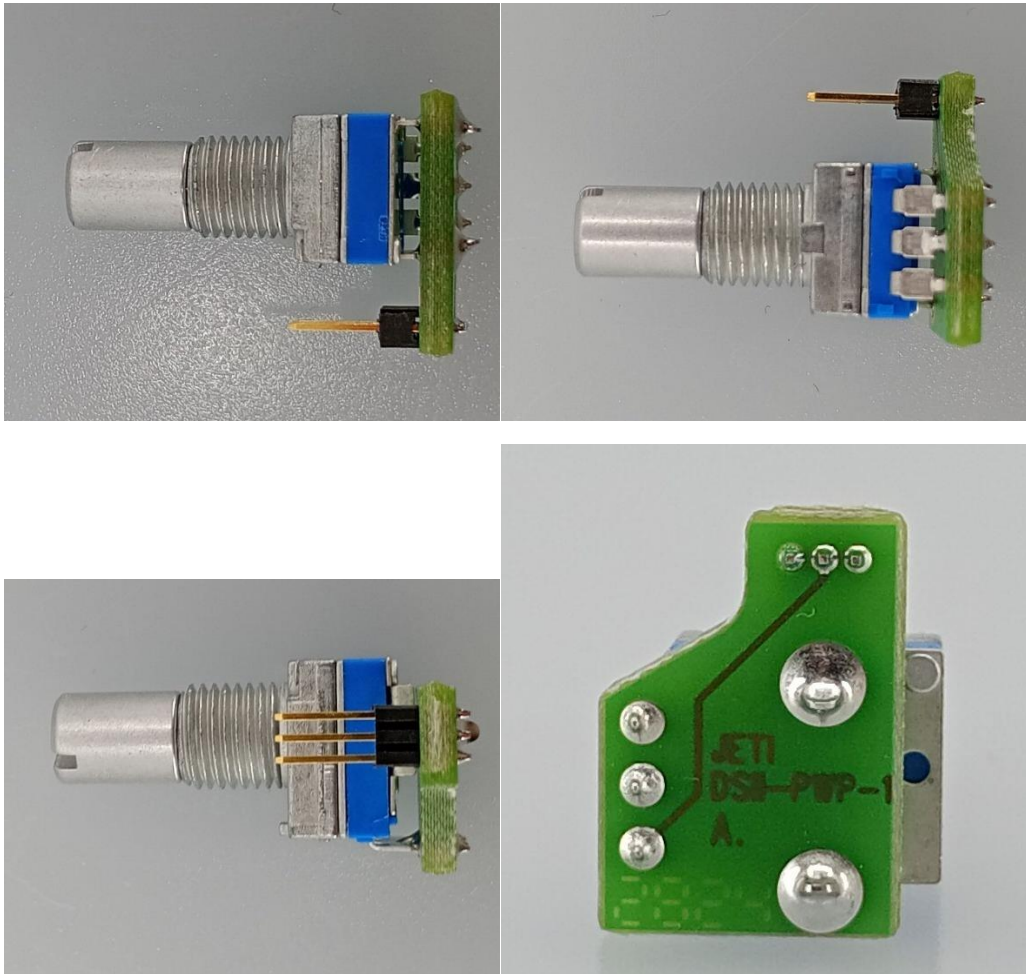
Figure 27 – DSII-PWP
