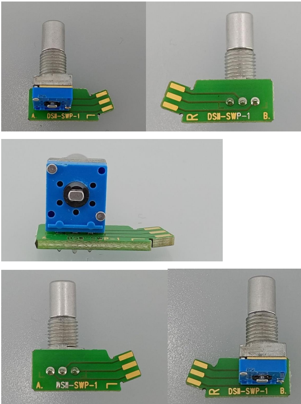
Figure 25 – DS-SWP
