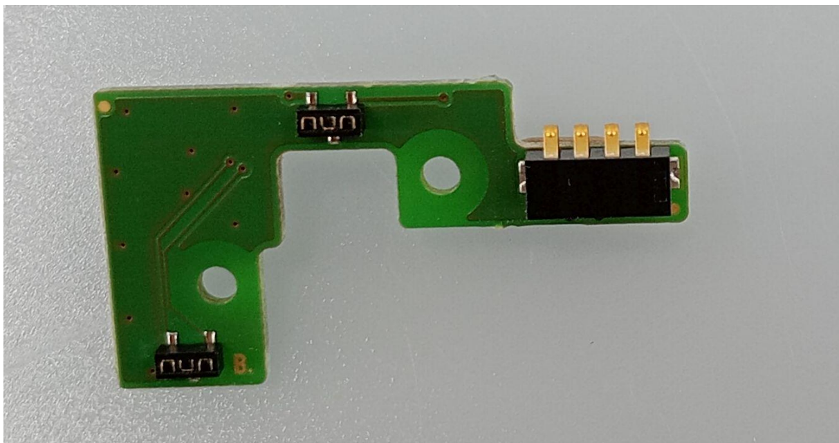
Figure 17 – DS24II-SWR (back)
