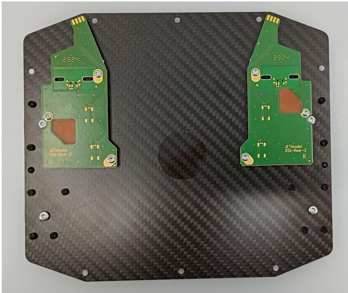
Figure 2– Back plate
