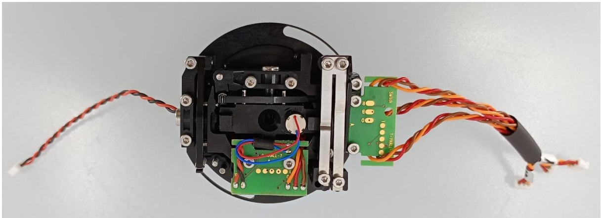
Figure 21 – T-YHALL (front)
