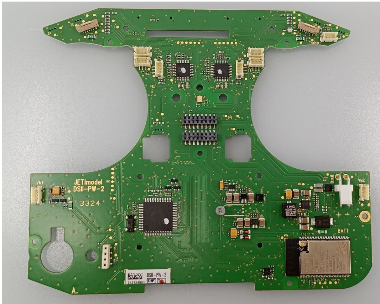
Figure 3 – DS24II-PW (front)
