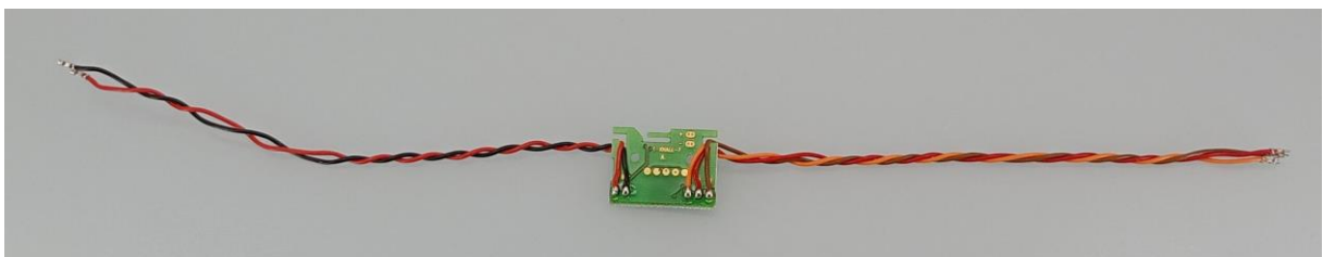
Figure 24 – T-XHALL (back)
