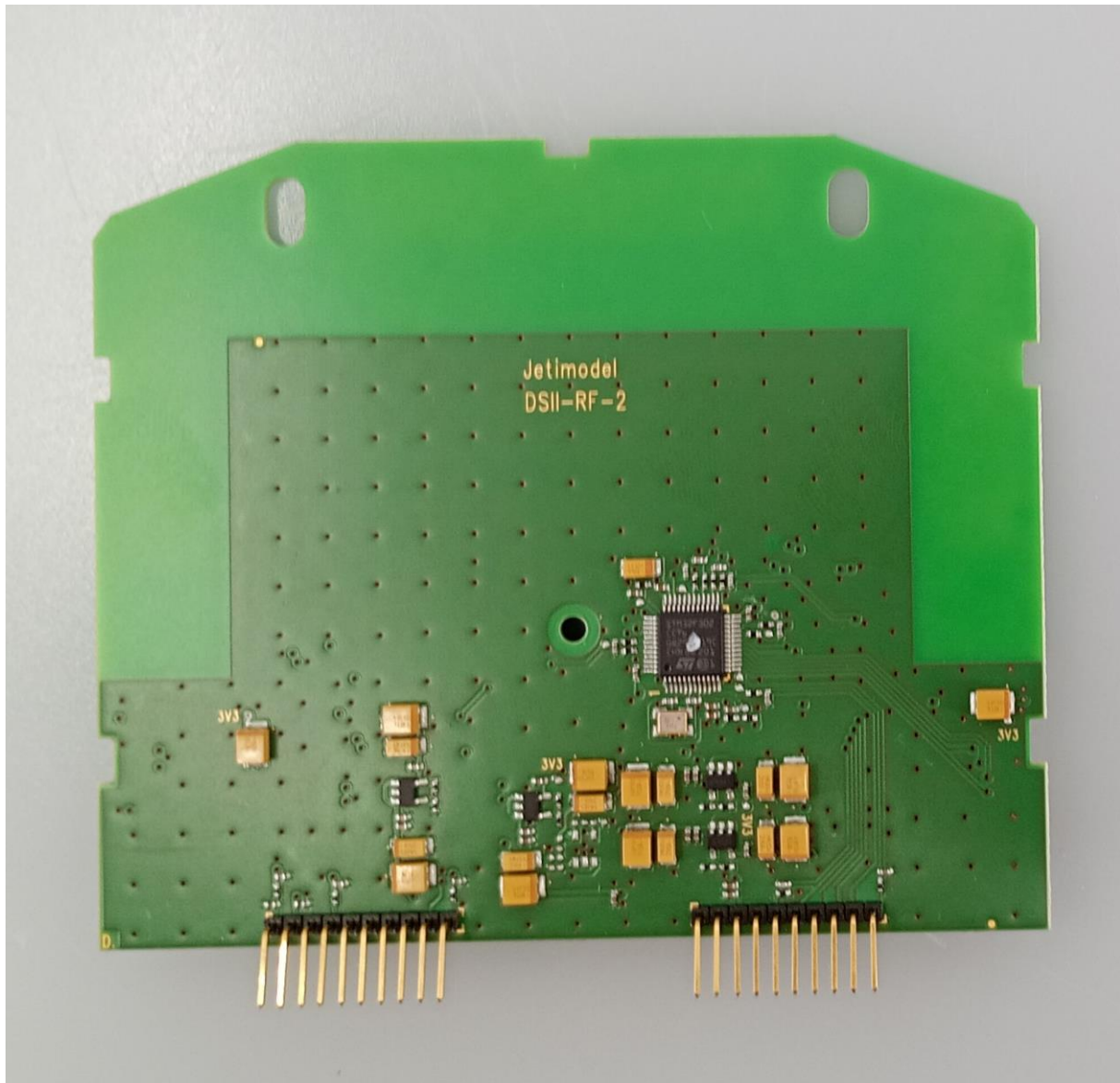
Figure 11 – DS24II-RF (back) RF modules
