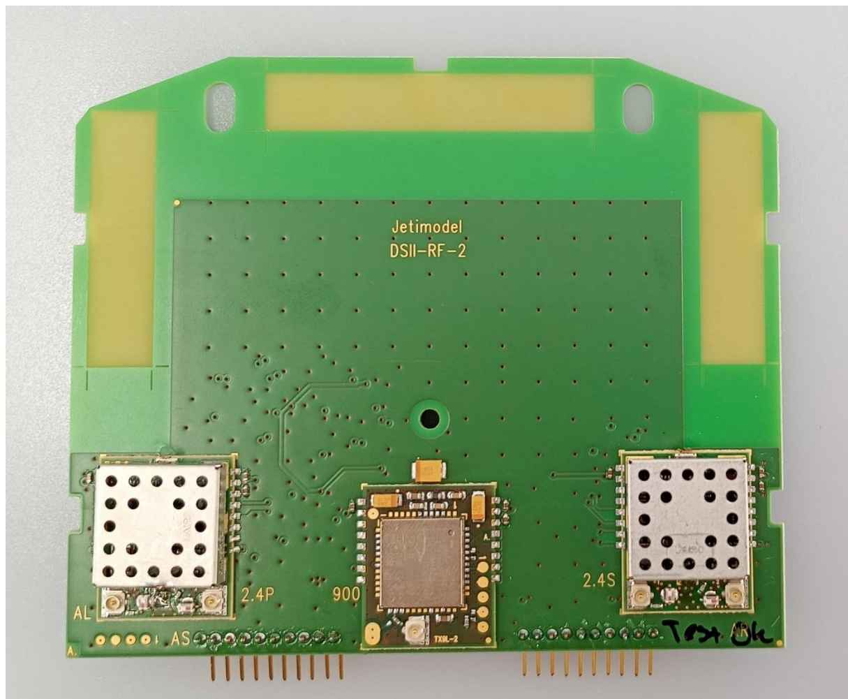
Figure 10 – DS24II-RF RF modules
