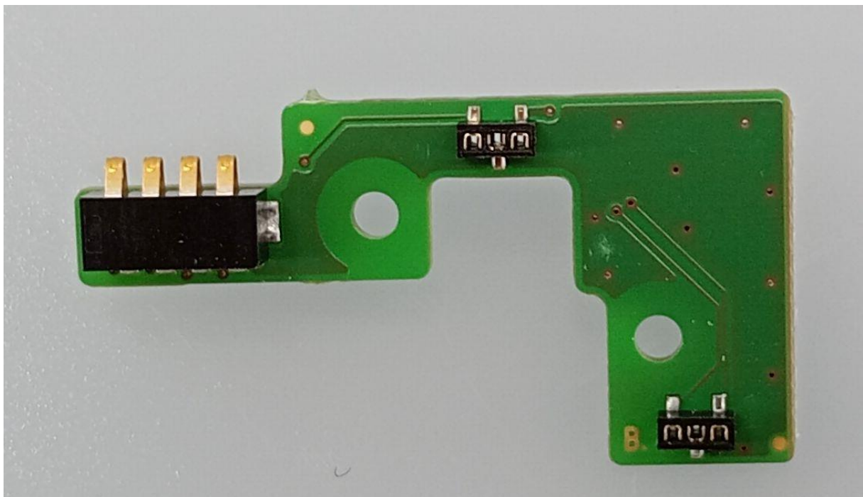
Figure 15 – DS24II-SWL (back)
