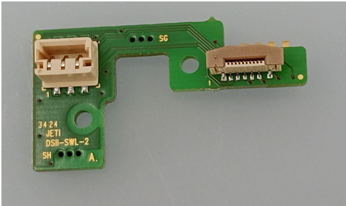
Figure 14 – DS24II-SWL (front)
