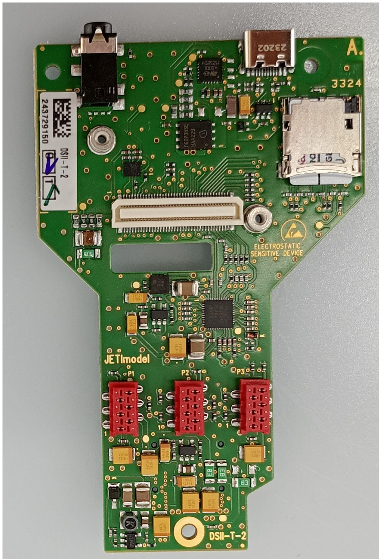
Figure 5 – DS24II-T (front)
