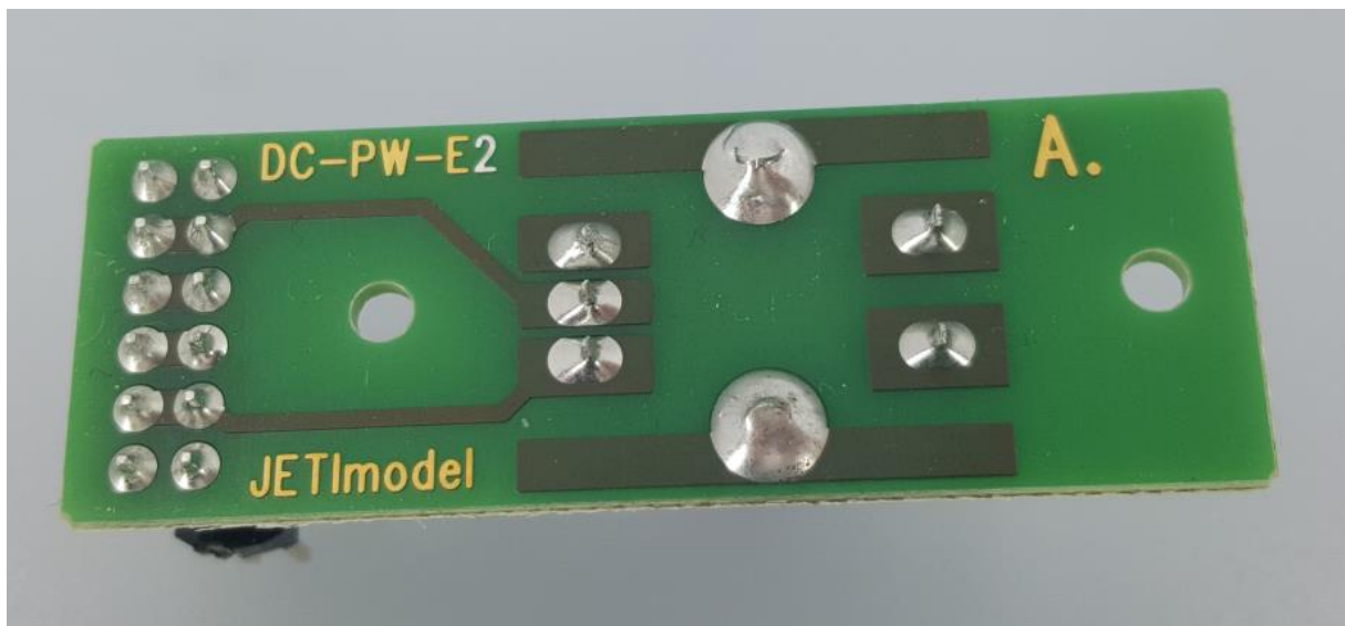
Figure 18 – DC-PW-E2 (front)
