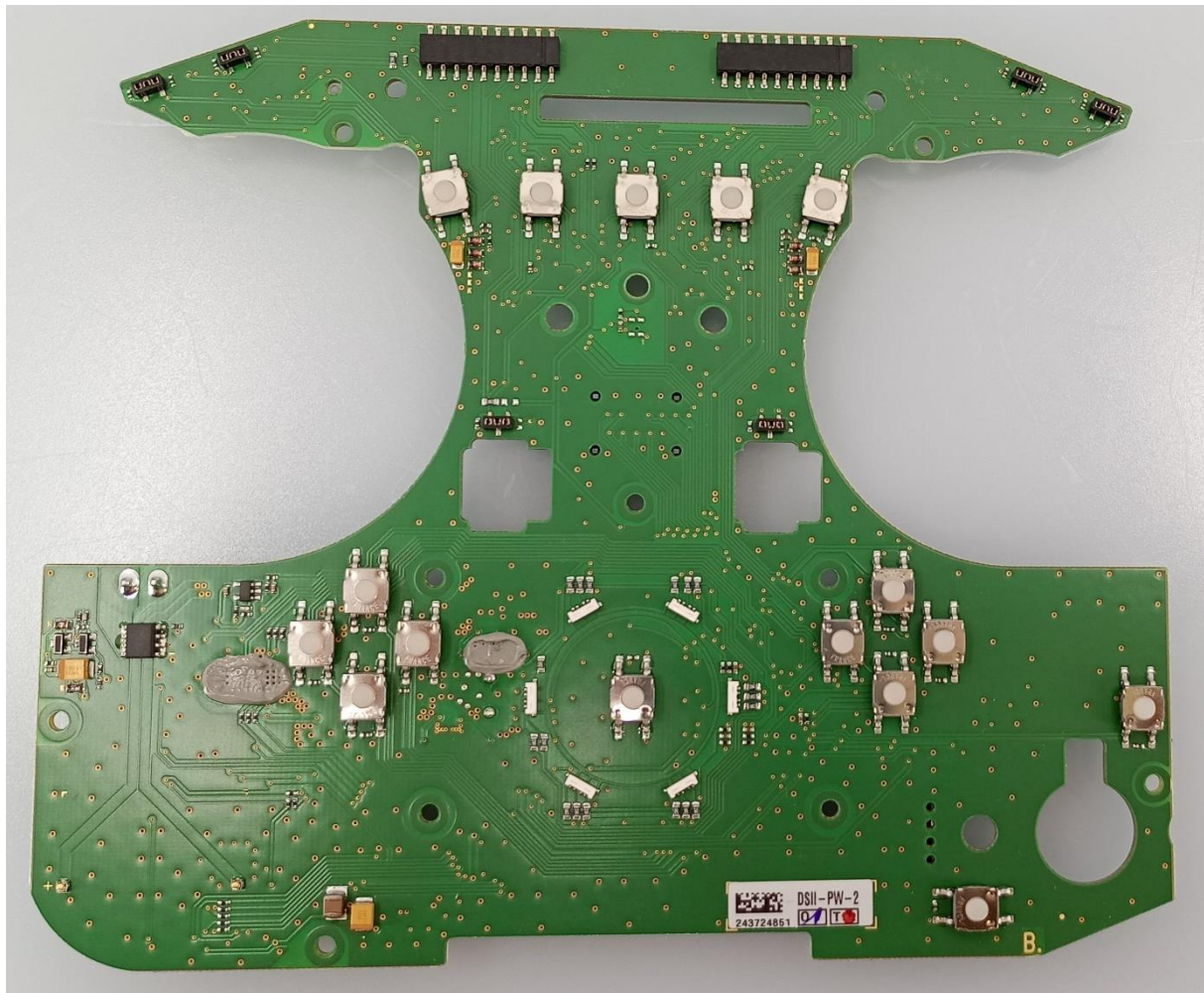
Figure 4 – DS24II-PW (back)
