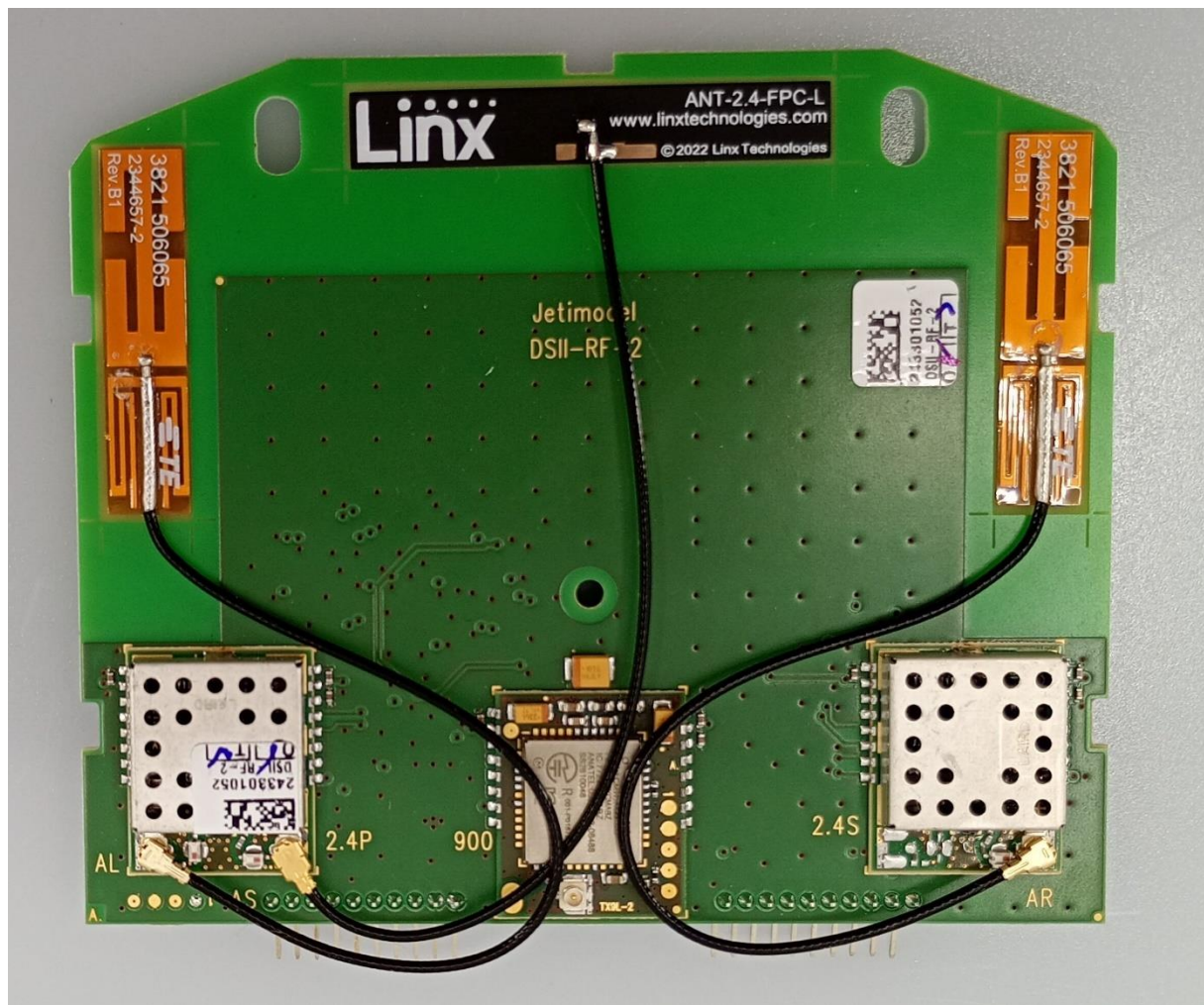
Figure 32 – DS24II-RF module with antennas
