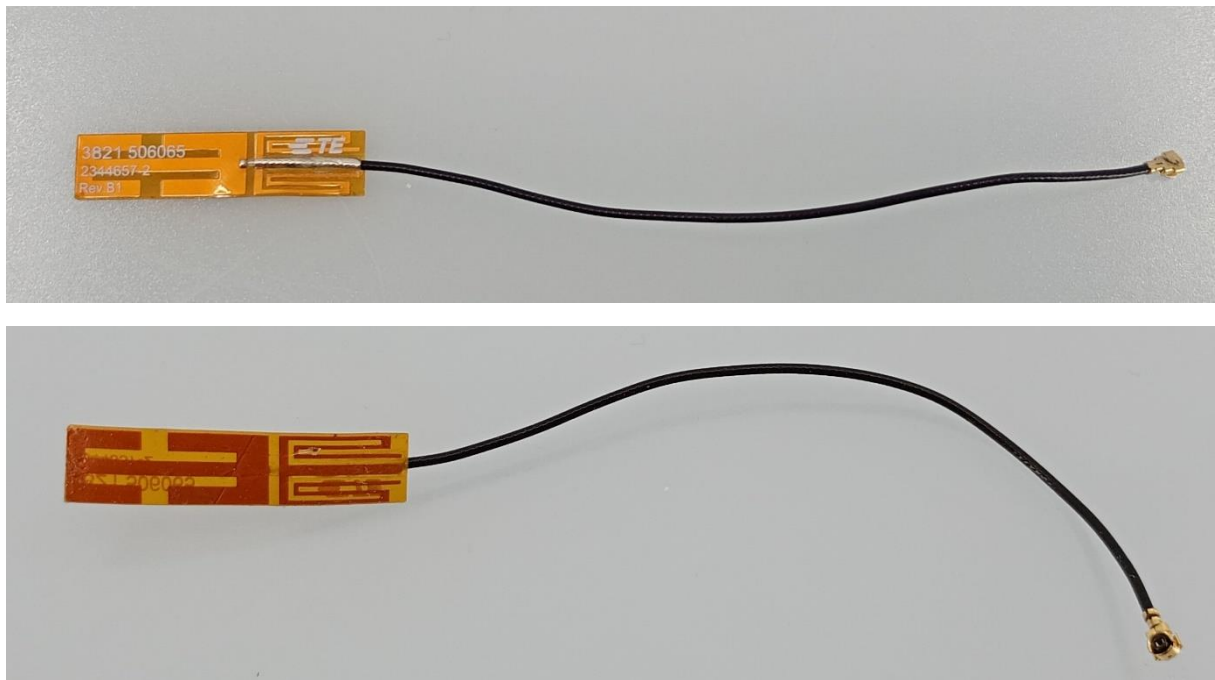
Figure 30 – 2.4GHz antenna (AP1, AS1 - 2344657-2)
