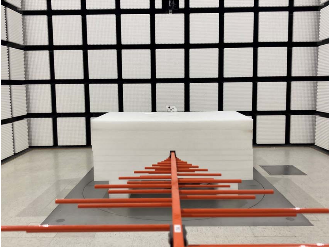
Radiated Emissions Below 1G rear View
