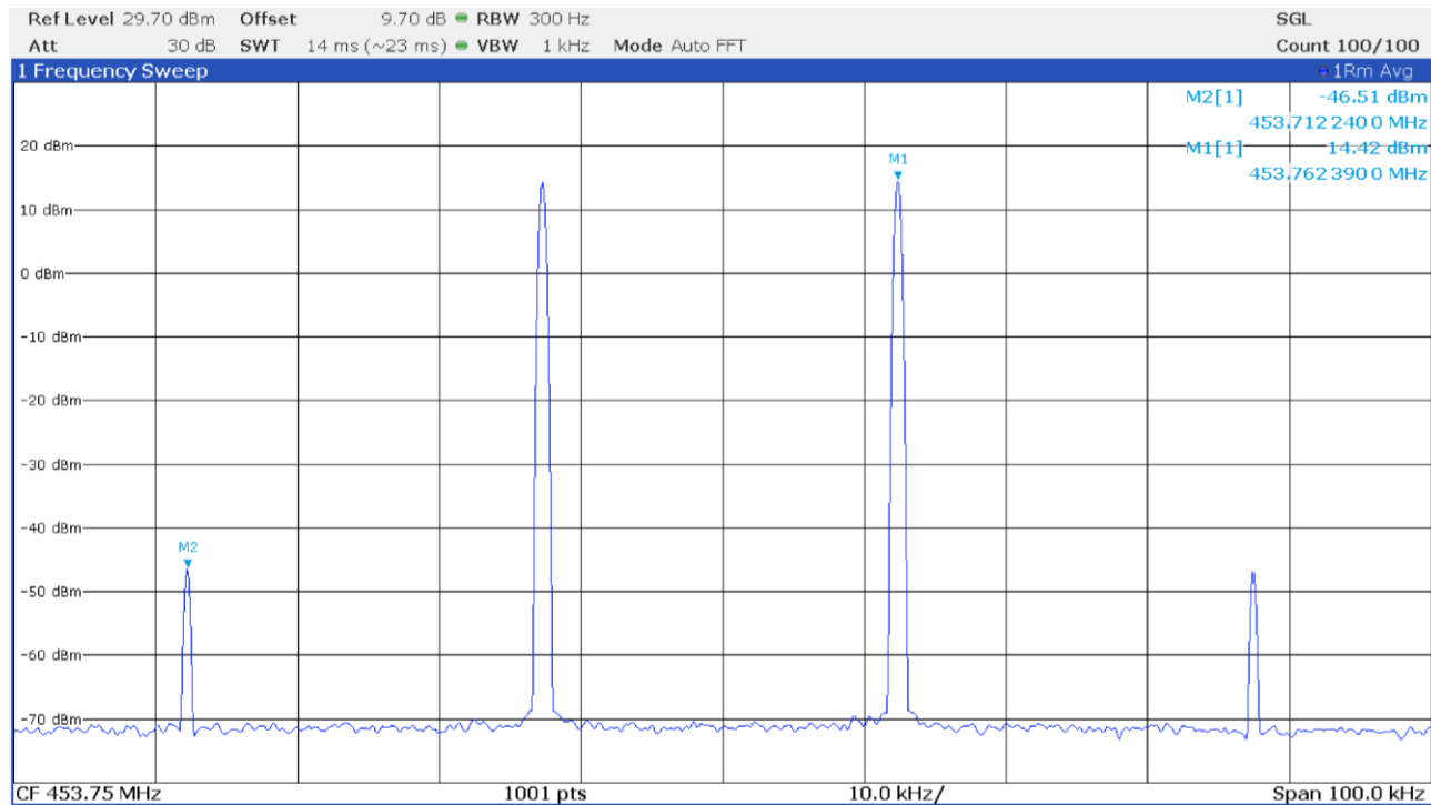
Figure 8.5-1: Down link intermodulation products with input signal at AGC threshold
