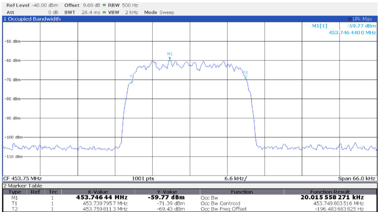
Figure 8.3-1: 99% occupied bandwidth, input signal at AGC threshold spectral plot – down link
