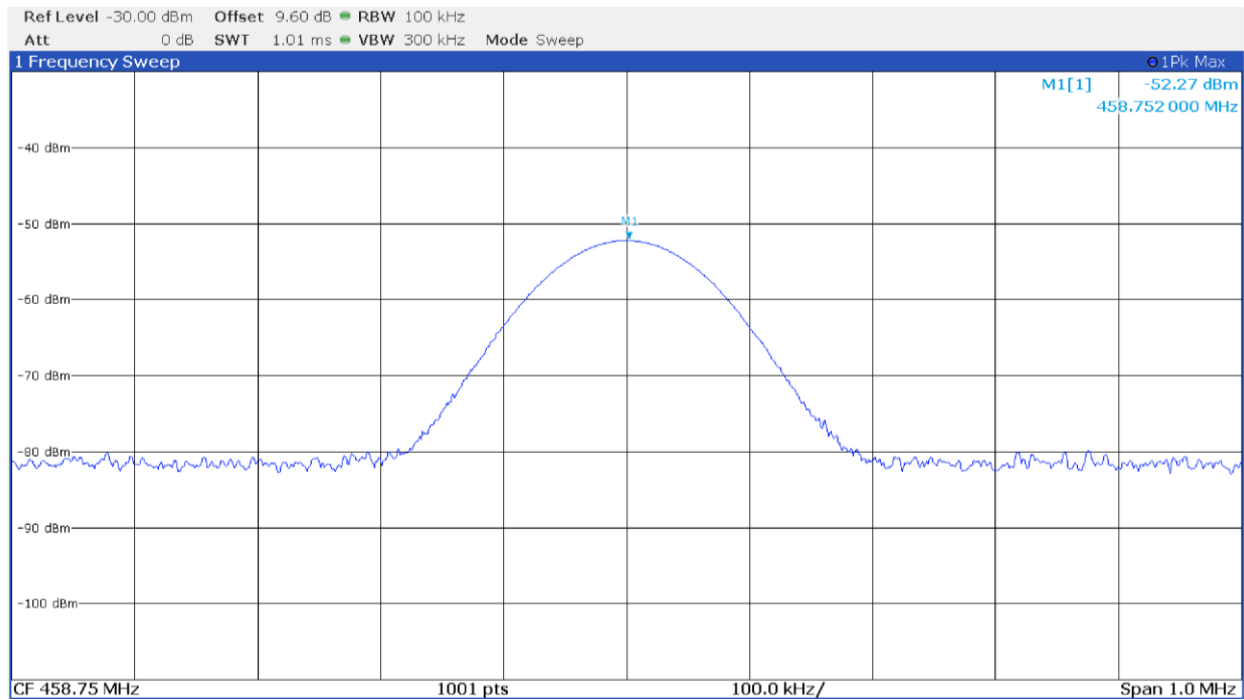
Figure 8.4-5: Input power with input signal at AGC threshold – up link
