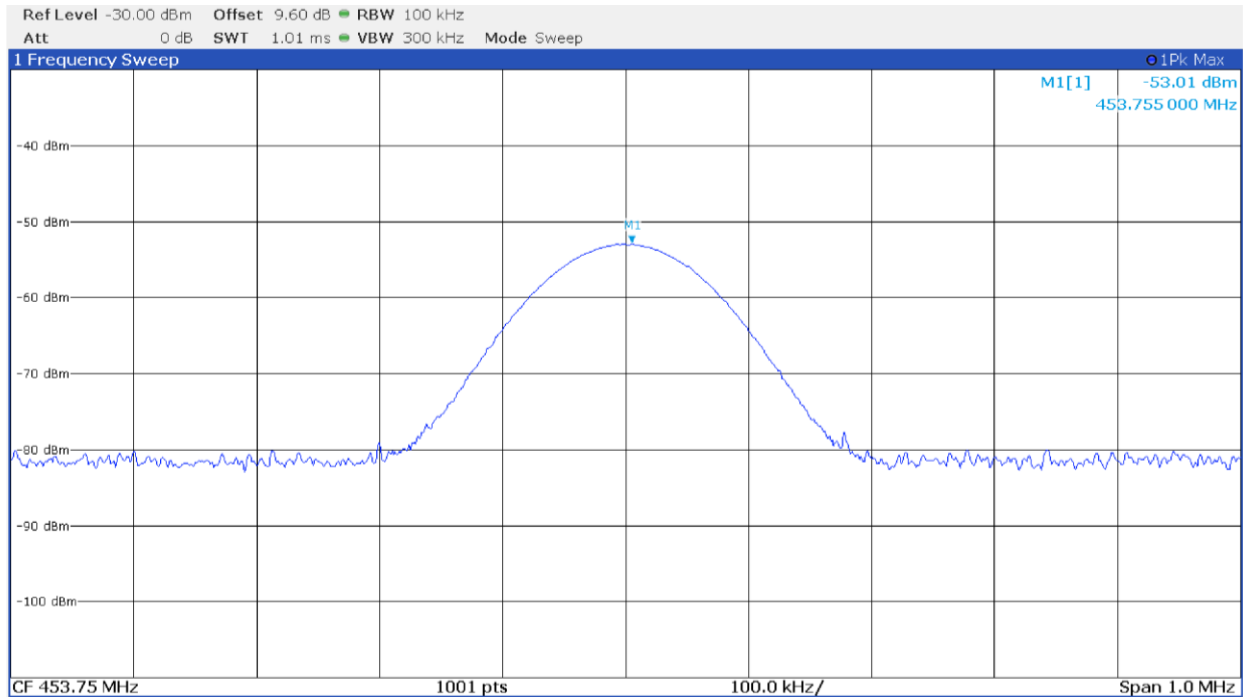
Figure 8.4-1: Input power with input signal at AGC threshold – down link
