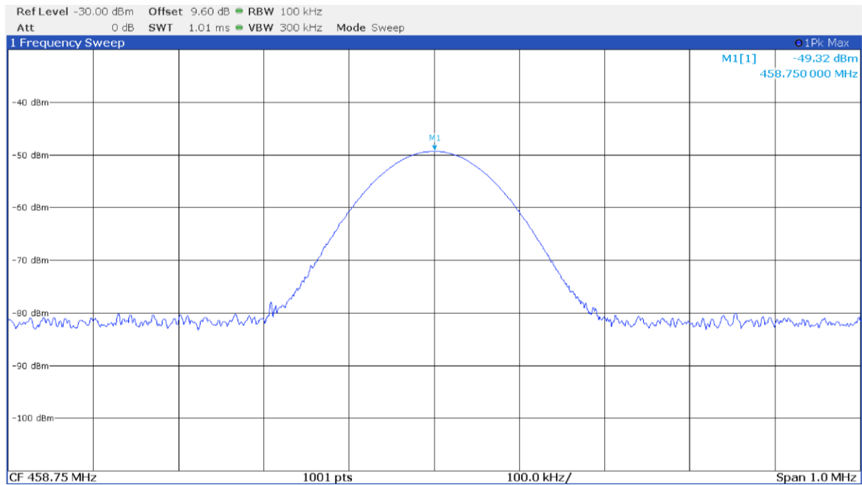
Figure 8.4-7: Input power with input signal at AGC threshold +3 dB – up link
