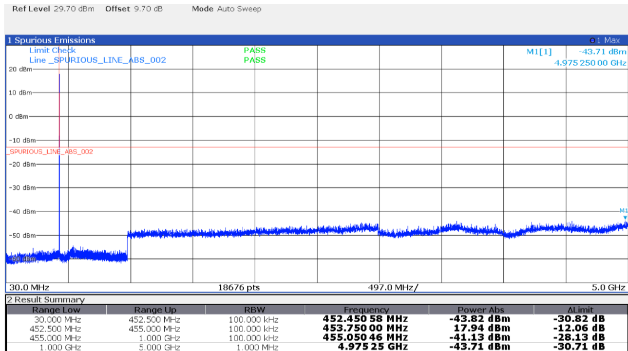
Figure 8.6-1: Conducted spurious emissions, down link
