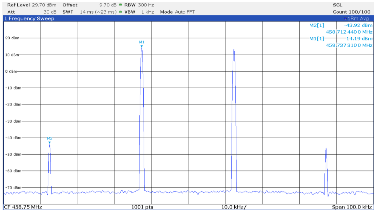
Figure 8.5-3: Up link intermodulation products with input signal at AGC threshold
