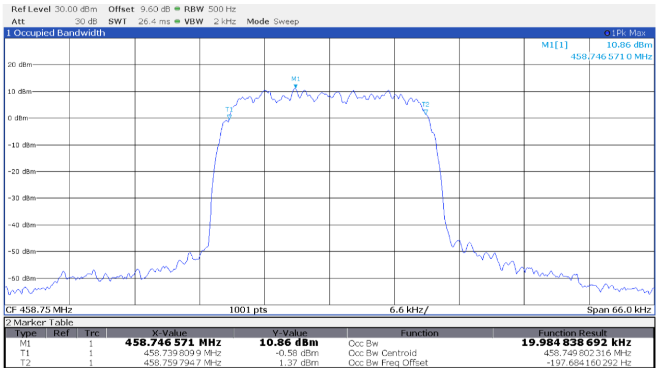
Figure 8.3-8: 99% occupied bandwidth, output signal at AGC threshold +3 dB spectral plot – up link
