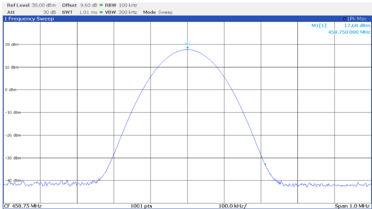
Figure 8.4-8: Output power with input signal at AGC threshold +3 dB – up link
