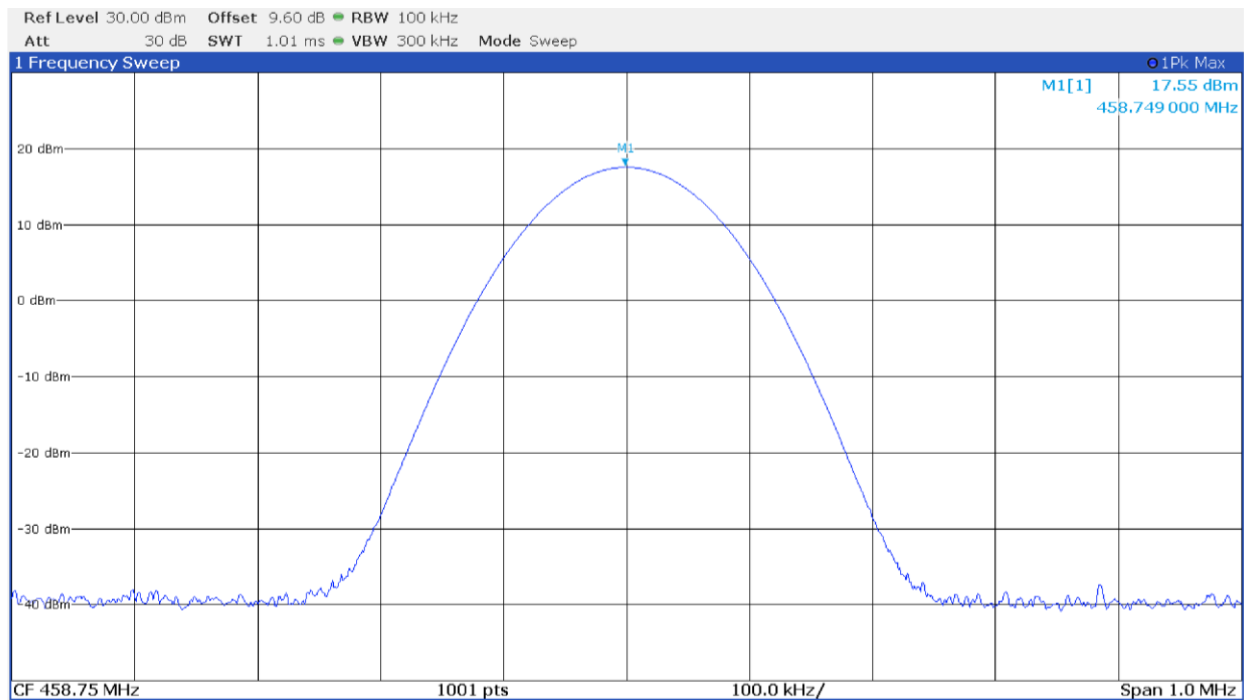
Figure 8.4-6: Output power with input signal at AGC threshold – up link
