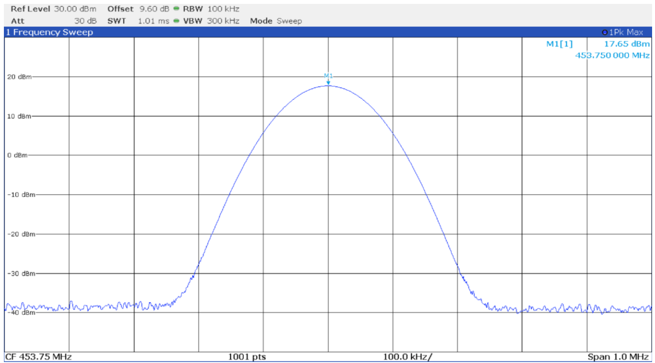
Figure 8.1-1: Down link - output spectral plot with input at AGC threshold – CW signal
