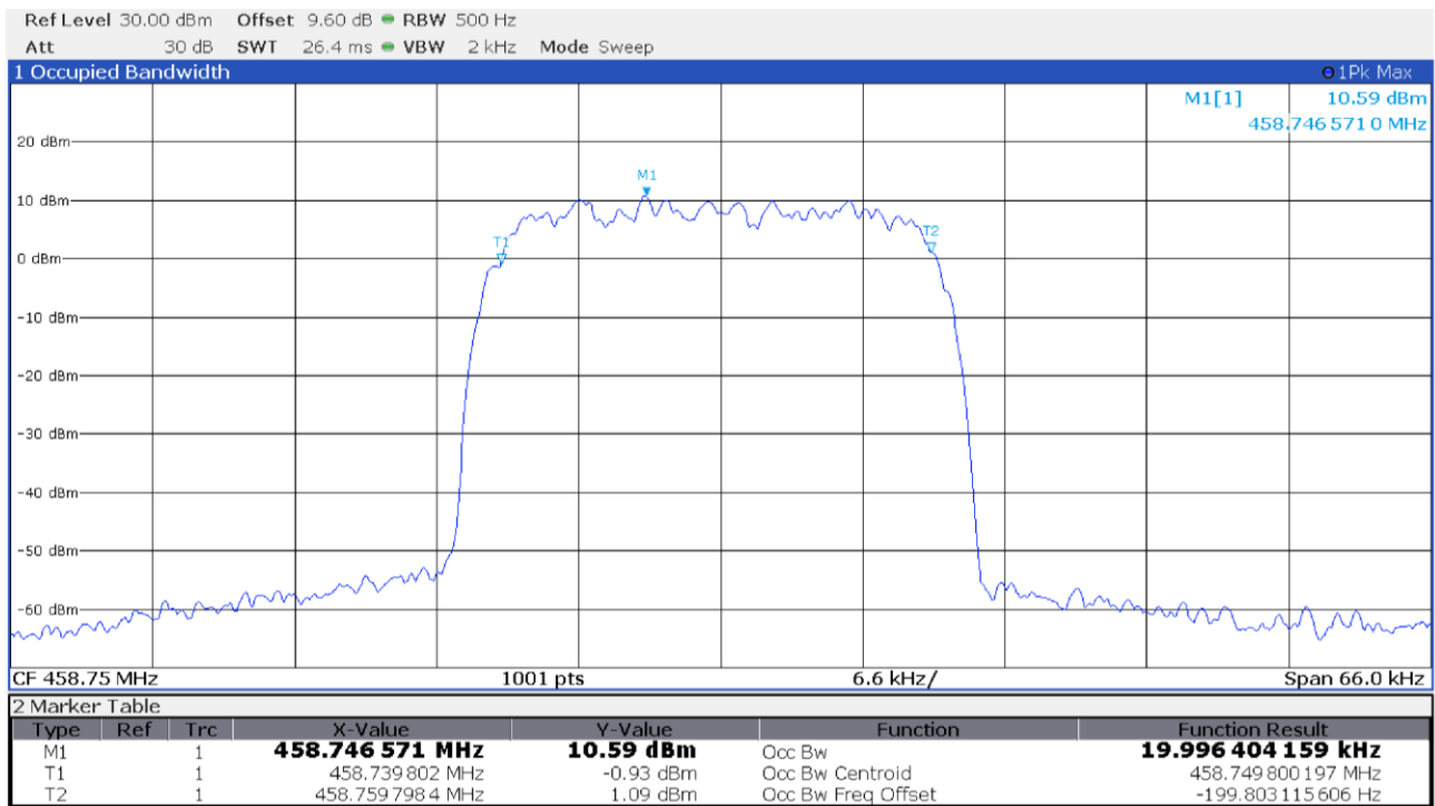
Figure 8.3-6: 99% occupied bandwidth, output signal at AGC threshold spectral plot – up link
