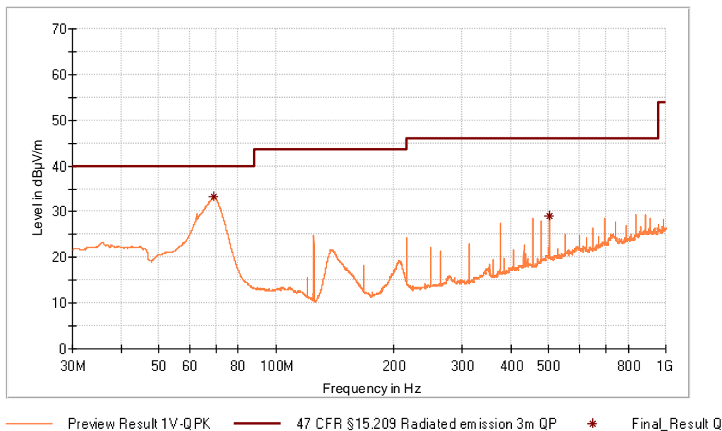
Figure 72: Chart of emissions test from 30 MHz to 1 GHz on middle channel (data rate ACL-E 2-DH1), EUT position Y, antenna polarization vertical
