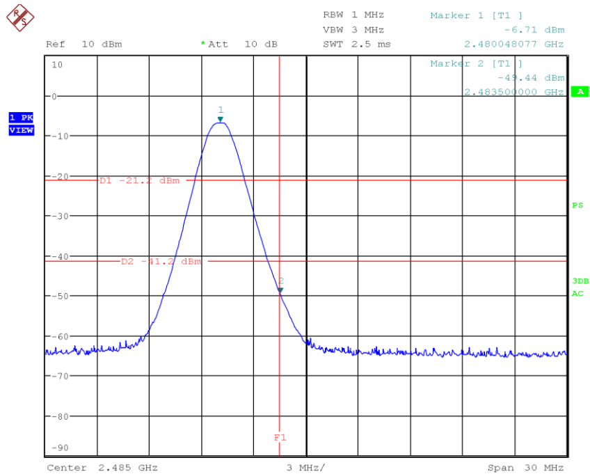
Figure 51: Chart of band-edge measurement on highest channel (PK) (data rate ACL-B DH5) – single mode
