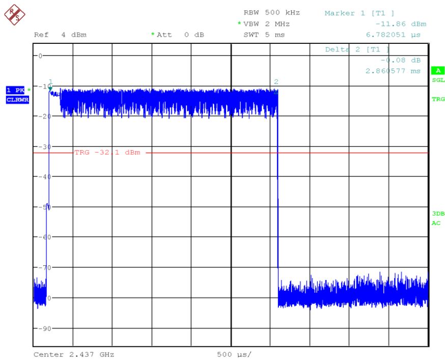
Figure 49: Burstlength (data rate ACL-E 3-DH5)
