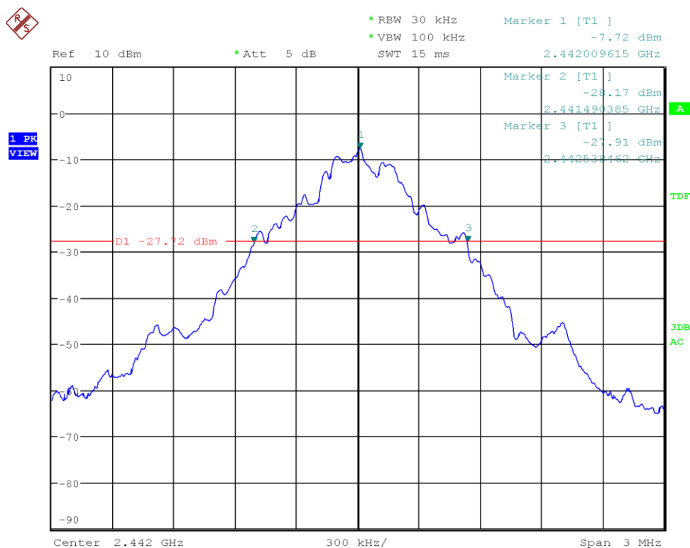
Figure 9: Chart of 20 dB bandwidth test on middle channel (data rate ACL-B DH1)
