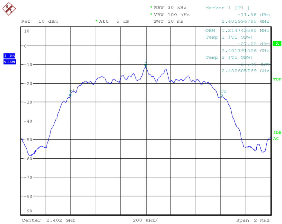
Figure 20: Chart of occupied bandwidth test on lowest channel (data rate ACL-E 2-DH3)
