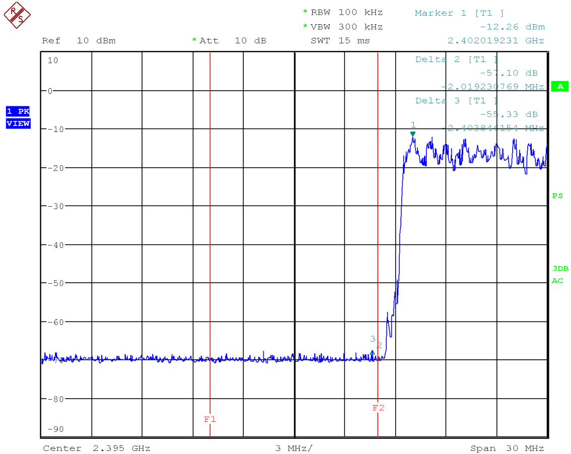
Figure 58: Chart of band-edge measurement on lowest channel (data rate ACL-E 2-DH1) – hopping mode
