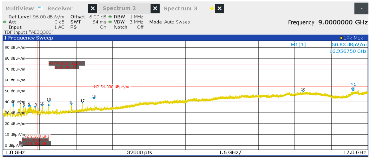
Figure 77: Chart of emissions test from 1 GHz to 17 GHz on highest channel (data rate ACL-E 2-DH1), EUT position X, antenna polarization vertical
