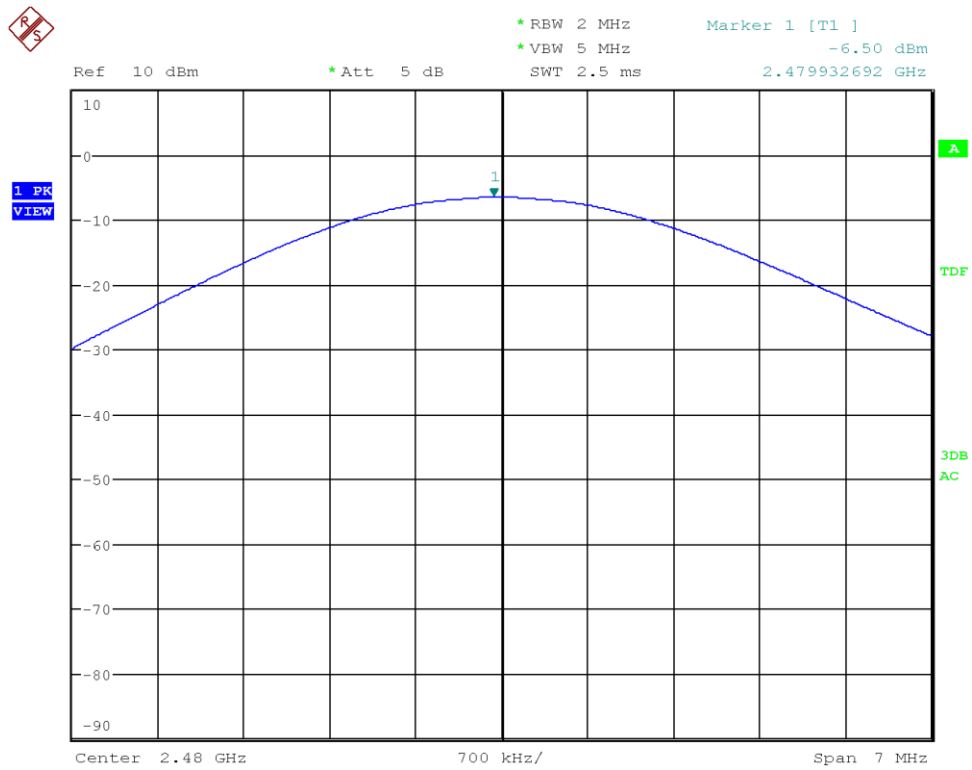
Figure 28: Chart of conducted output power on highest channel (data rate ACL-B DH1)
