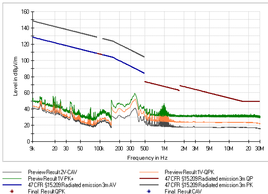
Figure 71: Chart of emissions test below 30 MHz on lowest channel (data rate ACL-E 2-DH1), EUT position X, antenna in line to the EUT
