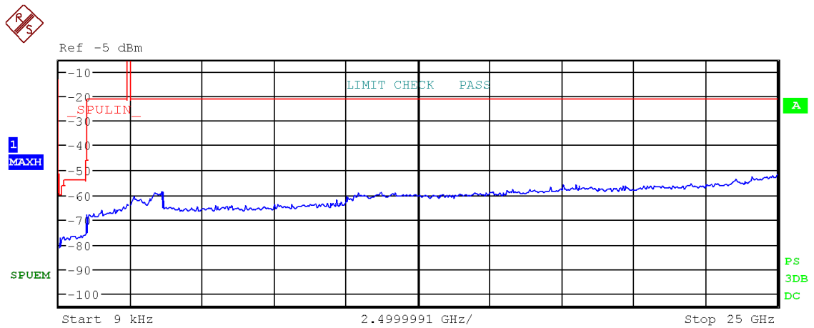
Figure 70: Chart of emissions test from 9 kHz to 25 GHz on highest channel (data rate ACL-E 3-DH1), PK-detector
