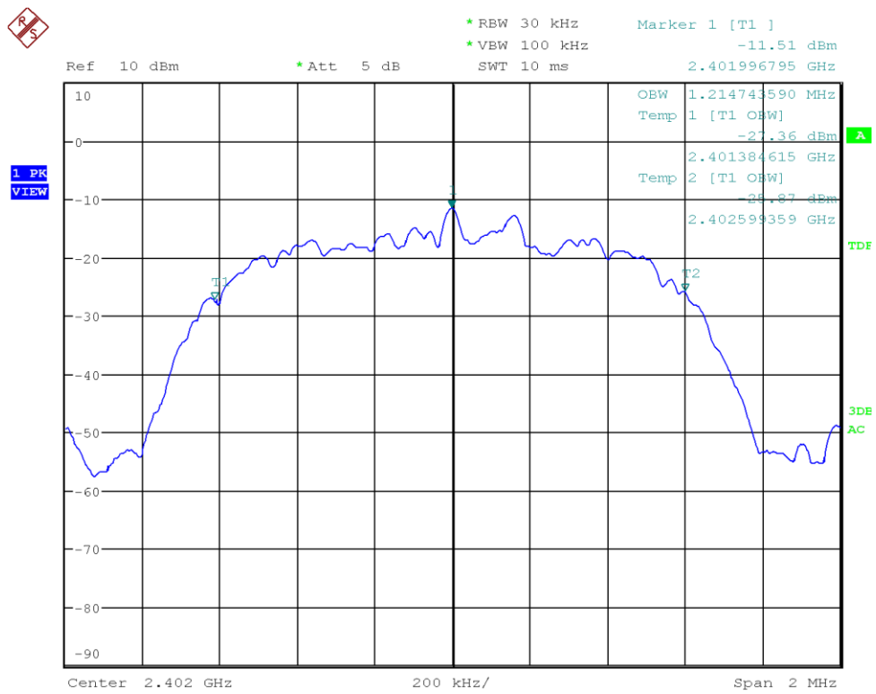
Figure 23: Chart of occupied bandwidth test on lowest channel (data rate ACL-E 3-DH3)
