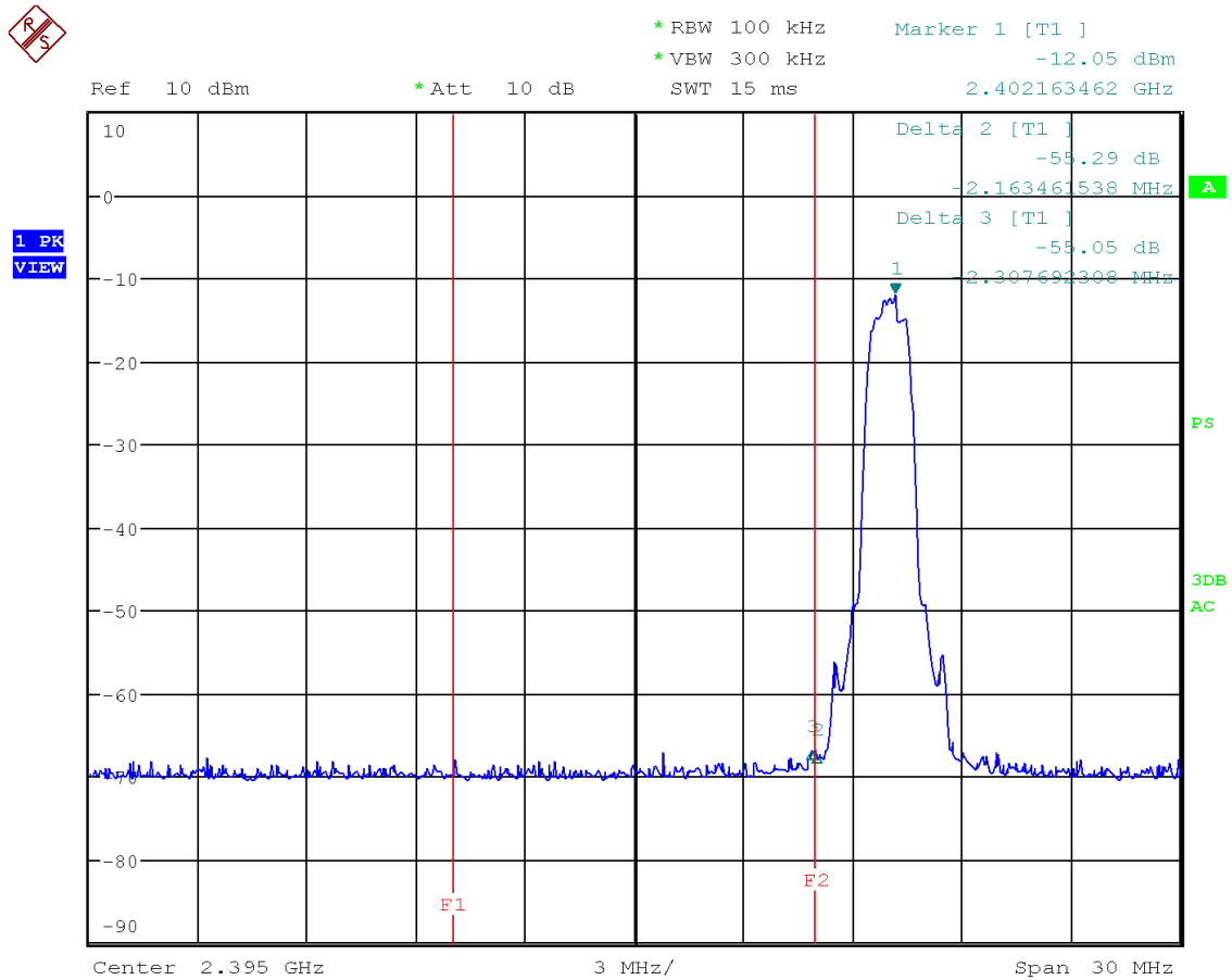
Figure 54: Chart of band-edge measurement on lowest channel (data rate ACL-E 3-DH3) – single mode
