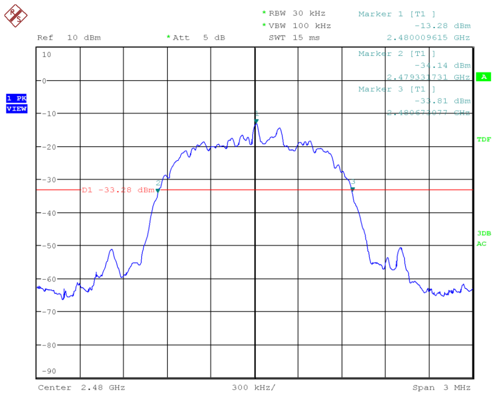
Figure 16: Chart of 20 dB bandwidth test on highest channel (data rate ACL-E 3-DH3)
