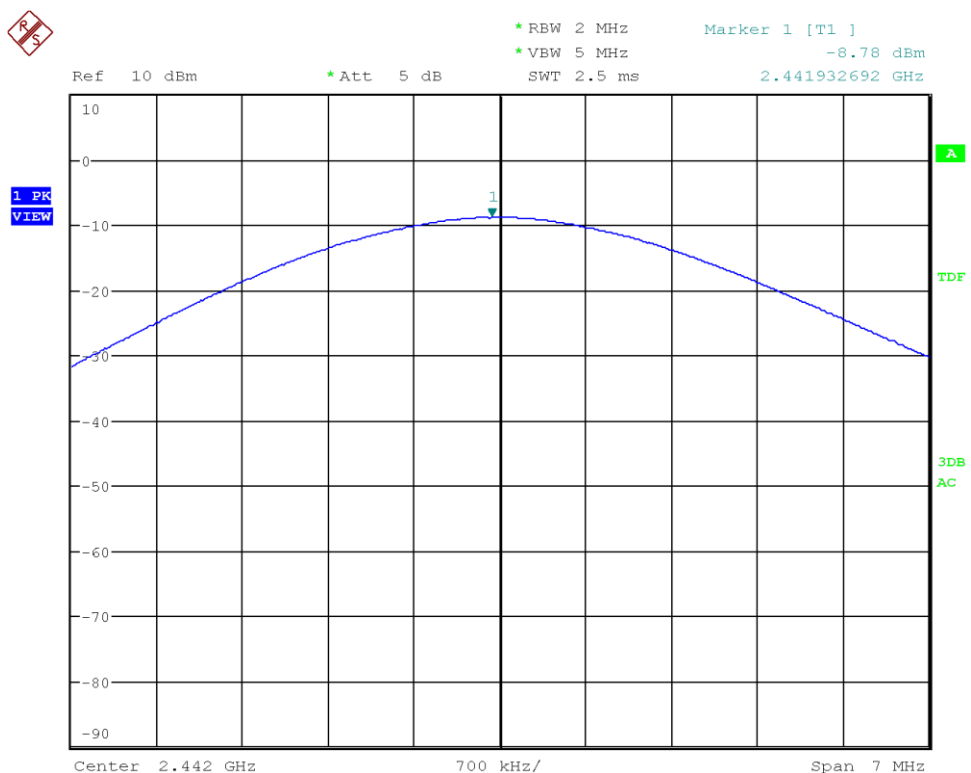
Figure 33: Chart of conducted output power on middle channel (data rate ACL-E 3-DH1)
