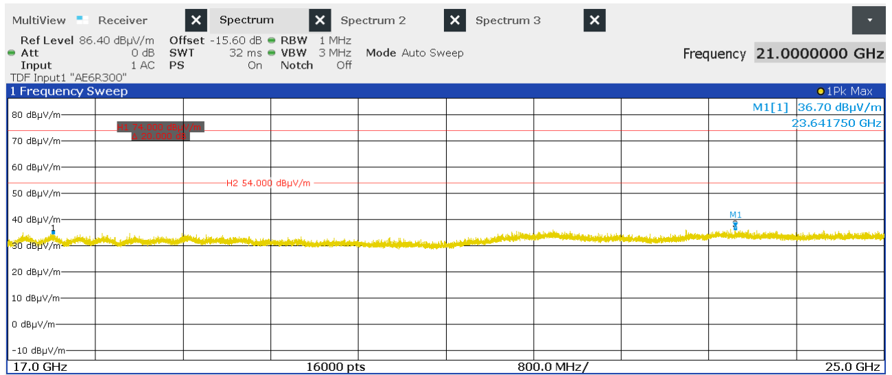
Figure 74: Chart of exploratory emission test from 17 GHz to 25 GHz on lowest channel (data rate ACL-E 2-DH1) at 0.5 m
