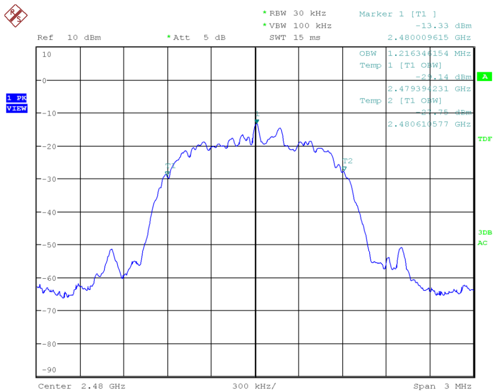
Figure 25: Chart of occupied bandwidth test on highest channel (data rate ACL-E 3-DH3)
