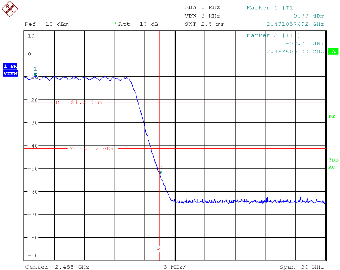
Figure 61: Chart of band-edge measurement on highest channel (PK) (data rate ACL-E 3-DH3) – hopping mode
