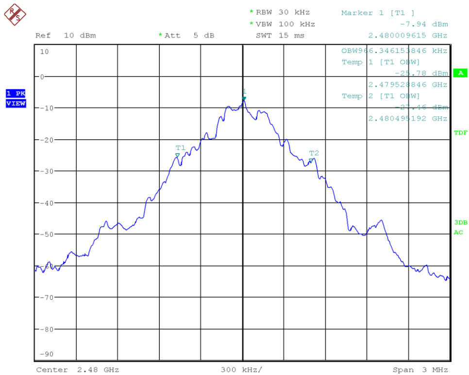
Figure 19: Chart of occupied bandwidth test on highest channel (data rate ACL-B DH1)
