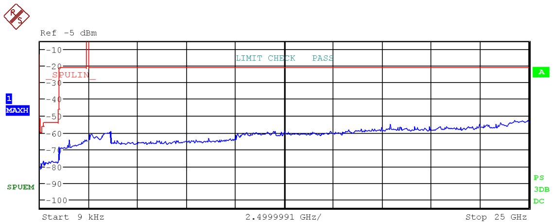
Figure 63: Chart of emissions test from 9 kHz to 25 GHz on middle channel (data rate ACL-B DH5), PK-detector
