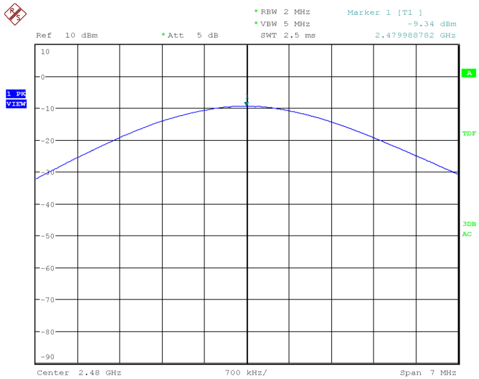
Figure 34: Chart of conducted output power on highest channel (data rate ACL-E 3-DH1)
