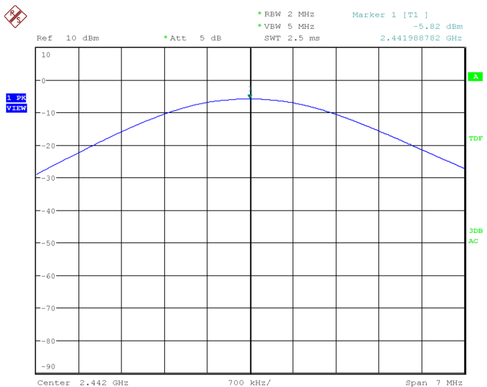
Figure 27: Chart of conducted output power on middle channel (data rate ACL-B DH1)
