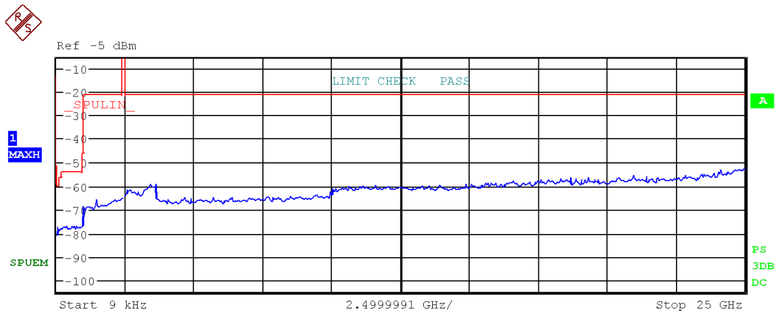
Figure 68: Chart of emissions test from 9 kHz to 25 GHz on lowest channel (data rate ACL-E 3-DH1), PK-detector
