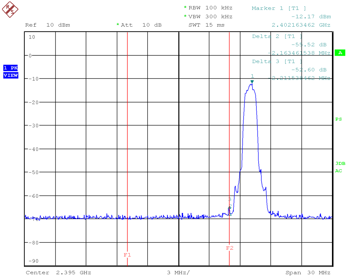
Figure 52: Chart of band-edge measurement on lowest channel (data rate ACL-E 2-DH3) – single mode
