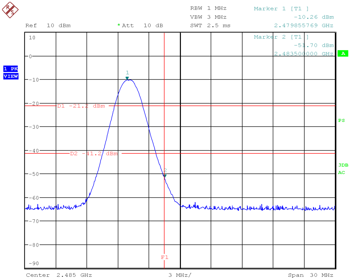
Figure 53: Chart of band-edge measurement on highest channel (PK) (data rate ACL-E 2-DH5) – single mode
