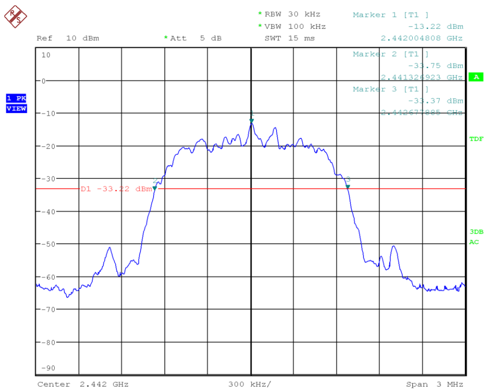
Figure 12: Chart of 20 dB bandwidth test on middle channel (data rate ACL-E 2-DH3)
