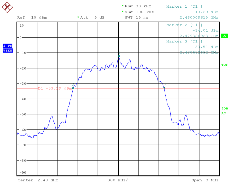
Figure 13: Chart of 20 dB bandwidth test on highest channel (data rate ACL-E 2-DH3)
