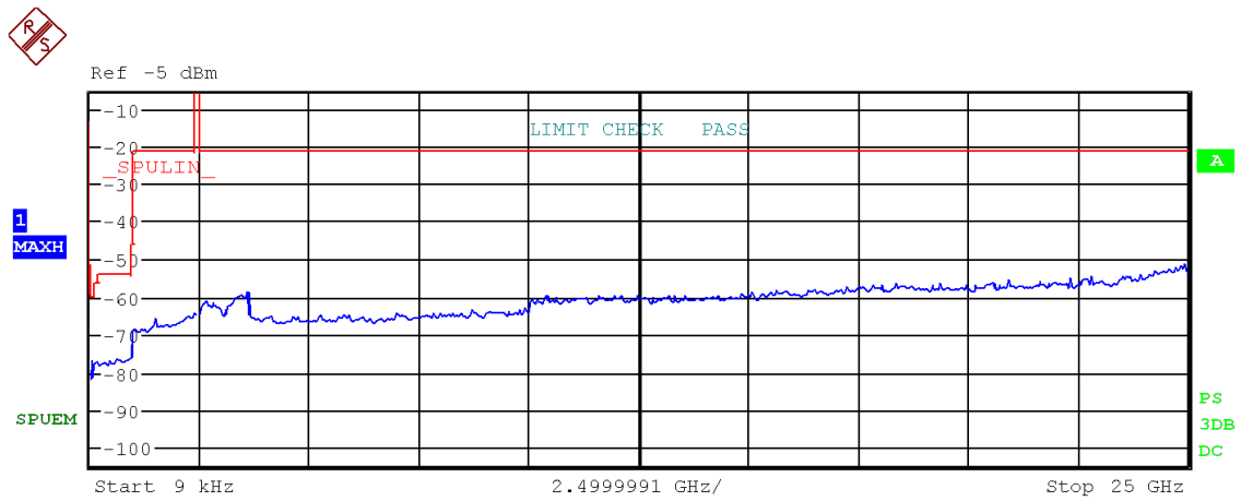
Figure 67: Chart of emissions test from 9 kHz to 25 GHz on highest channel (data rate ACL-E 2-DH1), PK-detector
