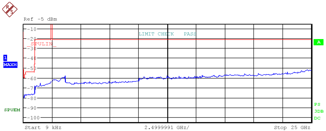
Figure 65: Chart of emissions test from 9 kHz to 25 GHz on lowest channel (data rate ACL-E 2-DH1), PK-detector
