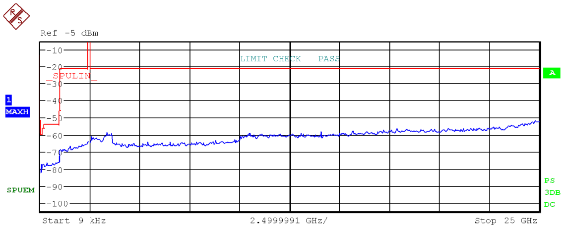
Figure 66: Chart of emissions test from 9 kHz to 25 GHz on middle channel (data rate ACL-E 2-DH1), PK-detector
