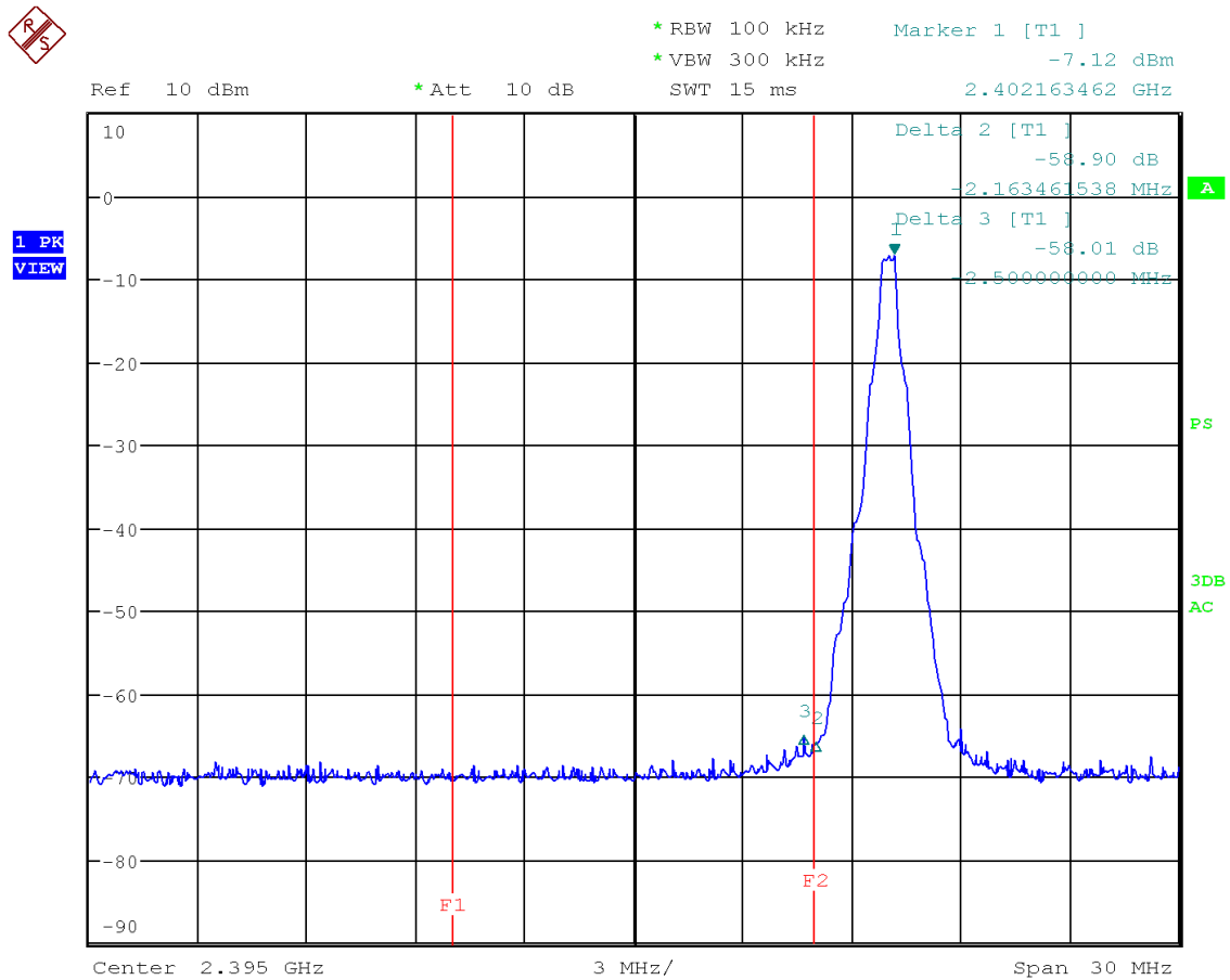
Figure 50: Chart of band-edge measurement on lowest channel (data rate ACL-B DH1) – single mode
