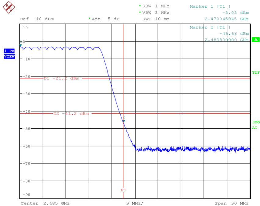
Figure 57: Chart of band-edge measurement on highest channel (PK) (data rate ACL-B DH5) – hopping mode
