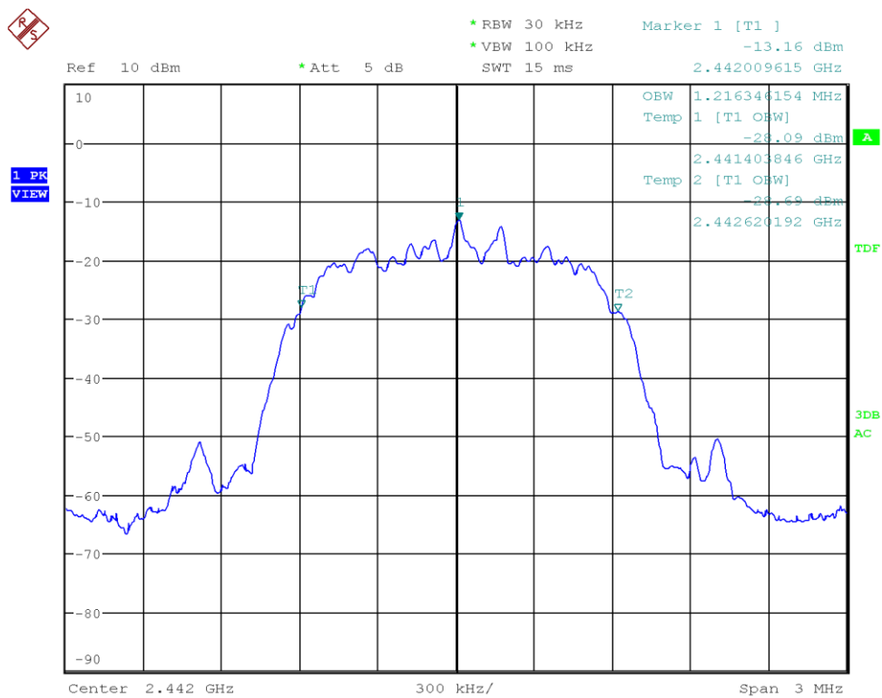
Figure 21: Chart of occupied bandwidth test on middle channel (data rate ACL-E 2-DH3)
