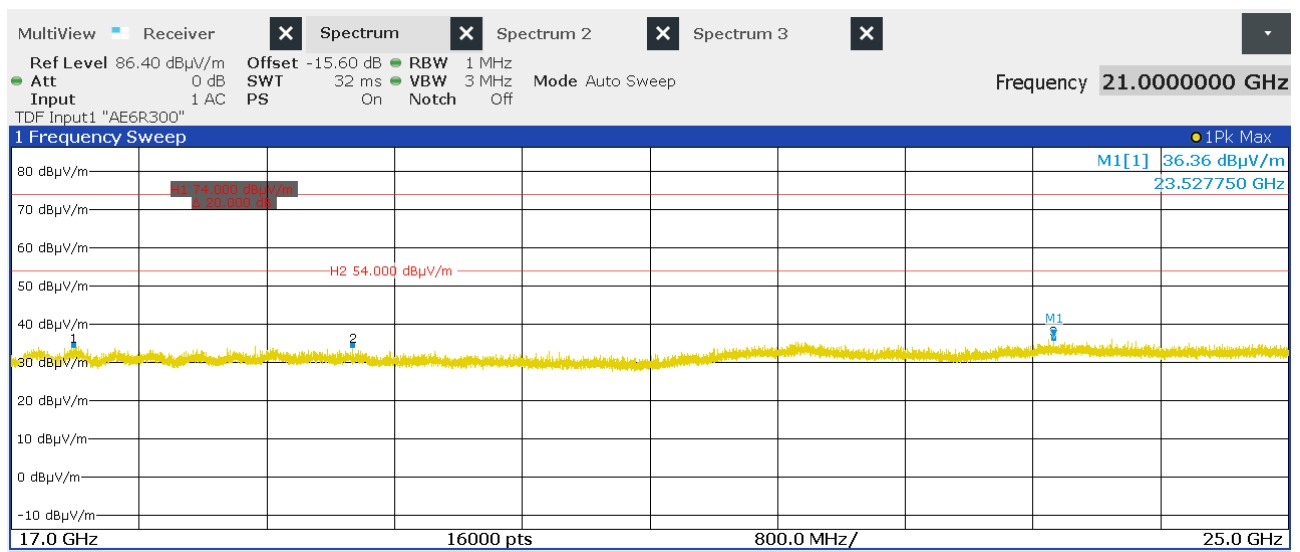
Figure 78: Chart of exploratory emission test from 17 GHz to 25 GHz on highest channel (data rate ACL-E 2-DH1) at 0.5 m
