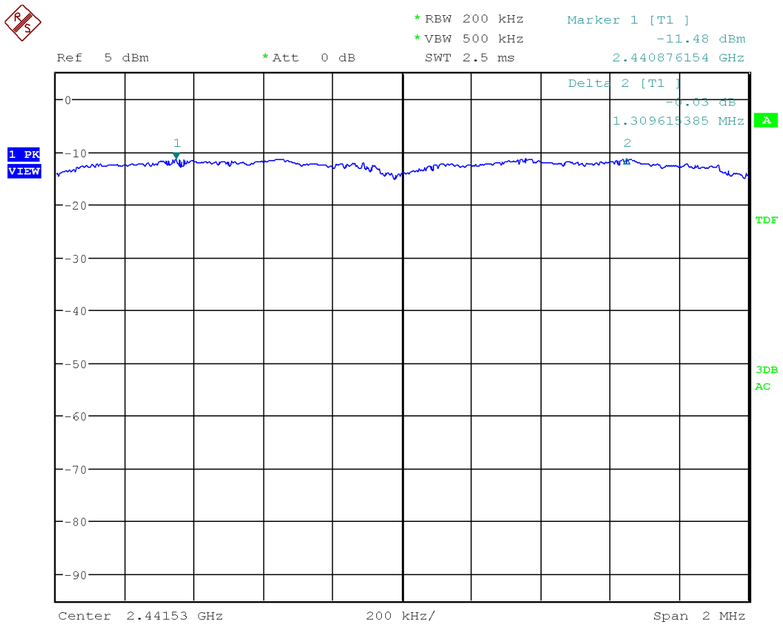
Figure 36: Chart of carrier frequency separation (data rate ACL-E 2-DH3)
