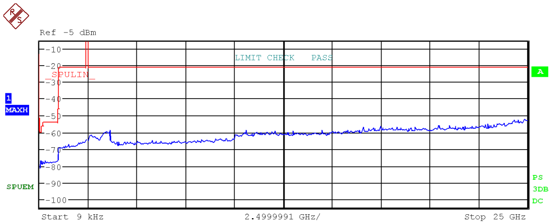
Figure 69: Chart of emissions test from 9 kHz to 25 GHz on middle channel (data rate ACL-E 3-DH1), PK-detector
