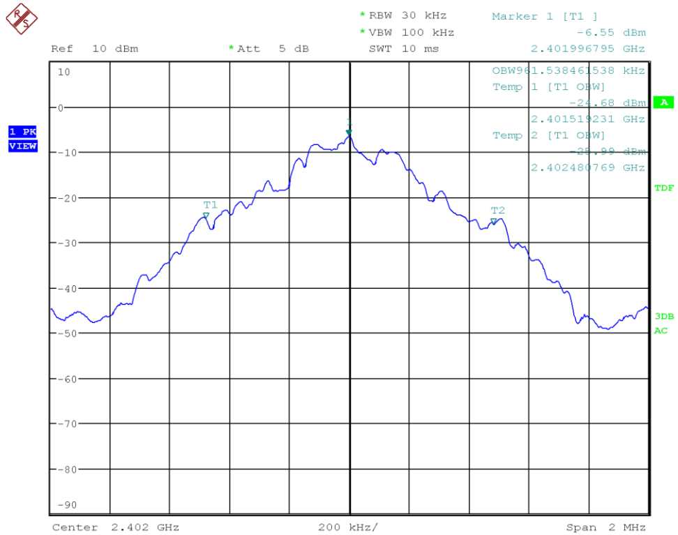
Figure 17: Chart of occupied bandwidth test on lowest channel (data rate ACL-B DH1)
