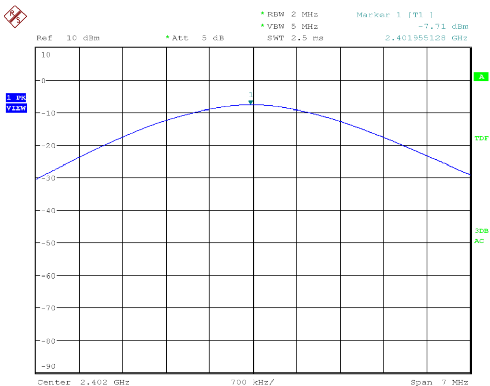
Figure 32: Chart of conducted output power on lowest channel (data rate ACL-E 3-DH1)
