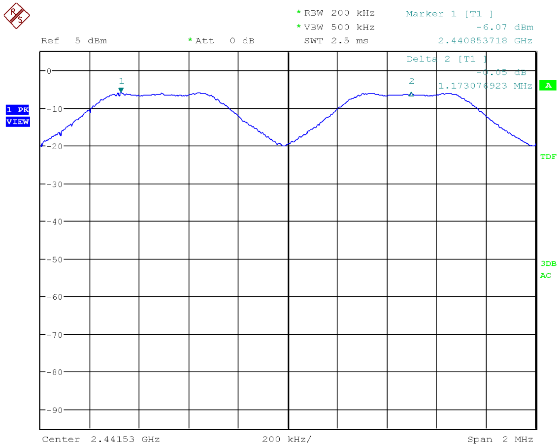
Figure 35: Chart of carrier frequency separation (data rate ACL-B DH3)
