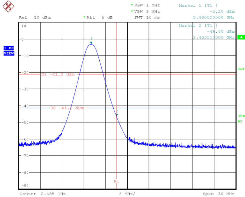
Figure 55: Chart of band-edge measurement on highest channel (PK) (data rate ACL-E 3-DH3) – single mode
