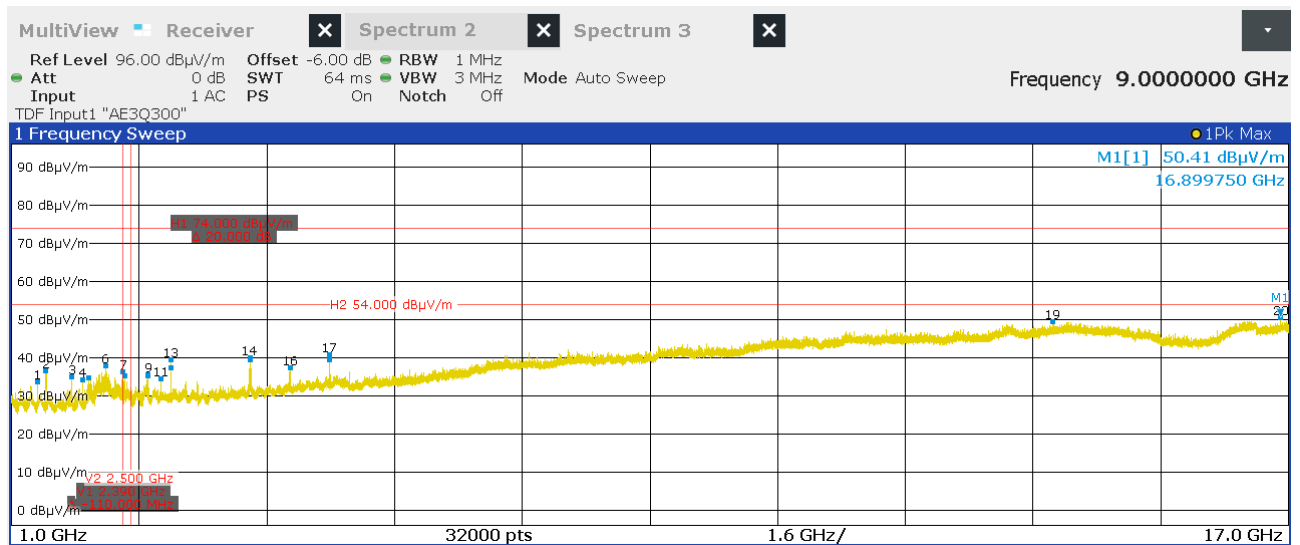
Figure 73: Chart of emissions test from 1 GHz to 17 GHz on lowest channel (data rate ACL-E 2-DH1), EUT position X, antenna polarization vertical
