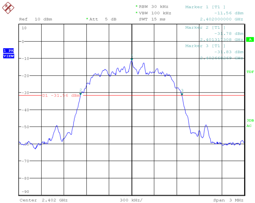
Figure 11: Chart of 20 dB bandwidth test on lowest channel (data rate ACL-E 2-DH3)
