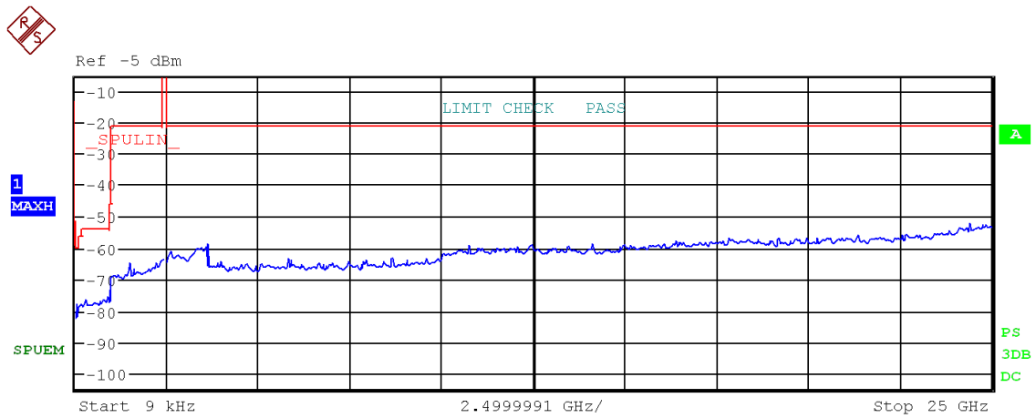
Figure 64: Chart of emissions test from 9 kHz to 25 GHz on highest channel (data rate ACL-B DH5), PK-detector
