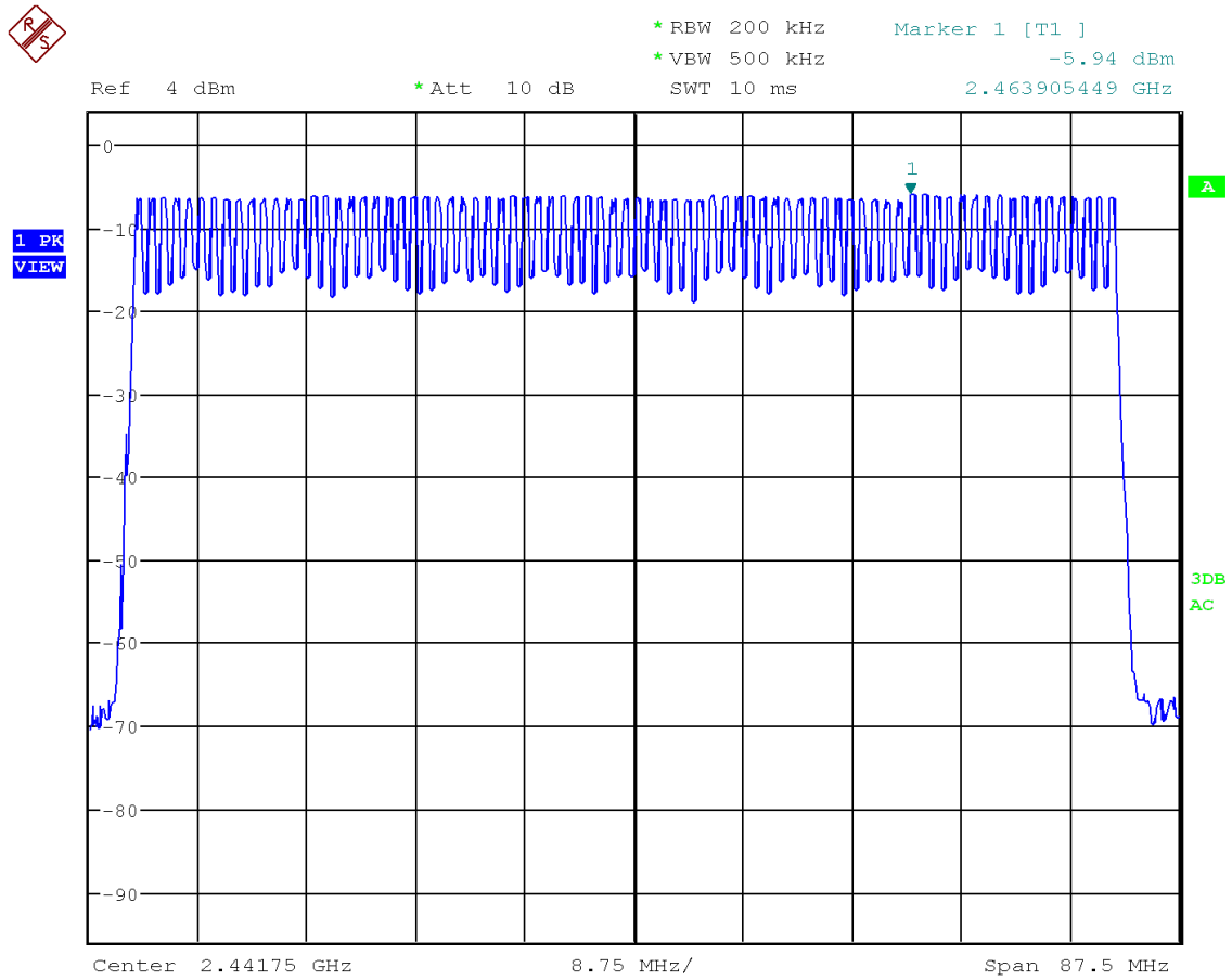
Figure 38: Chart of number of frequencies (data rate ACL-B DH1)
