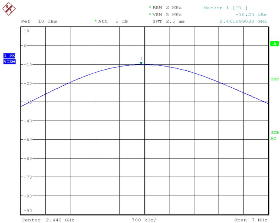
Figure 30: Chart of conducted output power on middle channel (data rate ACL-E 2-DH3)
