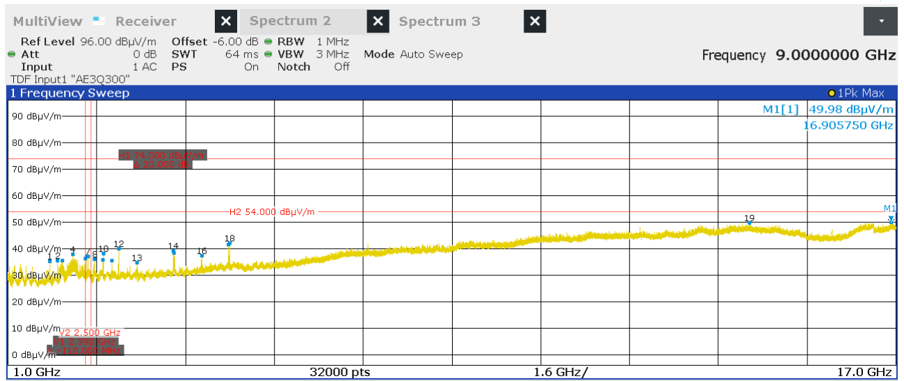
Figure 75: Chart of emissions test from 1 GHz to 17 GHz on middle channel (data rate ACL-E 2-DH1), EUT position X, antenna polarization vertical
