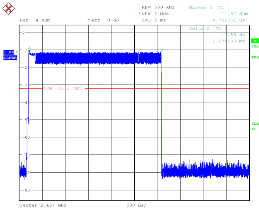
Figure 46: Burstlength (data rate ACL-E 2-DH5)
