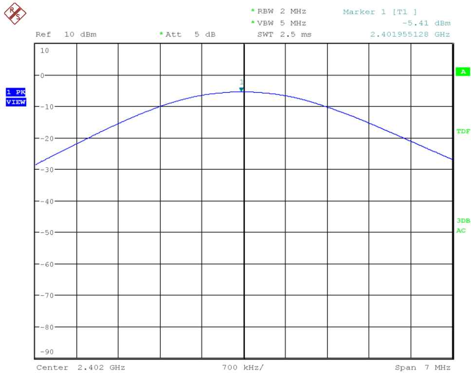
Figure 26: Chart of conducted output power on lowest channel (data rate ACL-B DH1)
