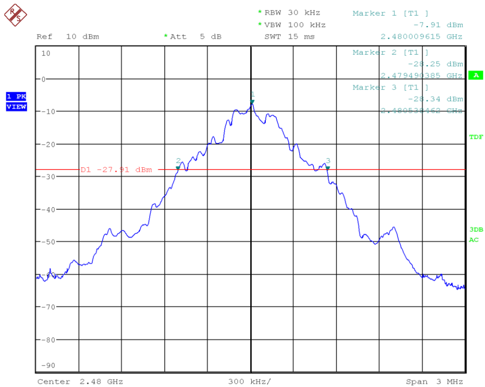
Figure 10: Chart of 20 dB bandwidth test on highest channel (data rate ACL-B DH1)
