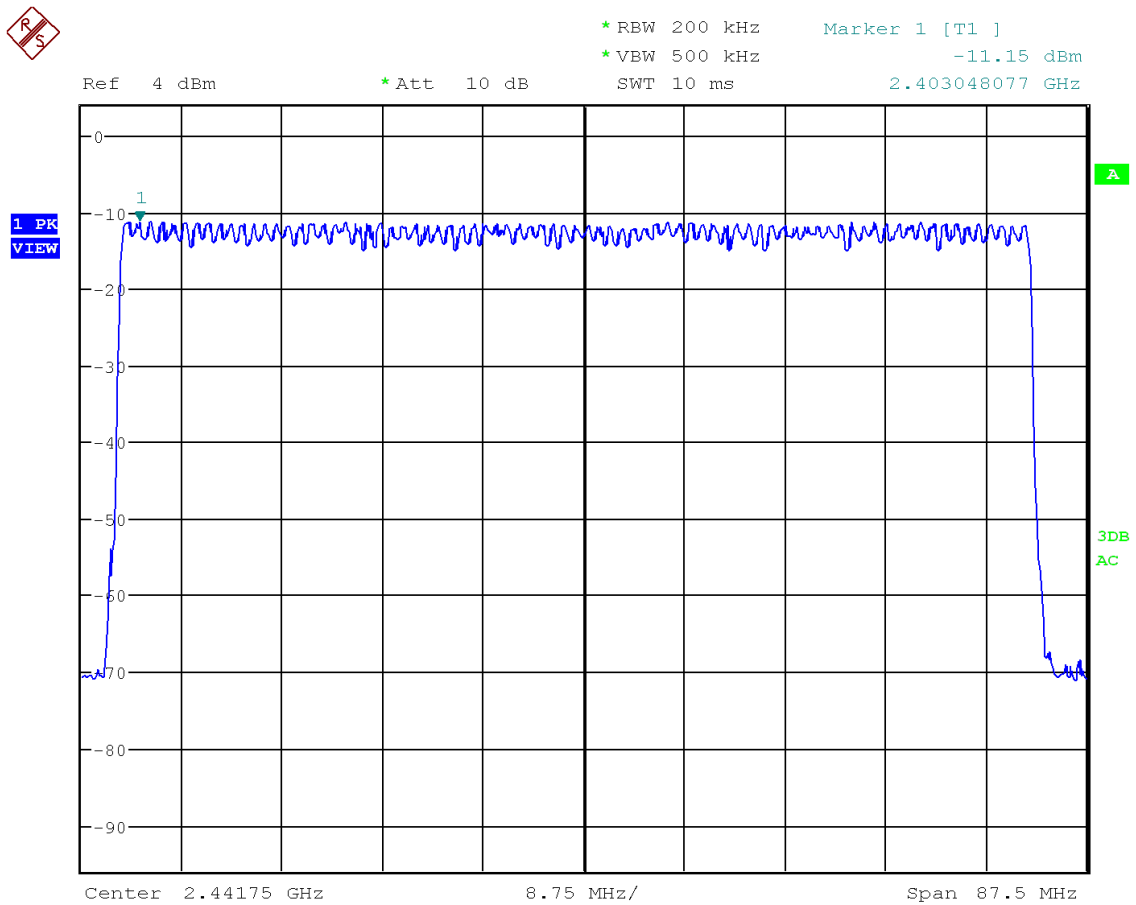
Figure 39: Chart of number of frequencies (data rate ACL-E 2-DH1)
