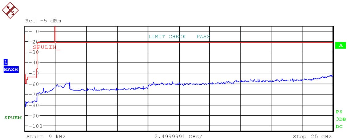
Figure 62: Chart of emissions test from 9 kHz to 25 GHz on lowest channel (data rate ACL-B DH5), PK-detector
