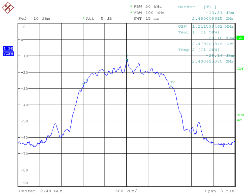
Figure 22: Chart of occupied bandwidth test on highest channel (data rate ACL-E 2-DH3)
