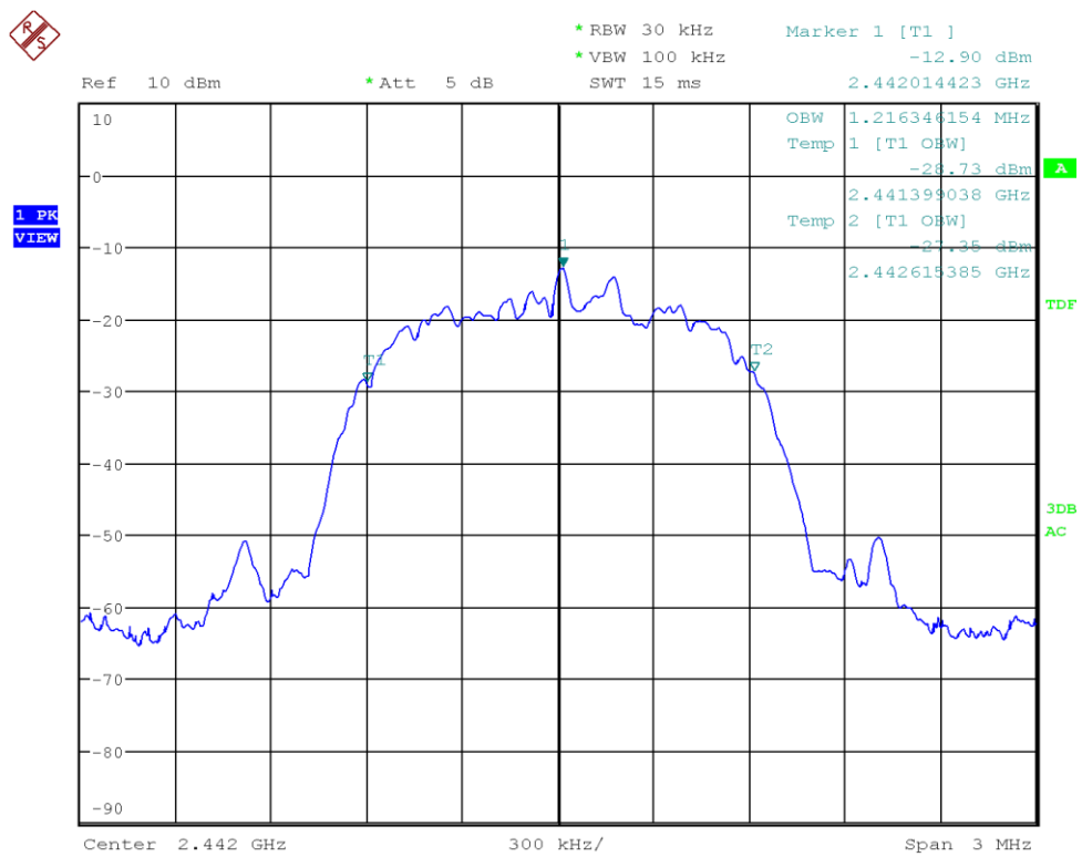
Figure 24: Chart of occupied bandwidth test on middle channel (data rate ACL-E 3-DH3)
