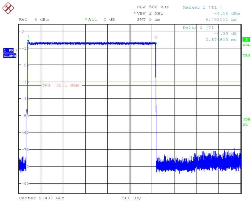
Figure 43: Burstlength (data rate ACL-B DH5)
