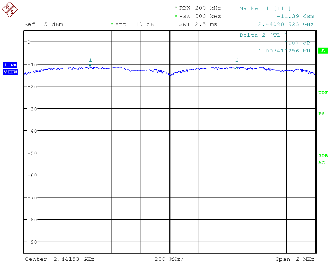
Figure 37: Chart of carrier frequency separation (data rate ACL-E 3-DH3)
