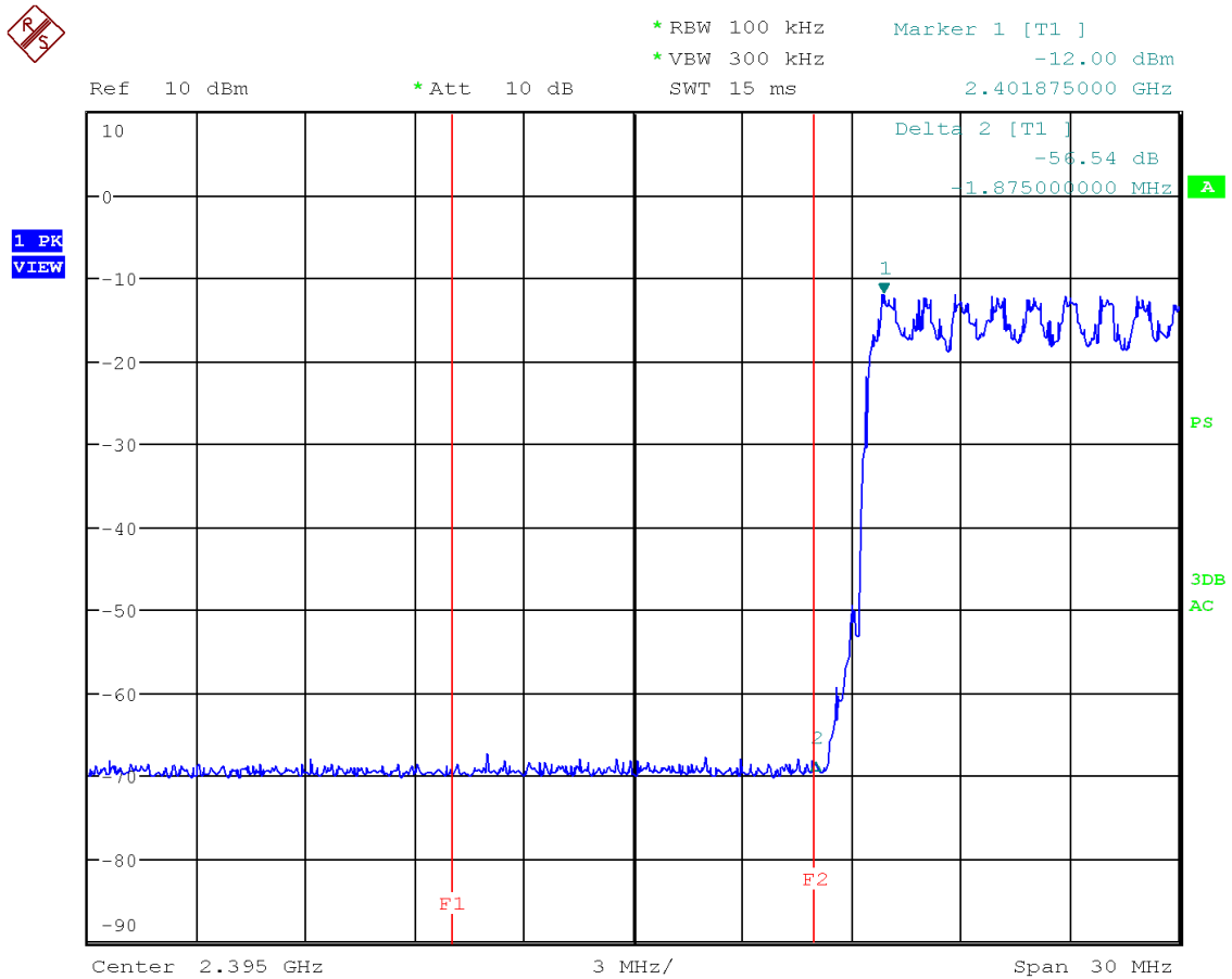
Figure 60: Chart of band-edge measurement on lowest channel (data rate ACL-E 3-DH1) – hopping mode
