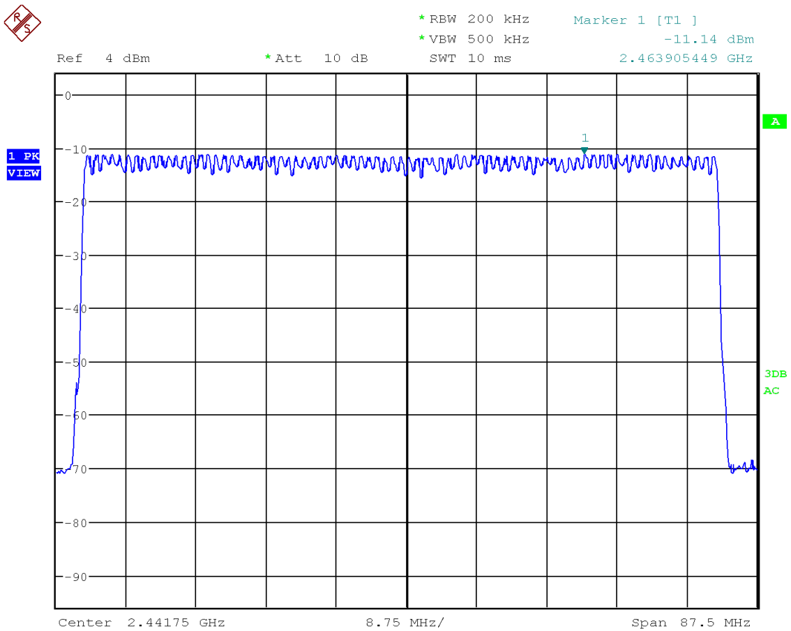
Figure 40: Chart of number of frequencies (data rate ACL-E 3-DH1)
