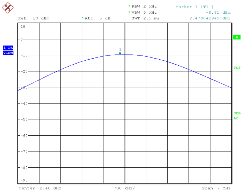
Figure 31: Chart of conducted output power on highest channel (data rate ACL-E 2-DH3)
