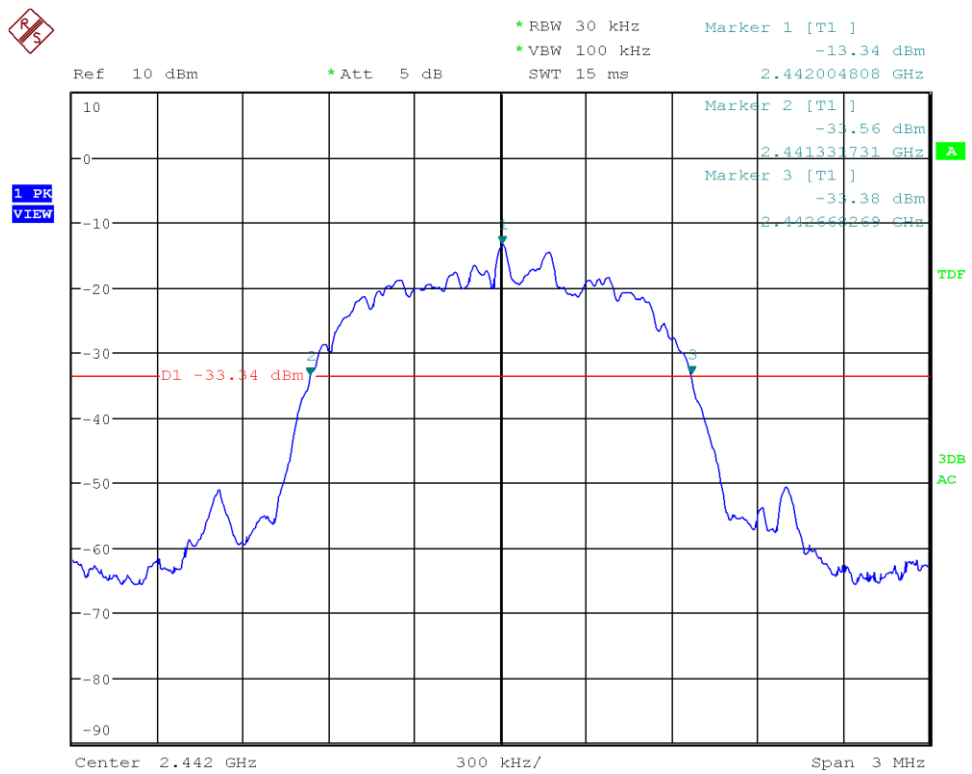
Figure 15: Chart of 20 dB bandwidth test on middle channel (data rate ACL-E 3-DH3)
