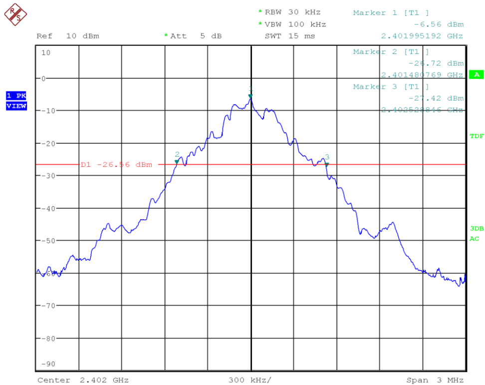
Figure 8: Chart of 20 dB bandwidth test on lowest channel (data rate ACL-B DH1)
