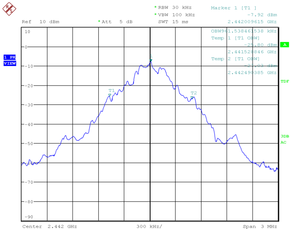
Figure 18: Chart of occupied bandwidth test on middle channel (data rate ACL-B DH1)
