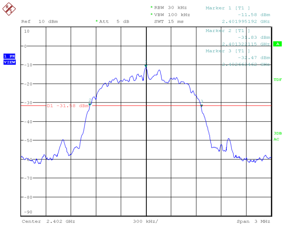
Figure 14: Chart of 20 dB bandwidth test on lowest channel (data rate ACL-E 3-DH3)
