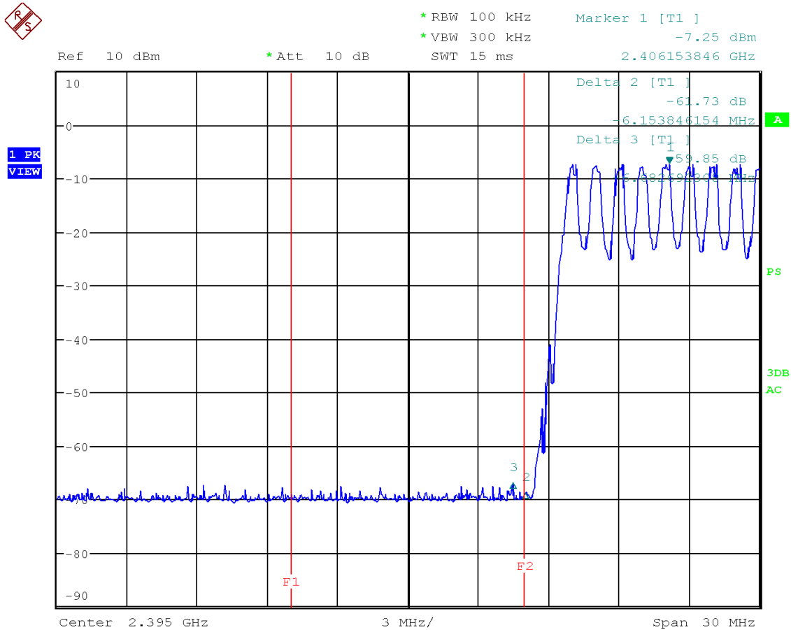
Figure 56: Chart of band-edge measurement on lowest channel (data rate ACL-B DH1) – hopping mode
