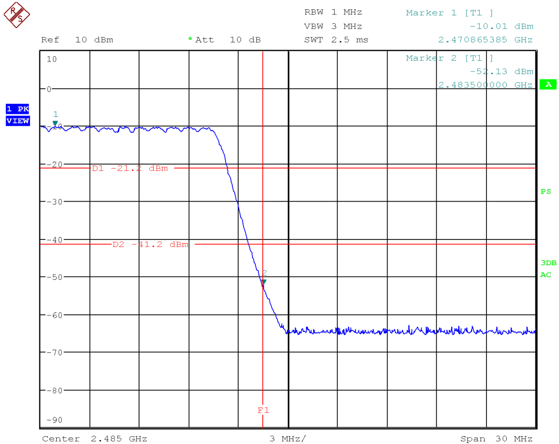
Figure 59: Chart of band-edge measurement on highest channel (PK) (data rate ACL-E 2-DH3) – hopping mode
